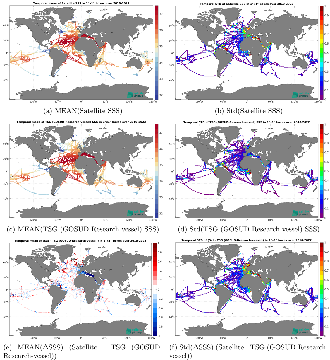
Figure 7: Temporal mean (left) and Std (right) of SSS from SMOS SSS L3 v335 - Monthly - 25 km (CATDS-CPDC) (top), TSG (GOSUD-Research-vessel) (middle), and of \Delta SSS (Satellite - TSG (GOSUD-Research-vessel)). Only match-up pairs are used to generate these maps.
