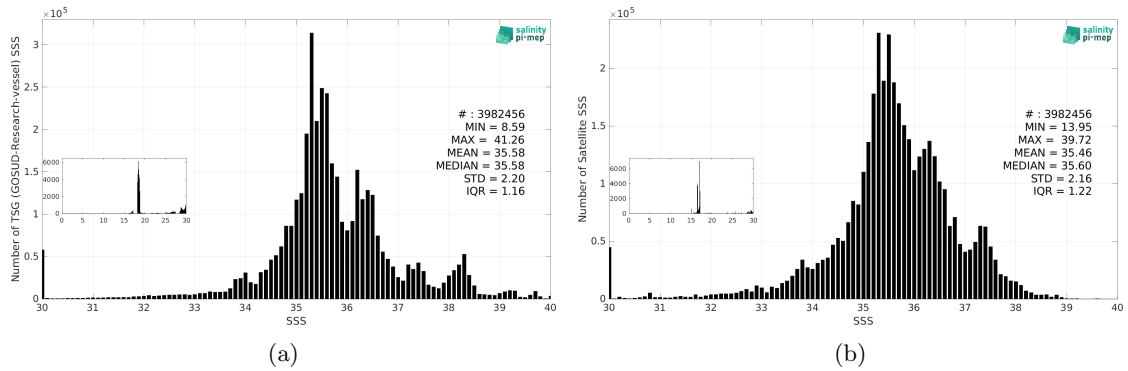
Figure 3: Histograms of SSS from TSG (GOSUD-Research-vessel) (a) and SMOS SSS L3 v335 - Monthly - 25 km (CATDS-CPDC) (b) considering all match-up pairs per bins of 0.1 over the Global Ocean Pi-MEP region and for the full satellite product period.
