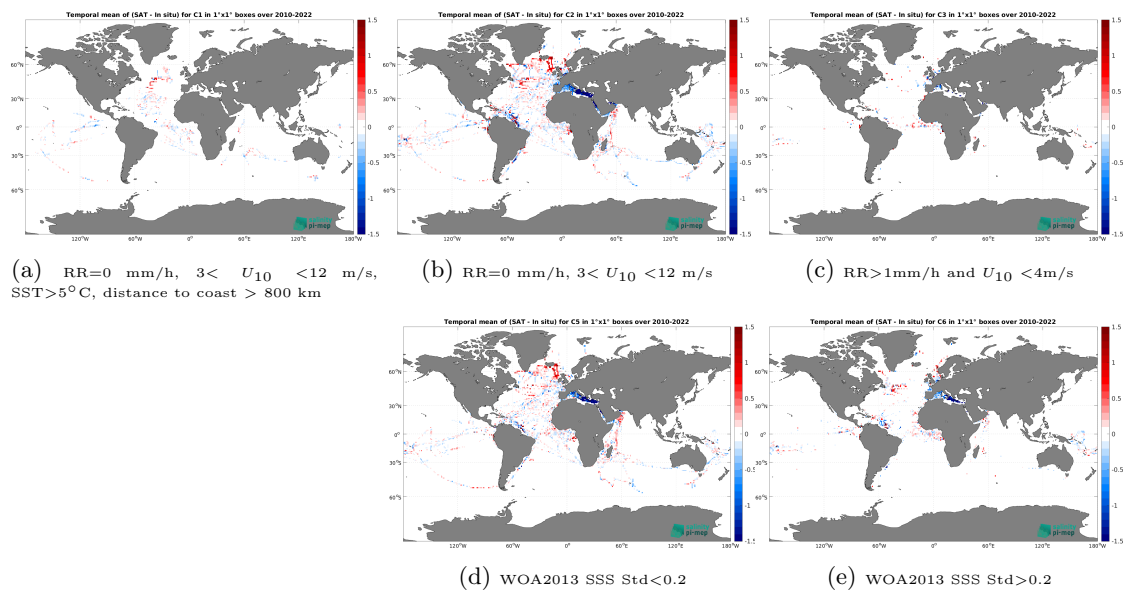
Figure 14: Temporal mean gridded over spatial boxes of size 1^\circ \times 1^\circ of \Delta\text{SSS} (SMOS SSS L3 v335 - Monthly - 25 km (CATDS-CPDC) - TSG (GOSUD-Research-vessel)) for 5 different subdatasets corresponding to:RR=0 mm/h, 3 < U_{10} < 12 m/s, SST > 5^\circ\text{C} , distance to coast > 800 km (a), RR=0 mm/h, 3 < U_{10} < 12 m/s (b), RR > 1 mm/h and U_{10} < 4 m/s (c), WOA2013 SSS Std < 0.2 (d), WOA2013 SSS Std > 0.2 (e).
