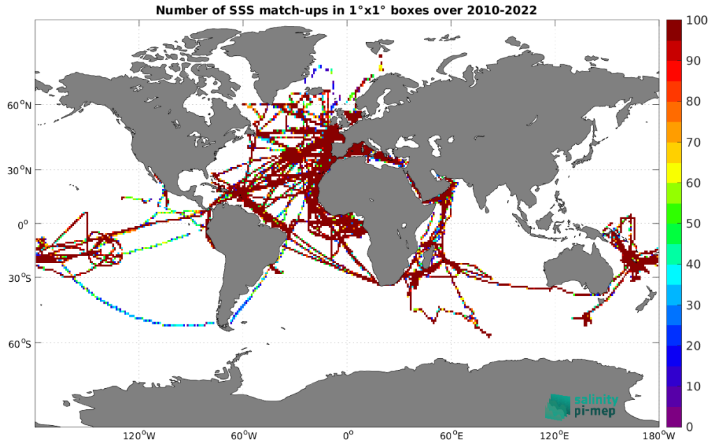
Figure 5: Number of SSS match-ups between TSG (GOSUD-Research-vessel) SSS and the SMOS SSS L3 v335 - Monthly - 25 km (CATDS-CPDC) SSS product for the Global Ocean Pi-MEP region over 1^\circ \times 1^\circ boxes and for the full satellite product period.
