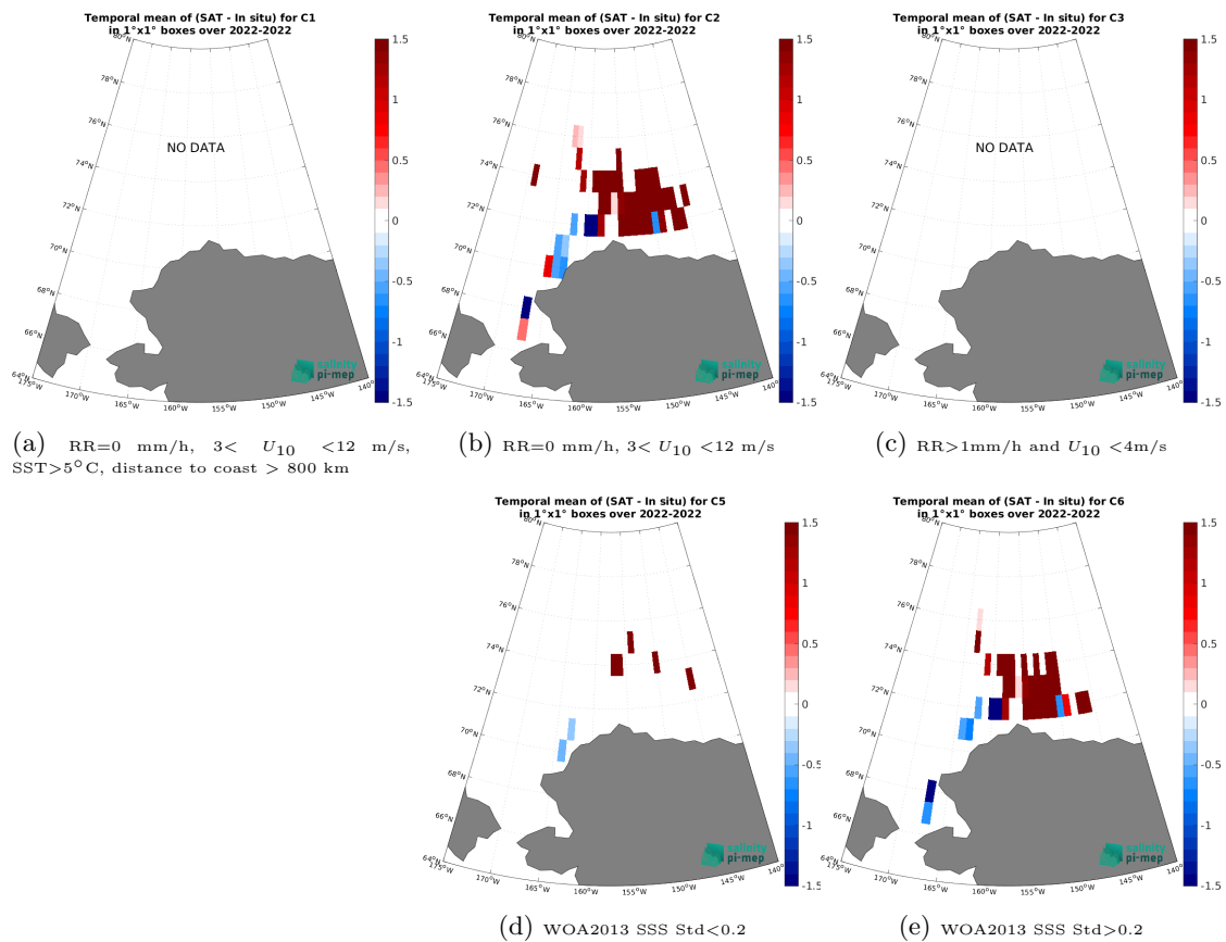
Figure 14: Temporal mean gridded over spatial boxes of size 1^\circ \times 1^\circ of \Delta\text{SSS} (SMOS SSS L3 v335 - Monthly - 25 km (CATDS-CPDC) - SASSIE) for 5 different subdatasets corresponding to:RR=0 mm/h, 3 < U_{10} < 12 m/s, SST>5°C, distance to coast > 800 km (a), RR=0 mm/h, 3 < U_{10} < 12 m/s (b), RR>1mm/h and U_{10} < 4 m/s (c), WOA2013 SSS Std<0.2 (d), WOA2013 SSS Std>0.2 (e).
