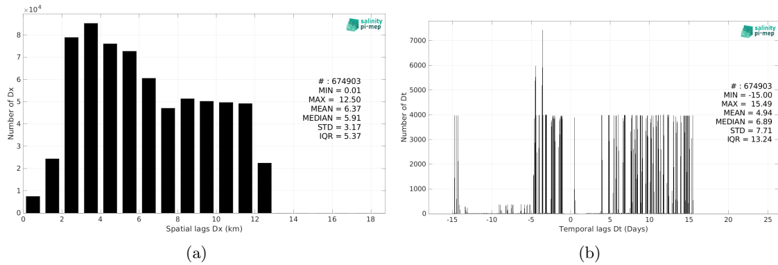
Figure 6: Histograms of the spatial (a) and temporal (b) lags between the location/time of the SASSIE measurement and the date of the corresponding SMOS SSS L3 v335 - Monthly - 25 km (CATDS-CPDC) SSS pixel.
