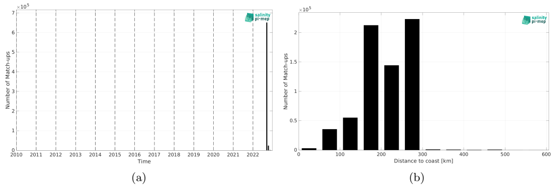
Figure 2: Number of match-ups between SASSIE and SMOS SSS L3 v335 - Monthly - 25 km (CATDS-CPDC) SSS as a function of time (a) and as function of the distance to coast (b) over the Global Ocean Pi-MEP region and for the full satellite product period.
