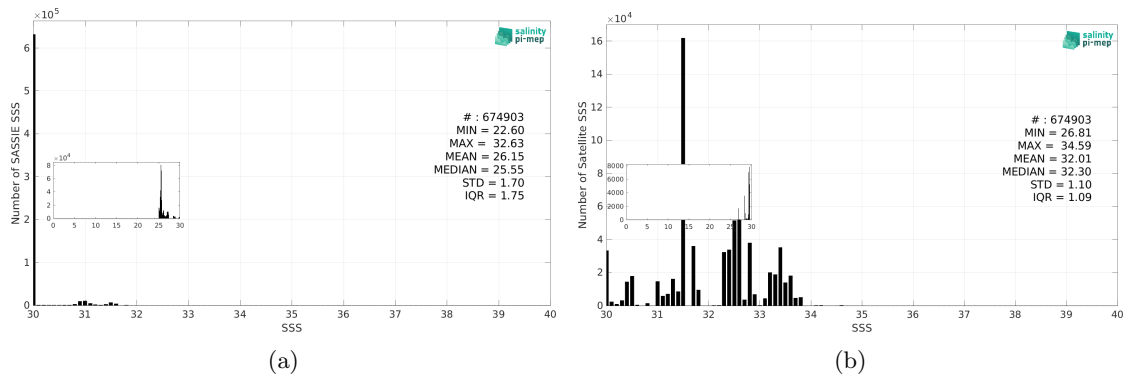
Figure 3: Histograms of SSS from SASSIE (a) and SMOS SSS L3 v335 - Monthly - 25 km (CATDS-CPDC) (b) considering all match-up pairs per bins of 0.1 over the Global Ocean Pi-MEP region and for the full satellite product period.
