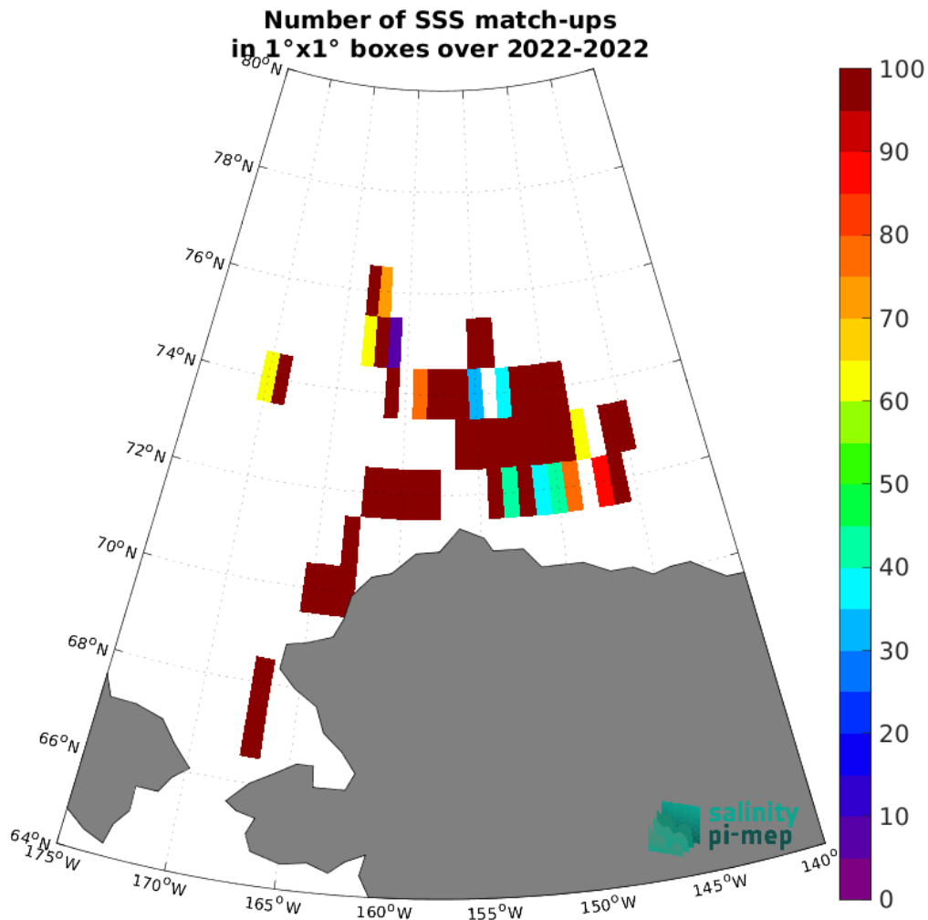
Figure 5: Number of SSS match-ups between SASSIE SSS and the SMOS SSS L3 v335 - Monthly - 25 km (CATDS-CPDC) SSS product for the Global Ocean Pi-MEP region over 1°x1° boxes and for the full satellite product period.
