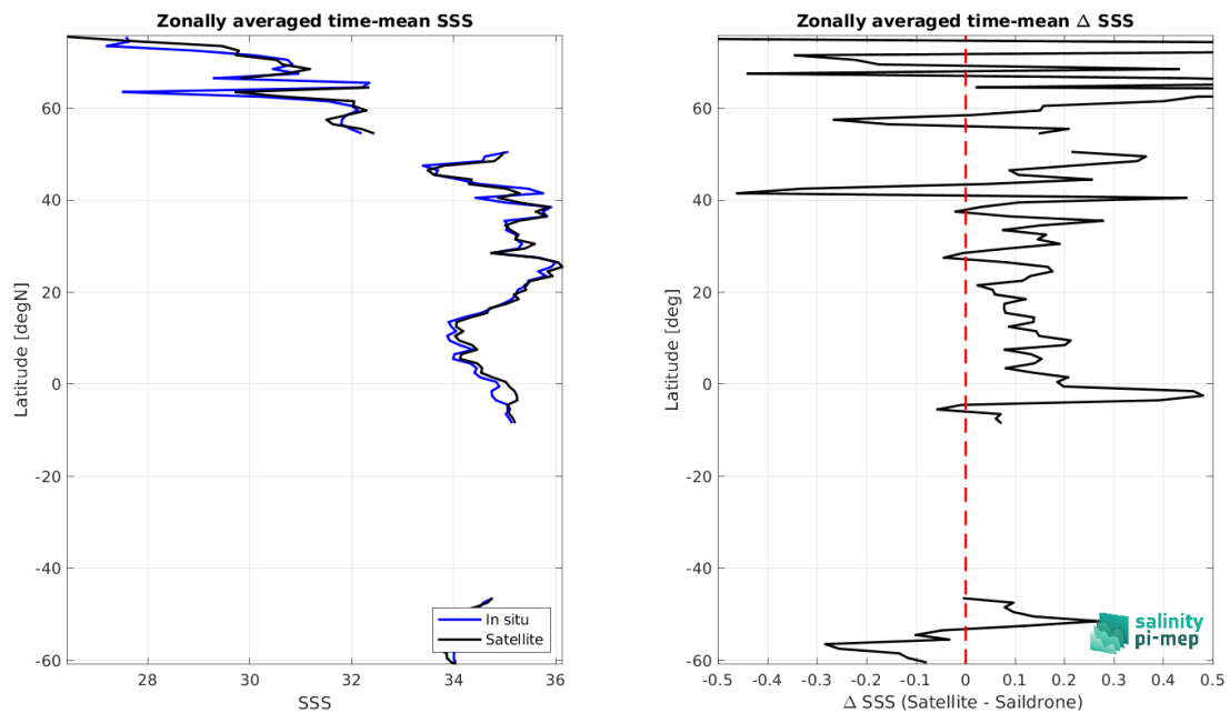
Figure 9: Left panel: Zonal mean SSS from SMOS SSS L3 v335 - Monthly - 25 km (CATDS-CPDC) satellite product (black) and from Sailldrone (blue). Right panel: Zonal mean of \Delta SSS (Satellite - Sailldrone) for all the collected Pi-MEP match-up pairs estimated over the full satellite product period.
