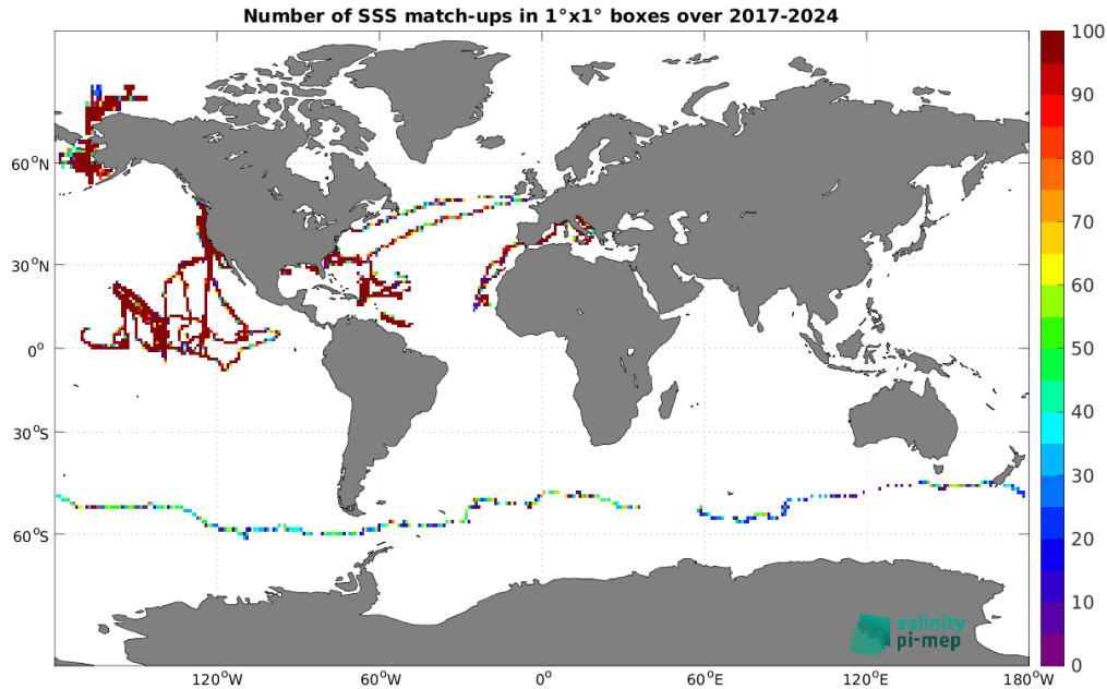
Figure 5: Number of SSS match-ups between Sairdrone SSS and the SMOS SSS L3 v335 - Monthly - 25 km (CATDS-CPDC) SSS product for the Global Ocean Pi-MEP region over 1^\circ \times 1^\circ boxes and for the full satellite product period.
