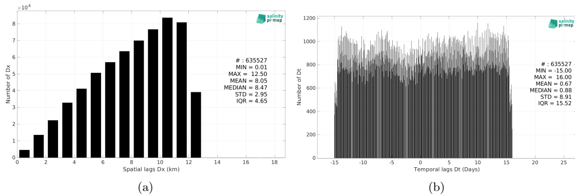
Figure 6: Histograms of the spatial (a) and temporal (b) lags between the location/time of the Sairdrone measurement and the date of the corresponding SMOS SSS L3 v335 - Monthly - 25 km (CATDS-CPDC) SSS pixel.
