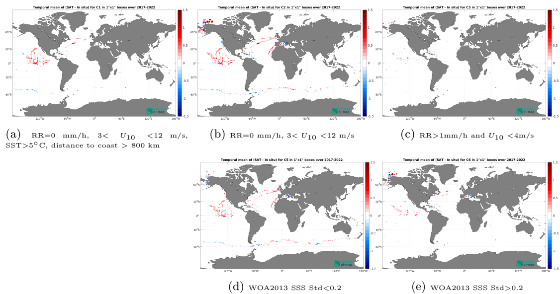
Figure 14: Temporal mean gridded over spatial boxes of size 1^\circ \times 1^\circ of \Delta SSS (SMOS SSS L3 v335 - Monthly - 25 km (CATDS-CPDC) - Saildrone) for 5 different subdatasets corresponding to:RR=0 mm/h, 3 < U_{10} < 12 m/s, SST > 5^\circ\text{C} , distance to coast > 800 km (a), RR=0 mm/h, 3 < U_{10} < 12 m/s (b), RR > 1 mm/h and U_{10} < 4 m/s (c), WOA2013 SSS Std < 0.2 (d), WOA2013 SSS Std > 0.2 (e).
