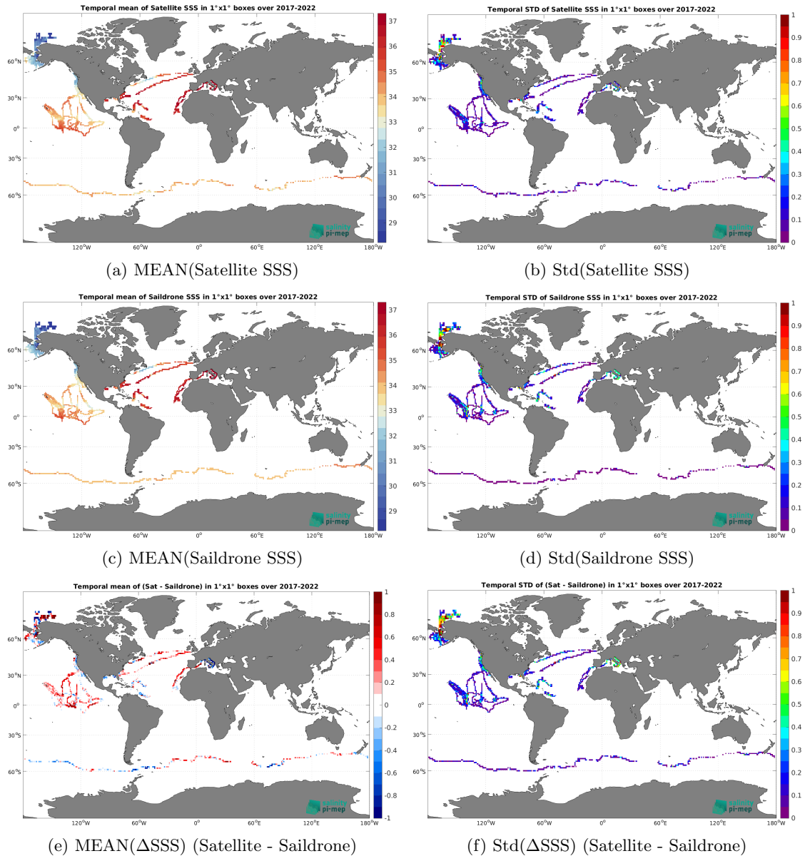
Figure 7: Temporal mean (left) and Std (right) of SSS from SMOS SSS L3 v335 - Monthly - 25 km (CATDS-CPDC) (top), Saildrone (middle), and of \Delta SSS (Satellite - Saildrone). Only match-up pairs are used to generate these maps.
