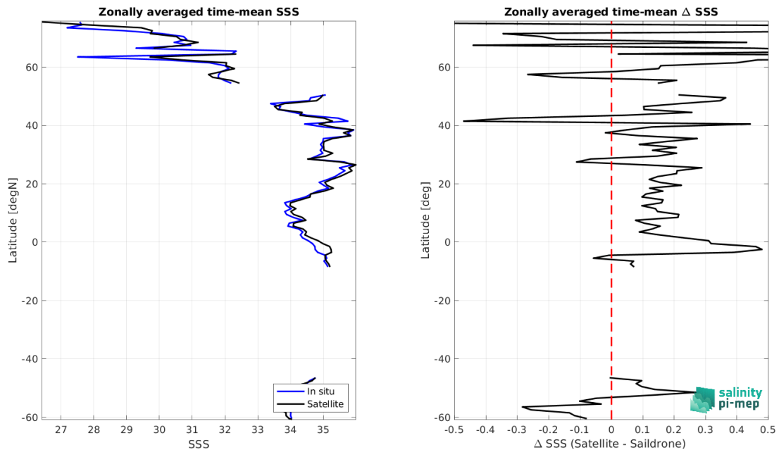
Figure 9: Left panel: Zonal mean SSS from SMOS SSS L3 v335 - Monthly - 25 km (CATDS-CPDC) satellite product (black) and from Saiddrone (blue). Right panel: Zonal mean of \Delta SSS (Satellite - Saiddrone) for all the collected Pi-MEP match-up pairs estimated over the full satellite product period.
