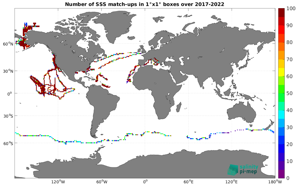
Figure 5: Number of SSS match-ups between Saildrone SSS and the SMOS SSS L3 v335 - Monthly - 25 km (CATDS-CPDC) SSS product for the Global Ocean Pi-MEP region over 1^\circ \times 1^\circ boxes and for the full satellite product period.
