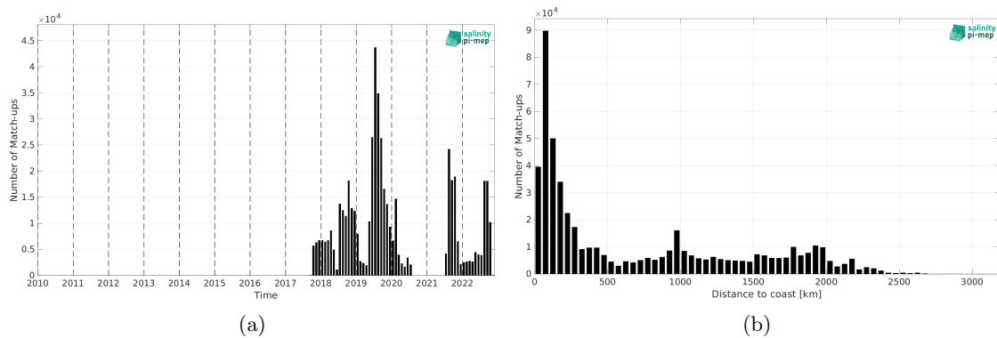
Figure 2: Number of match-ups between Saildrone and SMOS SSS L3 v335 - Monthly - 25 km (CATDS-CPDC) SSS as a function of time (a) and as function of the distance to coast (b) over the Global Ocean Pi-MEP region and for the full satellite product period.
