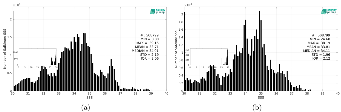
Figure 3: Histograms of SSS from Saildrone (a) and SMOS SSS L3 v335 - Monthly - 25 km (CATDS-CPDC) (b) considering all match-up pairs per bins of 0.1 over the Global Ocean Pi-MEP region and for the full satellite product period.
