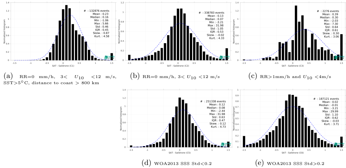
Figure 15: Normalized histogram of \Delta SSS (SMOS SSS L3 v335 - Monthly - 25 km (CATDS-CPDC) - Salldrone) for 5 different subdatasets corresponding to: RR=0 mm/h, 3 < U_{10} < 12 m/s, SST>5°C, distance to coast > 800 km (a), RR=0 mm/h, 3 < U_{10} < 12 m/s (b), RR>1mm/h and U_{10} < 4 m/s (c), WOA2013 SSS Std<0.2 (d), WOA2013 SSS Std>0.2 (e).
