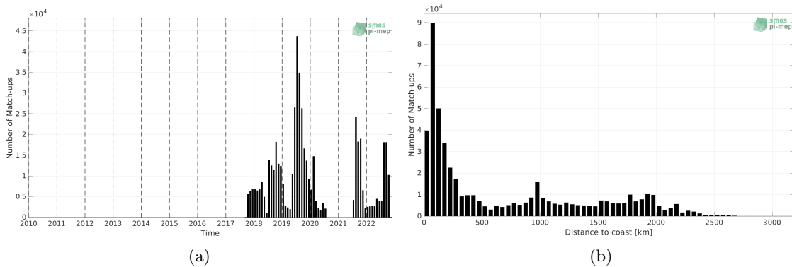
Figure 1: Number of match-ups between Saildrone and SMOS SSS L3 v335 - Monthly - 25 km (CATDS-CPDC) SSS as a function of time (a) and as function of the distance to coast (b) over the Global Ocean Pi-MEP region and for the full satellite product period.
