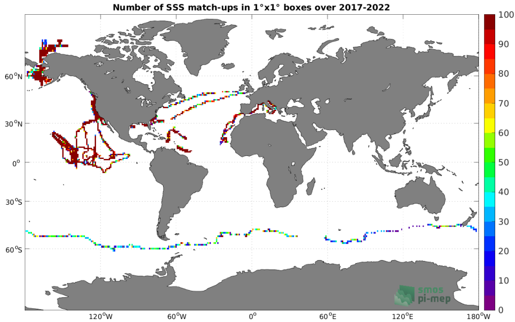
Figure 4: Number of SSS match-ups between Sairdrone SSS and the SMOS SSS L3 v335 - Monthly - 25 km (CATDS-CPDC) SSS product for the Global Ocean Pi-MEP region over 1^\circ \times 1^\circ boxes and for the full satellite product period.
