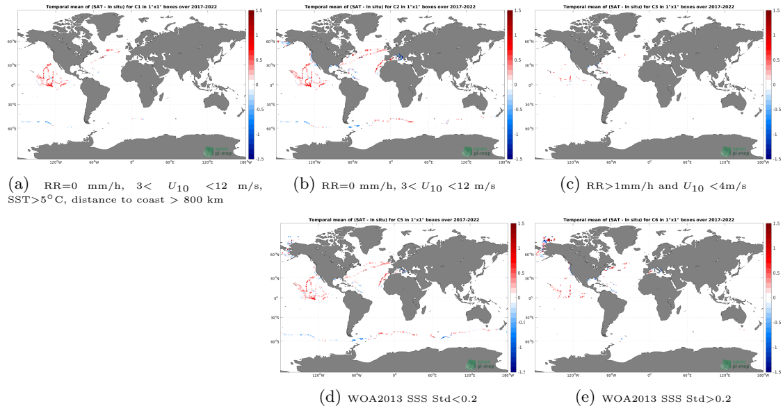
Figure 12: Temporal mean gridded over spatial boxes of size 1^\circ \times 1^\circ of \Delta SSS (SMOS SSS L3 v335 - Monthly - 25 km (CATDS-CPDC) - Saildrone) for 5 different subdatasets corresponding to:RR=0 mm/h, 3 < U_{10} < 12 m/s, SST > 5^\circ\text{C} , distance to coast > 800 km (a), RR=0 mm/h, 3 < U_{10} < 12 m/s (b), RR > 1 mm/h and U_{10} < 4 m/s (c), WOA2013 SSS Std < 0.2 (d), WOA2013 SSS Std > 0.2 (e).
