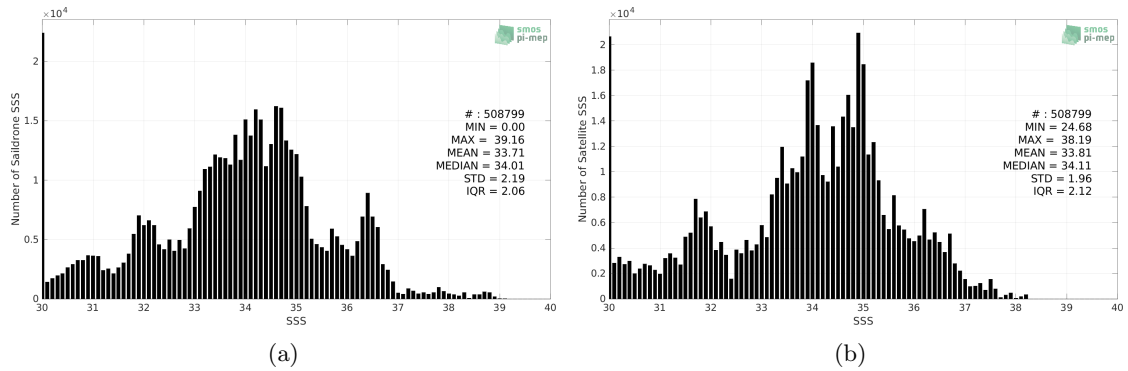
Figure 2: Histograms of SSS from Saildrone (a) and SMOS SSS L3 v335 - Monthly - 25 km (CATDS-CPDC) (b) considering all match-up pairs per bins of 0.1 over the Global Ocean Pi-MEP region and for the full satellite product period.
