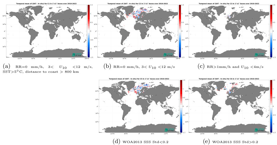
Figure 14: Temporal mean gridded over spatial boxes of size 1^\circ \times 1^\circ of \Delta SSS (SMOS SSS L3 v335 - Monthly - 25 km (CATDS-CPDC) - ICES) for 5 different subdatasets corresponding to: RR=0 mm/h, 3 < U_{10} < 12 m/s, SST > 5°C, distance to coast > 800 km (a), RR=0 mm/h, 3 < U_{10} < 12 m/s (b), RR > 1mm/h and U_{10} < 4 m/s (c), WOA2013 SSS Std < 0.2 (d), WOA2013 SSS Std > 0.2 (e).
