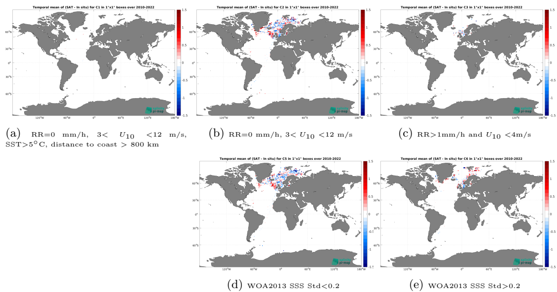
Figure 14: Temporal mean gridded over spatial boxes of size 1^\circ \times 1^\circ of \Delta SSS (SMOS SSS L3 v335 - Monthly - 25 km (CATDS-CPDC) - ICES) for 5 different subdatasets corresponding to:RR=0 mm/h, 3 < U_{10} < 12 m/s, SST > 5^\circ\text{C} , distance to coast > 800 km (a), RR=0 mm/h, 3 < U_{10} < 12 m/s (b), RR > 1 mm/h and U_{10} < 4 m/s (c), WOA2013 SSS Std < 0.2 (d), WOA2013 SSS Std > 0.2 (e).
