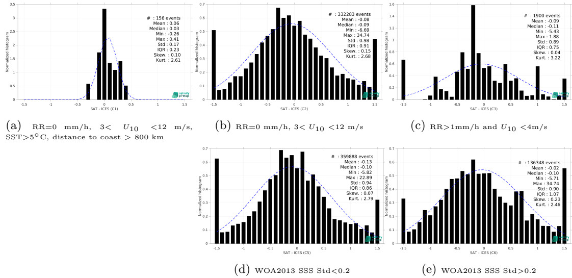
Figure 15: Normalized histogram of \Delta SSS (SMOS SSS L3 v335 - Monthly - 25 km (CATDS-CPDC) - ICES) for 5 different subdatasets corresponding to: RR=0 mm/h, 3 < U_{10} < 12 m/s, SST>5°C, distance to coast > 800 km (a), RR=0 mm/h, 3 < U_{10} < 12 m/s (b), RR>1mm/h and U_{10} < 4 m/s (c), WOA2013 SSS Std<0.2 (d), WOA2013 SSS Std>0.2 (e).
