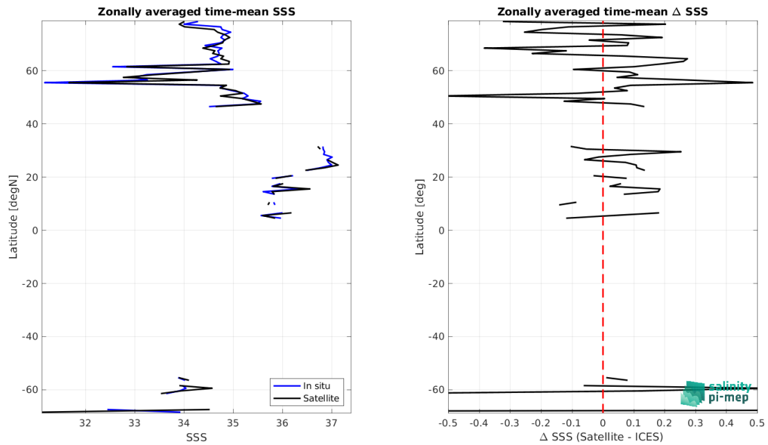
Figure 9: Left panel: Zonal mean SSS from SMOS SSS L3 v335 - Monthly - 25 km (CATDS-CPDC) satellite product (black) and from ICES (blue). Right panel: Zonal mean of \Delta SSS (Satellite - ICES) for all the collected Pi-MEP match-up pairs estimated over the full satellite product period.
