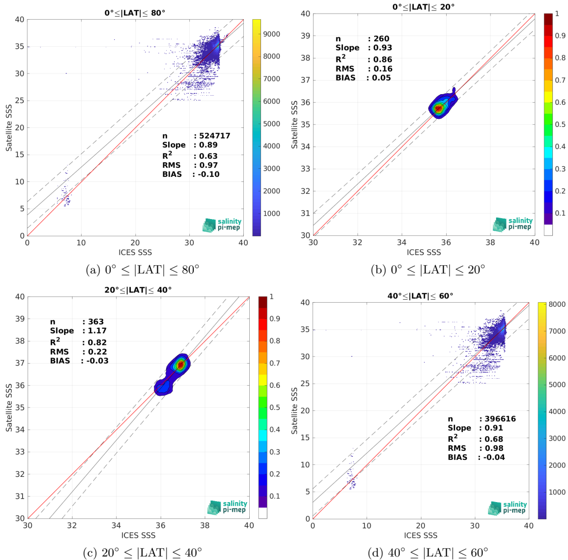
Figure 10: Contour maps of the concentration of SMOS SSS L3 v335 - Monthly - 25 km (CATDS-CPDC) SSS (y-axis) versus ICES SSS (x-axis) at match-up pairs for different latitude bands. For each plot, the red line shows x=y . The black thin and dashed lines indicate a linear fit through the data cloud and the \pm 95\% confidence levels, respectively. The number match-up pairs n , the slope and R^2 coefficient of the linear fit, the root mean square (RMS) and the mean bias between satellite and in situ data are indicated for each latitude band in each plots.
