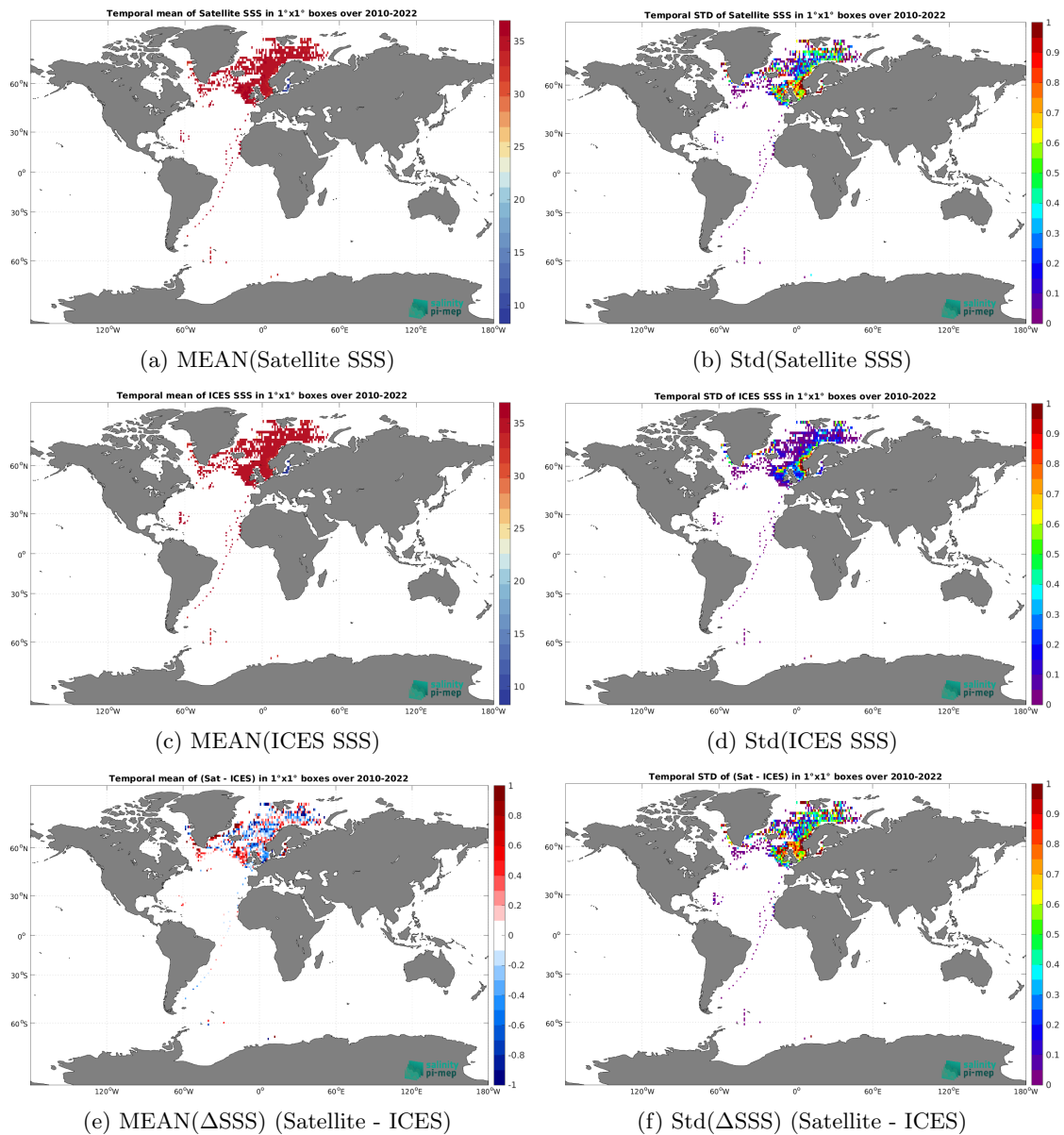
Figure 7: Temporal mean (left) and Std (right) of SSS from SMOS SSS L3 v335 - Monthly - 25 km (CATDS-CPDC) (top), ICES (middle), and of \Delta SSS (Satellite - ICES). Only match-up pairs are used to generate these maps.
