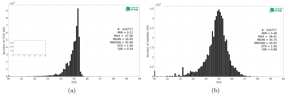
Figure 2: Histograms of SSS from ICES (a) and SMOS SSS L3 v335 - Monthly - 25 km (CATDS-CPDC) (b) considering all match-up pairs per bins of 0.1 over the Global Ocean Pi-MEP region and for the full satellite product period.
