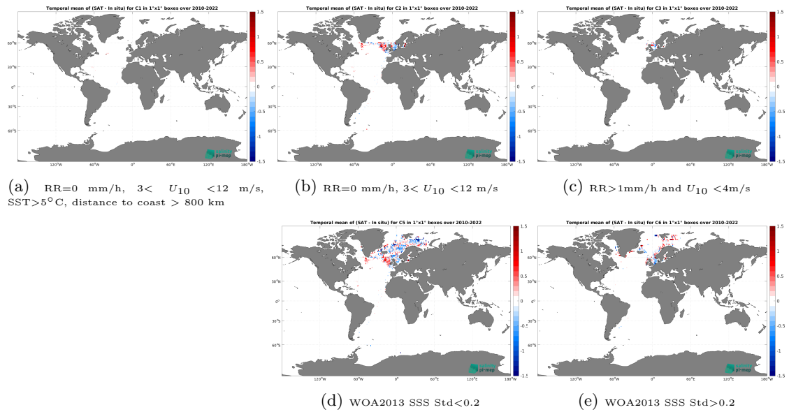
Figure 12: Temporal mean gridded over spatial boxes of size 1^\circ \times 1^\circ of \Delta SSS (SMOS SSS L3 v335 - Monthly - 25 km (CATDS-CPDC) - ICES) for 5 different subdatasets corresponding to:RR=0 mm/h, 3 < U_{10} < 12 m/s, SST >5^\circ C, distance to coast > 800 km (a), RR=0 mm/h, 3 < U_{10} < 12 m/s (b), RR >1 mm/h and U_{10} < 4 m/s (c), WOA2013 SSS Std <0.2 (d), WOA2013 SSS Std >0.2 (e).
