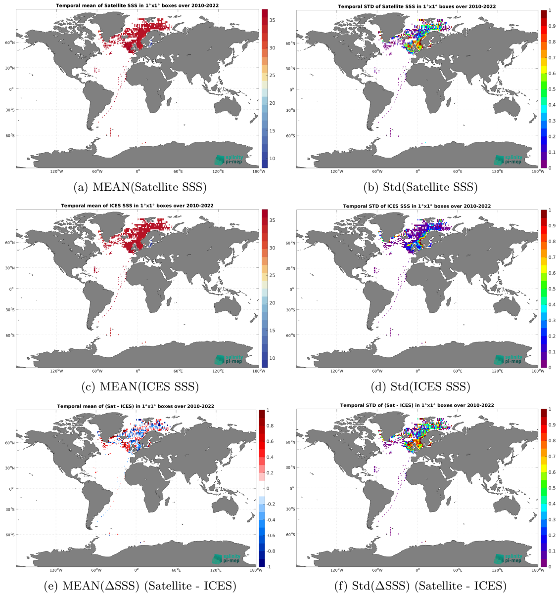
Figure 6: Temporal mean (left) and Std (right) of SSS from SMOS SSS L3 v335 - Monthly - 25 km (CATDS-CPDC) (top), ICES (middle), and of \Delta SSS (Satellite - ICES). Only match-up pairs are used to generate these maps.
