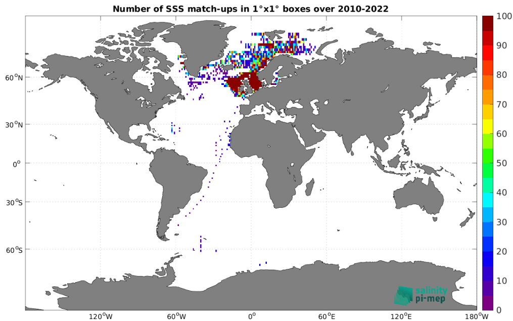
Figure 4: Number of SSS match-ups between ICES SSS and the SMOS SSS L3 v335 - Monthly - 25 km (CATDS-CPDC) SSS product for the Global Ocean Pi-MEP region over 1^\circ \times 1^\circ boxes and for the full satellite product period.
