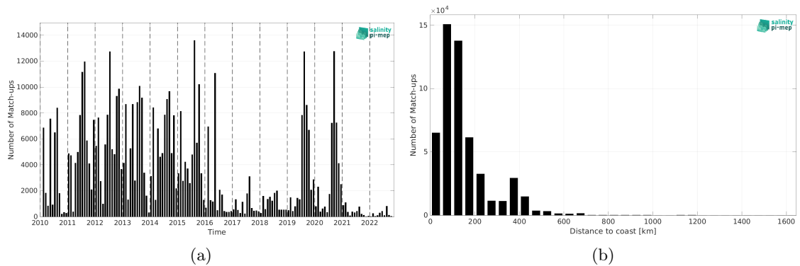
Figure 1: Number of match-ups between ICES and SMOS SSS L3 v335 - Monthly - 25 km (CATDS-CPDC) SSS as a function of time (a) and as function of the distance to coast (b) over the Global Ocean Pi-MEP region and for the full satellite product period.
