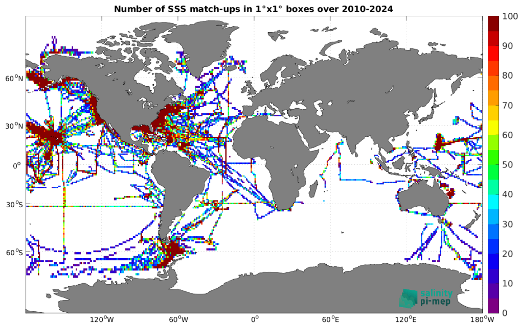
Figure 5: Number of SSS match-ups between TSG (SAMOS) SSS and the SMOS SSS L3 v335 - 10 Days - 25 km (CATDS-CPDC) SSS product for the Global Ocean Pi-MEP region over 1^\circ \times 1^\circ boxes and for the full satellite product period.
