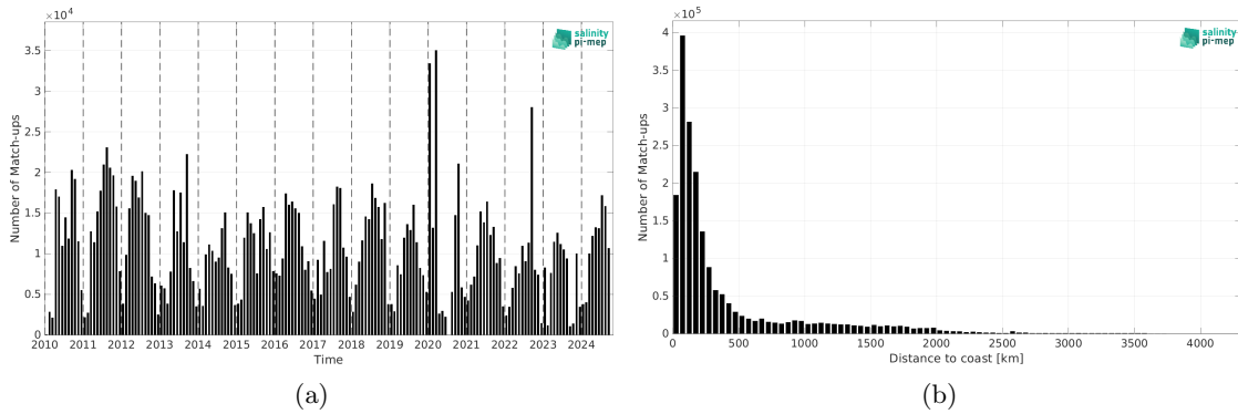
Figure 2: Number of match-ups between TSG (SAMOS) and SMOS SSS L3 v335 - 10 Days - 25 km (CATDS-CPDC) SSS as a function of time (a) and as function of the distance to coast (b) over the Global Ocean Pi-MEP region and for the full satellite product period.
