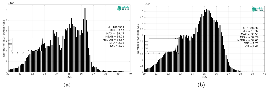
Figure 3: Histograms of SSS from TSG (SAMOS) (a) and SMOS SSS L3 v335 - 10 Days - 25 km (CATDS-CPDC) (b) considering all match-up pairs per bins of 0.1 over the Global Ocean Pi-MEP region and for the full satellite product period.
