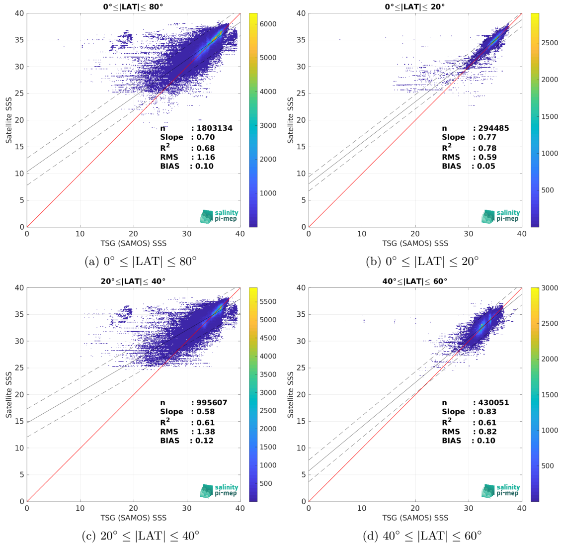
Figure 9: Contour maps of the concentration of SMOS SSS L3 v335 - 10 Days - 25 km (CATDS-CPDC) SSS (y-axis) versus TSG (SAMOS) SSS (x-axis) at match-up pairs for different latitude bands. For each plot, the red line shows x=y . The black thin and dashed lines indicate a linear fit through the data cloud and the \pm 95\% confidence levels, respectively. The number match-up pairs n , the slope and R^2 coefficient of the linear fit, the root mean square (RMS) and the mean bias between satellite and in situ data are indicated for each latitude band in each plots.
