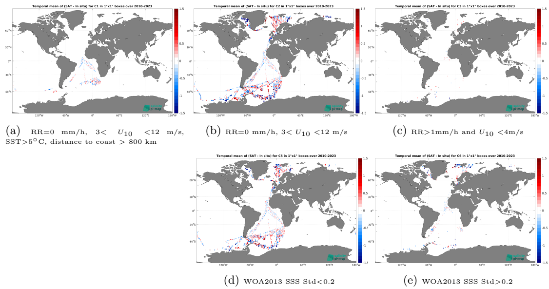
Figure 14: Temporal mean gridded over spatial boxes of size 1^\circ \times 1^\circ of \Delta SSS (SMOS SSS L3 v335 - 10 Days - 25 km (CATDS-CPDC) - TSG (Polarstern)) for 5 different subdatasets corresponding to: RR=0 mm/h, 3 < U_{10} < 12 m/s, SST > 5^\circ\text{C} , distance to coast > 800 km (a), RR=0 mm/h, 3 < U_{10} < 12 m/s (b), RR > 1 mm/h and U_{10} < 4 m/s (c), WOA2013 SSS Std < 0.2 (d), WOA2013 SSS Std > 0.2 (e).
