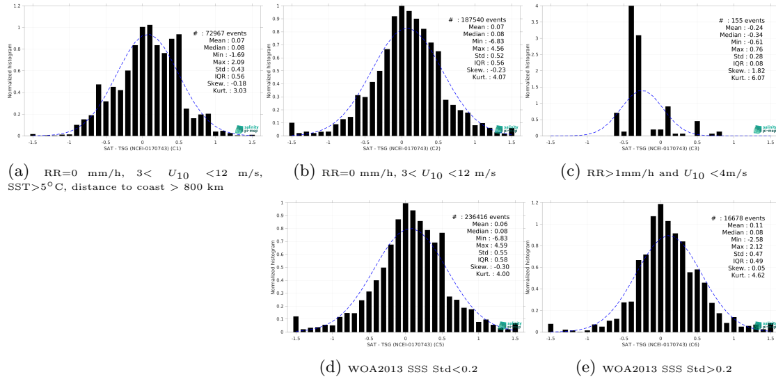
Figure 15: Normalized histogram of \Delta SSS (SMOS SSS L3 v335 - 10 Days - 25 km (CATDS-CPDC) - TSG (NCEI-0170743)) for 5 different subdatasets corresponding to: RR=0 mm/h, 3 < U_{10} < 12 m/s, SST>5°C, distance to coast > 800 km (a), RR=0 mm/h, 3 < U_{10} < 12 m/s (b), RR>1mm/h and U_{10} < 4 m/s (c), WOA2013 SSS Std<0.2 (d), WOA2013 SSS Std>0.2 (e).
