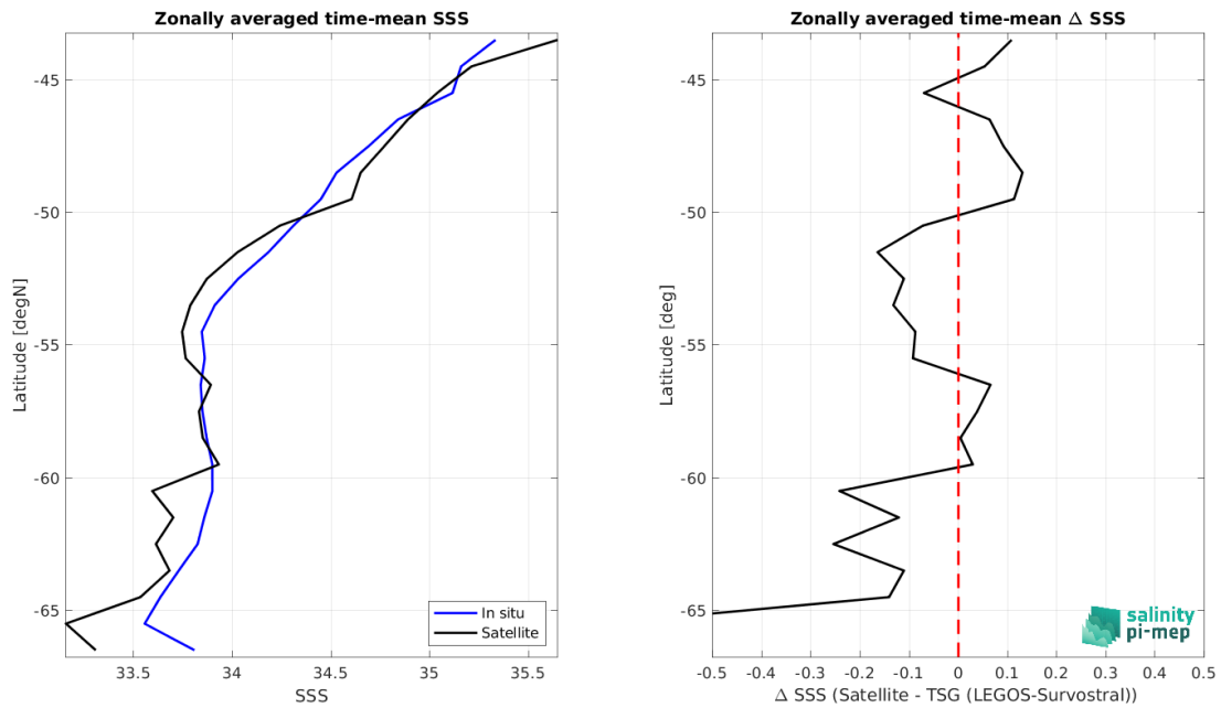
Figure 9: Left panel: Zonal mean SSS from SMOS SSS L3 v335 - 10 Days - 25 km (CATDS-CPDC) satellite product (black) and from TSG (LEGOS-Survostral) (blue). Right panel: Zonal mean of \Delta SSS (Satellite - TSG (LEGOS-Survostral)) for all the collected Pi-MEP match-up pairs estimated over the full satellite product period.
