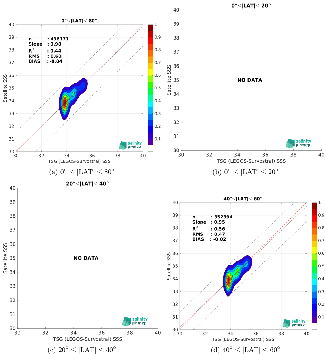
Figure 10: Contour maps of the concentration of SMOS SSS L3 v335 - 10 Days - 25 km (CATDS-CPDC) SSS (y-axis) versus TSG (LEGOS-Survostral) SSS (x-axis) at match-up pairs for different latitude bands. For each plot, the red line shows x=y . The black thin and dashed lines indicate a linear fit through the data cloud and the \pm 95\% confidence levels, respectively. The number match-up pairs n , the slope and R^2 coefficient of the linear fit, the root mean square (RMS) and the mean bias between satellite and in situ data are indicated for each latitude band in each plots.
