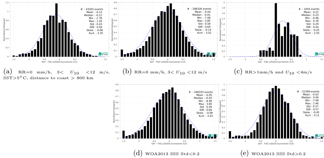
Figure 15: Normalized histogram of \Delta SSS (SMOS SSS L3 v335 - 10 Days - 25 km (CATDS-CPDC) - TSG (LEGOS-Survostral)) for 5 different subdatasets corresponding to: RR=0 mm/h, 3 < U_{10} < 12 m/s, SST>5°C, distance to coast > 800 km (a), RR=0 mm/h, 3 < U_{10} < 12 m/s (b), RR>1mm/h and U_{10} < 4 m/s (c), WOA2013 SSS Std<0.2 (d), WOA2013 SSS Std>0.2 (e).
