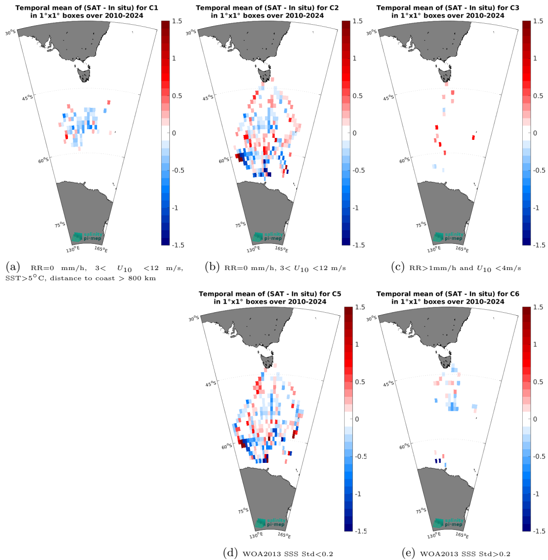
Figure 14: Temporal mean gridded over spatial boxes of size 1^\circ \times 1^\circ of \Delta\text{SSS} (SMOS SSS L3 v335 - 10 Days - 25 km (CATDS-CPDC) - TSG (LEGOS-Survostral)) for 5 different subdatasets corresponding to: RR=0 mm/h, 3 < U_{10} < 12 m/s, SST > 5^\circ\text{C} , distance to coast > 800 km (a), RR=0 mm/h, 3 < U_{10} < 12 m/s (b), RR > 1 mm/h and U_{10} < 4 m/s (c), WOA2013 SSS Std < 0.2 (d), WOA2013 SSS Std > 0.2 (e).
