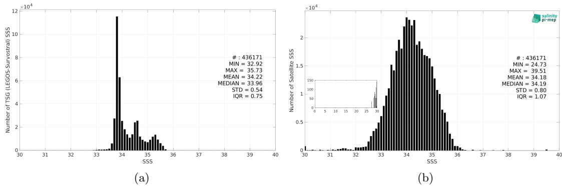
Figure 3: Histograms of SSS from TSG (LEGOS-Survostral) (a) and SMOS SSS L3 v335 - 10 Days - 25 km (CATDS-CPDC) (b) considering all match-up pairs per bins of 0.1 over the Global Ocean Pi-MEP region and for the full satellite product period.
