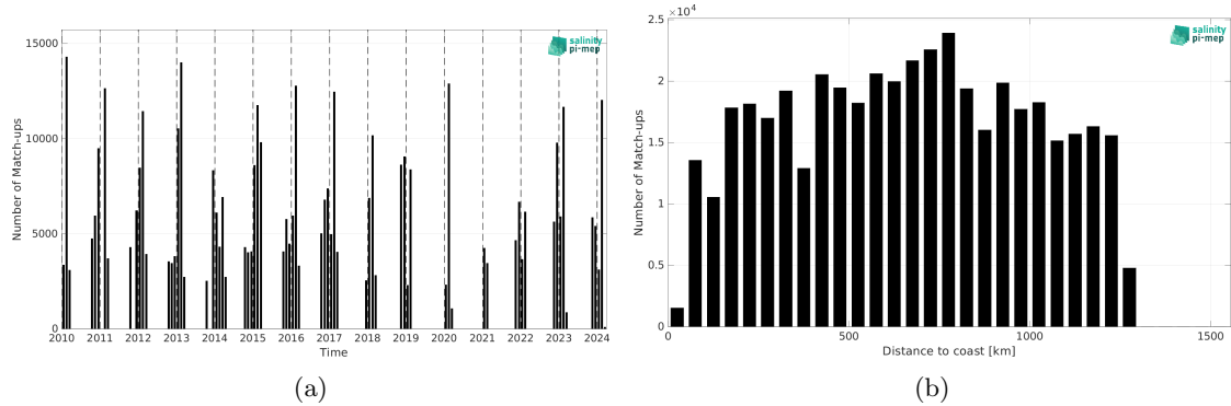
Figure 2: Number of match-ups between TSG (LEGOS-Survostral) and SMOS SSS L3 v335 - 10 Days - 25 km (CATDS-CPDC) SSS as a function of time (a) and as function of the distance to coast (b) over the Global Ocean Pi-MEP region and for the full satellite product period.
