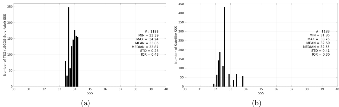
Figure 3: Histograms of SSS from TSG (LEGOS-Surv-Adel) (a) and SMOS SSS L3 v335 - 10 Days - 25 km (CATDS-CPDC) (b) considering all match-up pairs per bins of 0.1 over the Global Ocean Pi-MEP region and for the full satellite product period.
