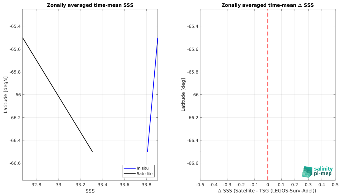
Figure 9: Left panel: Zonal mean SSS from SMOS SSS L3 v335 - 10 Days - 25 km (CATDS-CPDC) satellite product (black) and from TSG (LEGOS-Surv-Adel) (blue). Right panel: Zonal mean of \Delta SSS (Satellite - TSG (LEGOS-Surv-Adel)) for all the collected Pi-MEP match-up pairs estimated over the full satellite product period.
