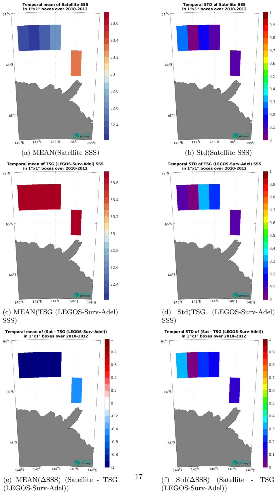
Figure 6: Temporal mean (left) and Std (right) of SSS from SMOS SSS L3 v335 - 10 Days - 25 km (CATDS-CPDC) (top), TSG (LEGOS-Surv-Adel) (middle), and of \Delta SSS (Satellite - TSG (LEGOS-Surv-Adel)). Only match-up pairs are used to generate these maps.
