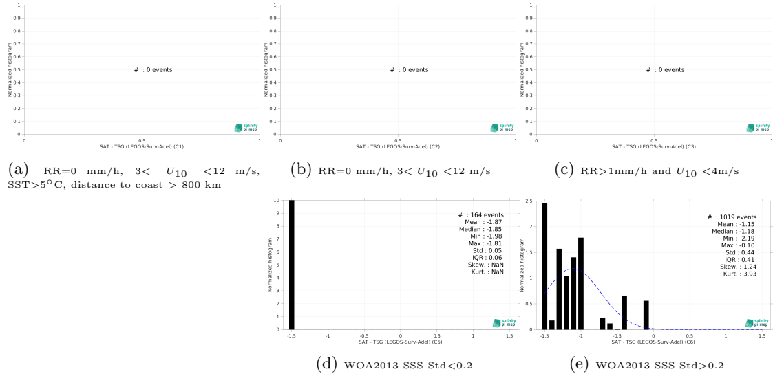
Figure 13: Normalized histogram of \Delta SSS (SMOS SSS L3 v335 - 10 Days - 25 km (CATDS-CPDC) - TSG (LEGOS-Surv-Adel)) for 5 different subdatasets corresponding to: RR=0 mm/h, 3 < U_{10} < 12 m/s, SST > 5°C, distance to coast > 800 km (a), RR=0 mm/h, 3 < U_{10} < 12 m/s (b), RR > 1mm/h and U_{10} < 4 m/s (c), WOA2013 SSS Std < 0.2 (d), WOA2013 SSS Std > 0.2 (e).
