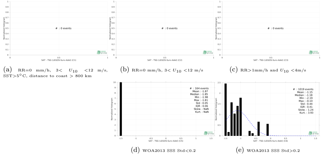
Figure 13: Normalized histogram of \Delta SSS (SMOS SSS L3 v335 - 10 Days - 25 km (CATDS-CPDC) - TSG (LEGOS-Surv-Adel)) for 5 different subdatasets corresponding to: RR=0 mm/h, 3 < U_{10} < 12 m/s, SST > 5°C, distance to coast > 800 km (a), RR=0 mm/h, 3 < U_{10} < 12 m/s (b), RR > 1mm/h and U_{10} < 4 m/s (c), WOA2013 SSS Std < 0.2 (d), WOA2013 SSS Std > 0.2 (e).
