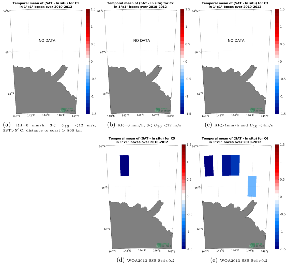
Figure 12: Temporal mean gridded over spatial boxes of size 1^\circ \times 1^\circ of \Delta SSS (SMOS SSS L3 v335 - 10 Days - 25 km (CATDS-CPDC) - TSG (LEGOS-Surv-Adel)) for 5 different subdatasets corresponding to:RR=0 mm/h, 3 < U_{10} < 12 m/s, SST>5°C, distance to coast > 800 km (a), RR=0 mm/h, 3 < U_{10} < 12 m/s (b), RR>1mm/h and U_{10} < 4 m/s (c), WOA2013 SSS Std<0.2 (d), WOA2013 SSS Std>0.2 (e).
