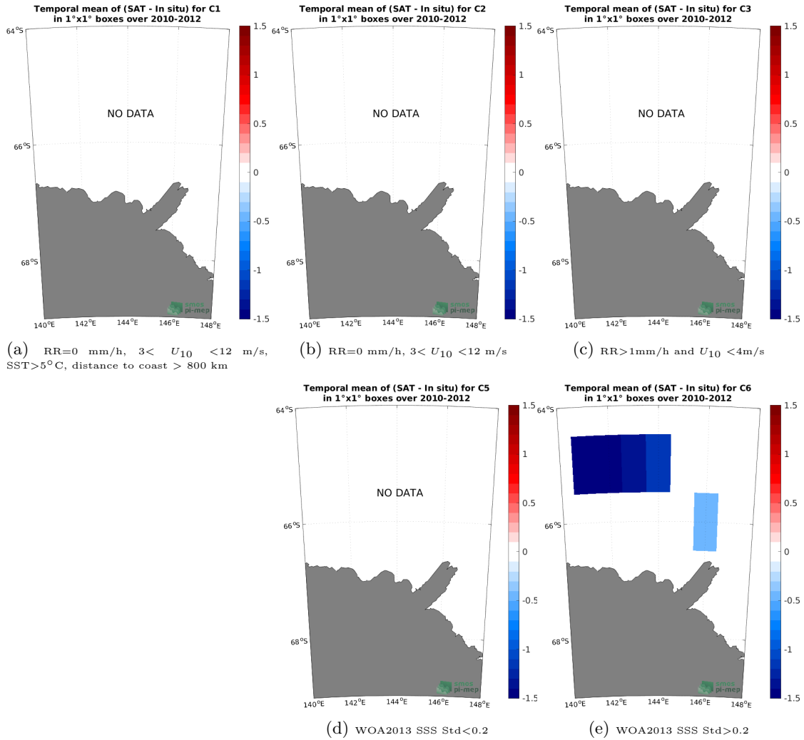
Figure 12: Temporal mean gridded over spatial boxes of size 1°x1° of \Delta SSS (SMOS SSS L3 v335 - 10 Days - 25 km (CATDS-CPDC) - TSG (LEGOS-Surv-Adel)) for 5 different subdatasets corresponding to:RR=0 mm/h, 3 < U_{10} < 12 m/s, SST>5°C, distance to coast > 800 km (a), RR=0 mm/h, 3 < U_{10} < 12 m/s (b), RR>1mm/h and U_{10} < 4 m/s (c), WOA2013 SSS Std<0.2 (d), WOA2013 SSS Std>0.2 (e).
