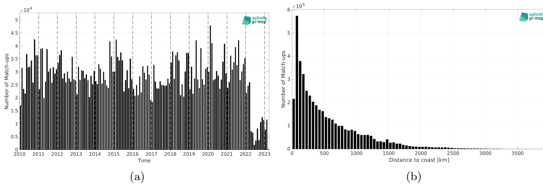
Figure 2: Number of match-ups between TSG (LEGOS-DM) and SMOS SSS L3 v335 - 10 Days - 25 km (CATDS-CPDC) SSS as a function of time (a) and as function of the distance to coast (b) over the Global Ocean Pi-MEP region and for the full satellite product period.
