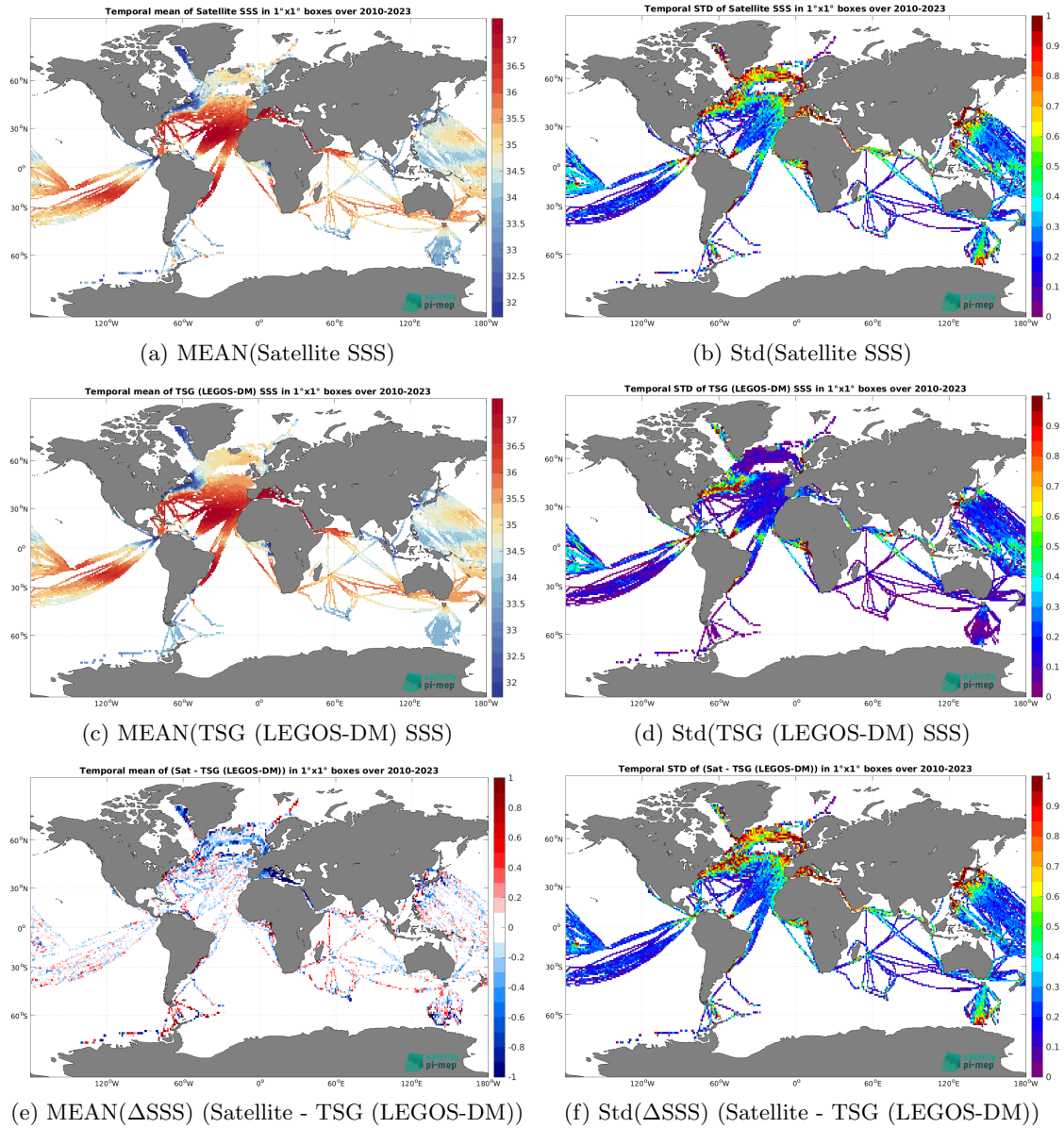
Figure 7: Temporal mean (left) and Std (right) of SSS from SMOS SSS L3 v335 - 10 Days - 25 km (CATDS-CPDC) (top), TSG (LEGOS-DM) (middle), and of \Delta SSS (Satellite - TSG (LEGOS-DM)). Only match-up pairs are used to generate these maps.
