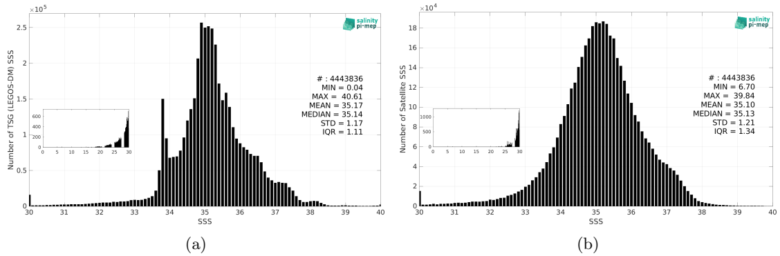
Figure 3: Histograms of SSS from TSG (LEGOS-DM) (a) and SMOS SSS L3 v335 - 10 Days - 25 km (CATDS-CPDC) (b) considering all match-up pairs per bins of 0.1 over the Global Ocean Pi-MEP region and for the full satellite product period.
