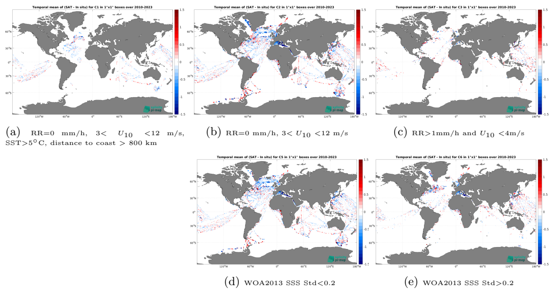
Figure 14: Temporal mean gridded over spatial boxes of size 1^\circ \times 1^\circ of \Delta SSS (SMOS SSS L3 v335 - 10 Days - 25 km (CATDS-CPDC) - TSG (LEGOS-DM)) for 5 different subdatasets corresponding to: RR=0 mm/h, 3 < U_{10} < 12 m/s, SST > 5^\circ\text{C} , distance to coast > 800 km (a), RR=0 mm/h, 3 < U_{10} < 12 m/s (b), RR > 1 mm/h and U_{10} < 4 m/s (c), WOA2013 SSS Std < 0.2 (d), WOA2013 SSS Std > 0.2 (e).
