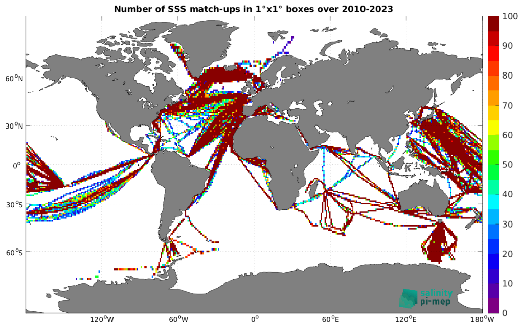
Figure 5: Number of SSS match-ups between TSG (LEGOS-DM) SSS and the SMOS SSS L3 v335 - 10 Days - 25 km (CATDS-CPDC) SSS product for the Global Ocean Pi-MEP region over 1^\circ \times 1^\circ boxes and for the full satellite product period.
