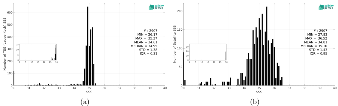
Figure 3: Histograms of SSS from TSG (Lauge-Koch) (a) and SMOS SSS L3 v335 - 10 Days - 25 km (CATDS-CPDC) (b) considering all match-up pairs per bins of 0.1 over the Global Ocean Pi-MEP region and for the full satellite product period.
