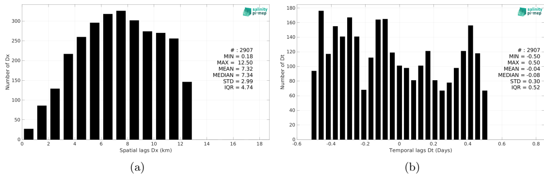
Figure 6: Histograms of the spatial (a) and temporal (b) lags between the location/time of the TSG (Lauge-Koch) measurement and the date of the corresponding SMOS SSS L3 v335 - 10 Days - 25 km (CATDS-CPDC) SSS pixel.
