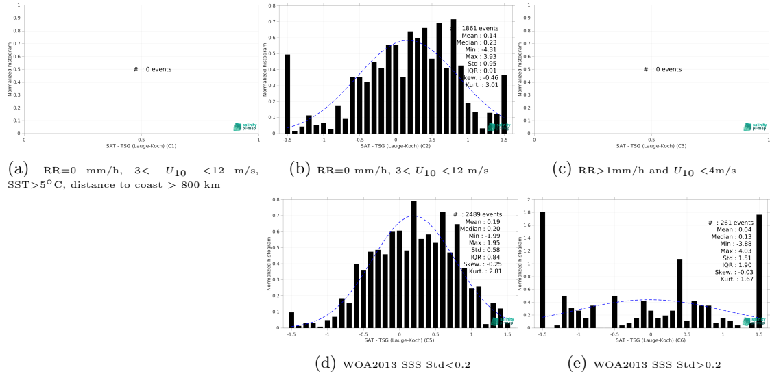
Figure 15: Normalized histogram of \Delta SSS (SMOS SSS L3 v335 - 10 Days - 25 km (CATDS-CPDC) - TSG (Lauge-Koch)) for 5 different subdatasets corresponding to: RR=0 mm/h, 3 < U_{10} < 12 m/s, SST > 5°C, distance to coast > 800 km (a), RR=0 mm/h, 3 < U_{10} < 12 m/s (b), RR > 1mm/h and U_{10} < 4 m/s (c), WOA2013 SSS Std < 0.2 (d), WOA2013 SSS Std > 0.2 (e).
