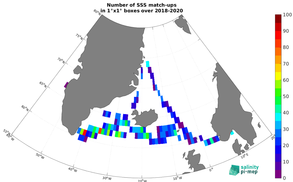
Figure 5: Number of SSS match-ups between TSG (Lauge-Koch) SSS and the SMOS SSS L3 v335 - 10 Days - 25 km (CATDS-CPDC) SSS product for the Global Ocean Pi-MEP region over 1^\circ \times 1^\circ boxes and for the full satellite product period.
