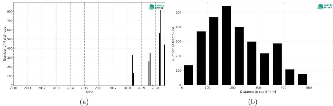
Figure 2: Number of match-ups between TSG (Lauge-Koch) and SMOS SSS L3 v335 - 10 Days - 25 km (CATDS-CPDC) SSS as a function of time (a) and as function of the distance to coast (b) over the Global Ocean Pi-MEP region and for the full satellite product period.
