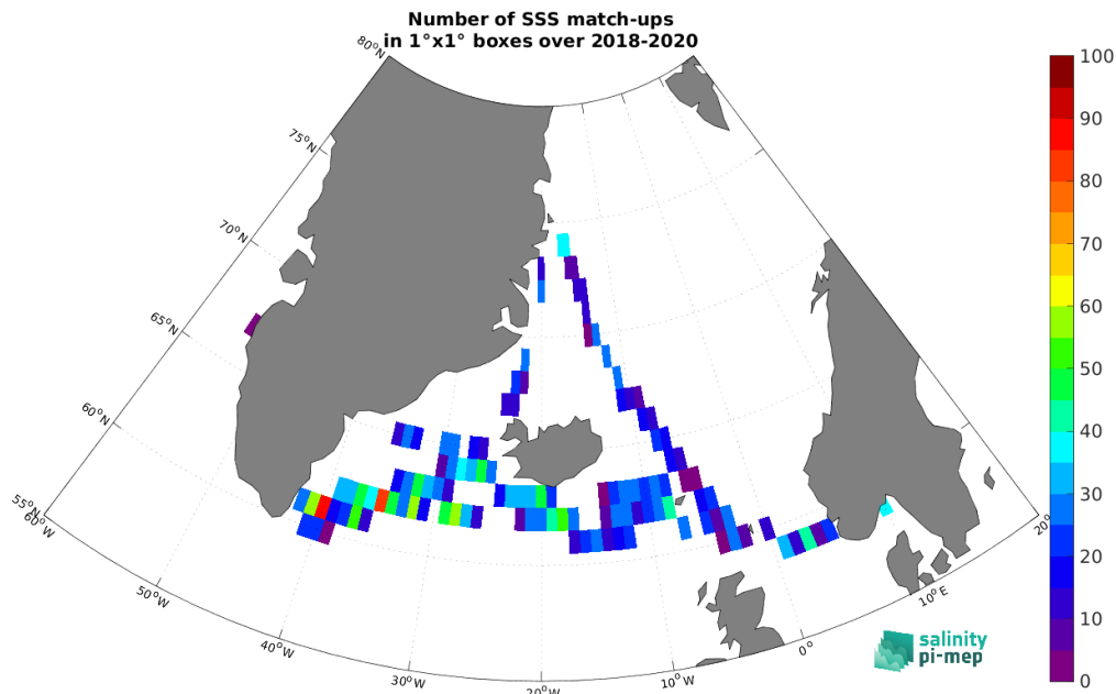
Figure 5: Number of SSS match-ups between TSG (Lauge-Koch) SSS and the SMOS SSS L3 v335 - 10 Days - 25 km (CATDS-CPDC) SSS product for the Global Ocean Pi-MEP region over 1^\circ \times 1^\circ boxes and for the full satellite product period.
