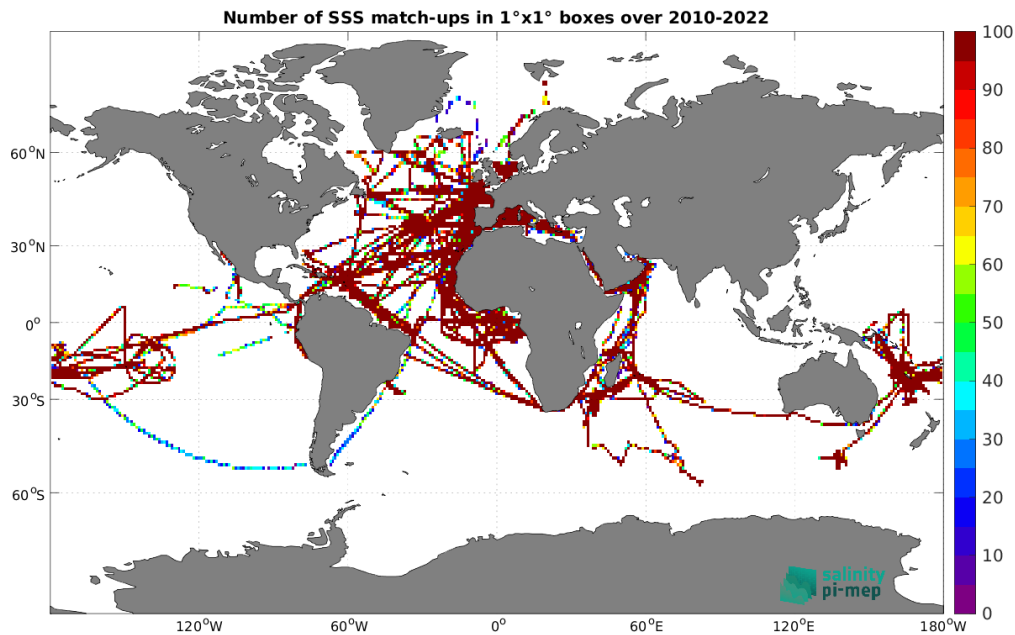
Figure 5: Number of SSS match-ups between TSG (GOSUD-Research-vessel) SSS and the SMOS SSS L3 v335 - 10 Days - 25 km (CATDS-CPDC) SSS product for the Global Ocean Pi-MEP region over 1^\circ \times 1^\circ boxes and for the full satellite product period.
