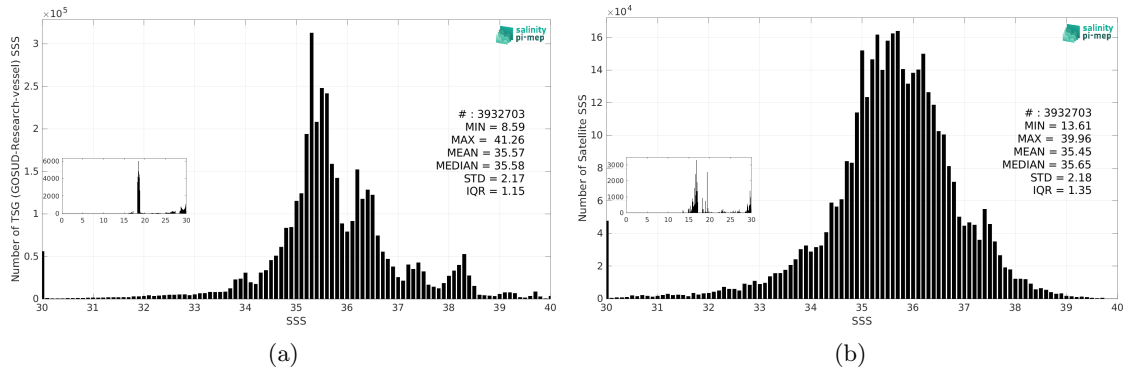
Figure 3: Histograms of SSS from TSG (GOSUD-Research-vessel) (a) and SMOS SSS L3 v335 - 10 Days - 25 km (CATDS-CPDC) (b) considering all match-up pairs per bins of 0.1 over the Global Ocean Pi-MEP region and for the full satellite product period.
