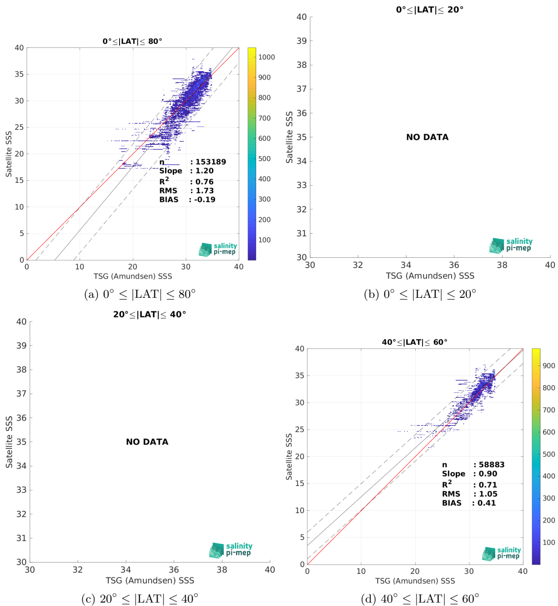
Figure 9: Contour maps of the concentration of SMOS SSS L3 v335 - 10 Days - 25 km (CATDS-CPDC) SSS (y-axis) versus TSG (Amundsen) SSS (x-axis) at match-up pairs for different latitude bands. For each plot, the red line shows x=y . The black thin and dashed lines indicate a linear fit through the data cloud and the \pm 95\% confidence levels, respectively. The number match-up pairs n , the slope and R^2 coefficient of the linear fit, the root mean square (RMS) and the mean bias between satellite and in situ data are indicated for each latitude band in each plots.
