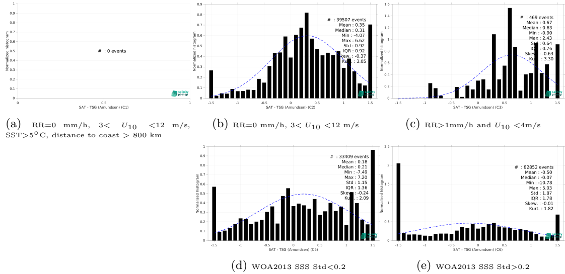
Figure 13: Normalized histogram of \Delta SSS (SMOS SSS L3 v335 - 10 Days - 25 km (CATDS-CPDC) - TSG (Amundsen)) for 5 different subdatasets corresponding to: RR=0 mm/h, 3 < U_{10} < 12 m/s, SST > 5°C, distance to coast > 800 km (a), RR=0 mm/h, 3 < U_{10} < 12 m/s (b), RR > 1mm/h and U_{10} < 4 m/s (c), WOA2013 SSS Std < 0.2 (d), WOA2013 SSS Std > 0.2 (e).
