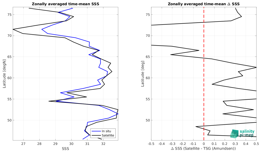
Figure 8: Left panel: Zonal mean SSS from SMOS SSS L3 v335 - 10 Days - 25 km (CATDS-CPDC) satellite product (black) and from TSG (Amundsen) (blue). Right panel: Zonal mean of \Delta SSS (Satellite - TSG (Amundsen)) for all the collected Pi-MEP match-up pairs estimated over the full satellite product period.
