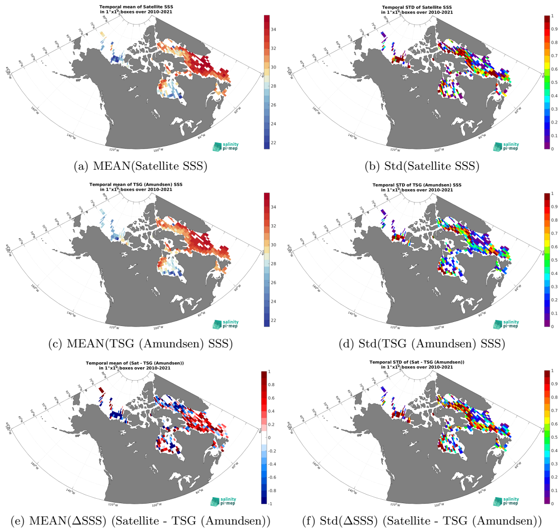
Figure 6: Temporal mean (left) and Std (right) of SSS from SMOS SSS L3 v335 - 10 Days - 25 km (CATDS-CPDC) (top), TSG (Amundsen) (middle), and of \Delta SSS (Satellite - TSG (Amundsen)). Only match-up pairs are used to generate these maps.
