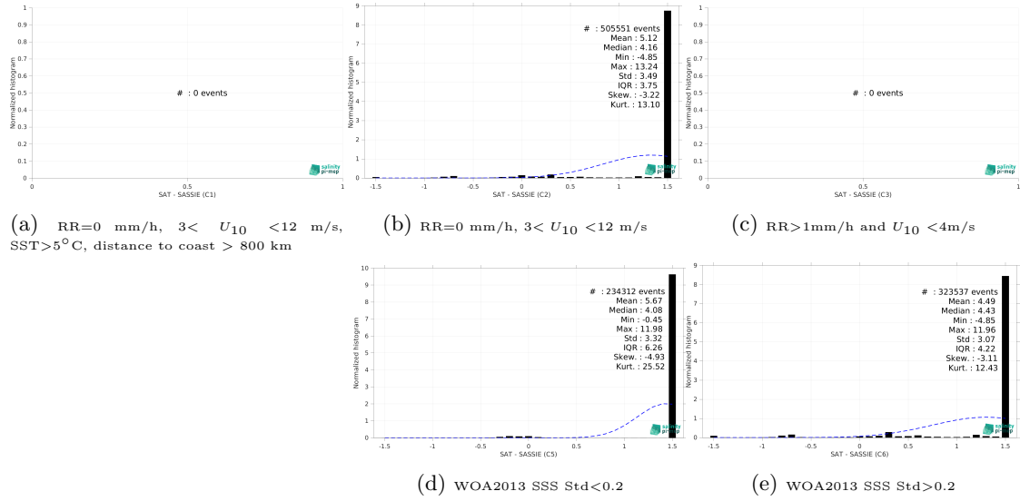
Figure 15: Normalized histogram of \Delta SSS (SMOS SSS L3 v335 - 10 Days - 25 km (CATDS-CPDC) - SASSIE) for 5 different subdatasets corresponding to: RR=0 mm/h, 3 < U_{10} < 12 m/s, SST>5°C, distance to coast > 800 km (a), RR=0 mm/h, 3 < U_{10} < 12 m/s (b), RR>1mm/h and U_{10} < 4 m/s (c), WOA2013 SSS Std<0.2 (d), WOA2013 SSS Std>0.2 (e).
