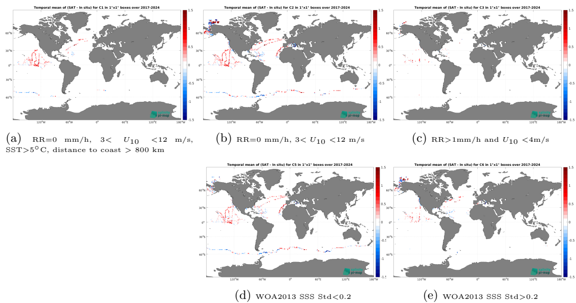
Figure 14: Temporal mean gridded over spatial boxes of size 1^\circ \times 1^\circ of \Delta SSS (SMOS SSS L3 v335 - 10 Days - 25 km (CATDS-CPDC) - Saildrone) for 5 different subdatasets corresponding to: RR=0 mm/h, 3 < U_{10} < 12 m/s, SST > 5^\circ\text{C} , distance to coast > 800 km (a), RR=0 mm/h, 3 < U_{10} < 12 m/s (b), RR > 1 mm/h and U_{10} < 4 m/s (c), WOA2013 SSS Std < 0.2 (d), WOA2013 SSS Std > 0.2 (e).
