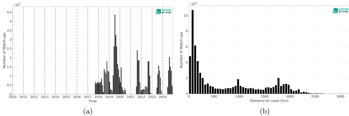
Figure 2: Number of match-ups between Saildrone and SMOS SSS L3 v335 - 10 Days - 25 km (CATDS-CPDC) SSS as a function of time (a) and as function of the distance to coast (b) over the Global Ocean Pi-MEP region and for the full satellite product period.
