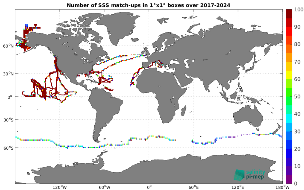
Figure 5: Number of SSS match-ups between Saildrone SSS and the SMOS SSS L3 v335 - 10 Days - 25 km (CATDS-CPDC) SSS product for the Global Ocean Pi-MEP region over 1^\circ \times 1^\circ boxes and for the full satellite product period.
