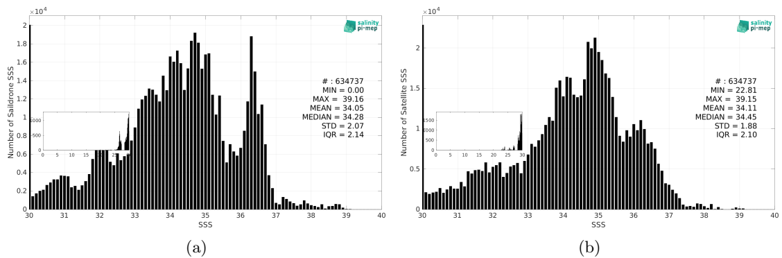
Figure 3: Histograms of SSS from Saildrone (a) and SMOS SSS L3 v335 - 10 Days - 25 km (CATDS-CPDC) (b) considering all match-up pairs per bins of 0.1 over the Global Ocean Pi-MEP region and for the full satellite product period.
