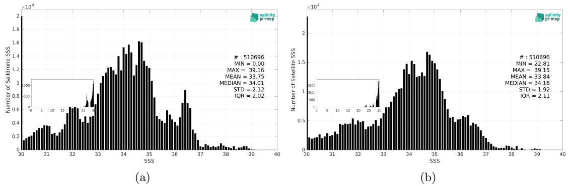
Figure 3: Histograms of SSS from Saldrone (a) and SMOS SSS L3 v335 - 10 Days - 25 km (CATDS-CPDC) (b) considering all match-up pairs per bins of 0.1 over the Global Ocean Pi-MEP region and for the full satellite product period.
