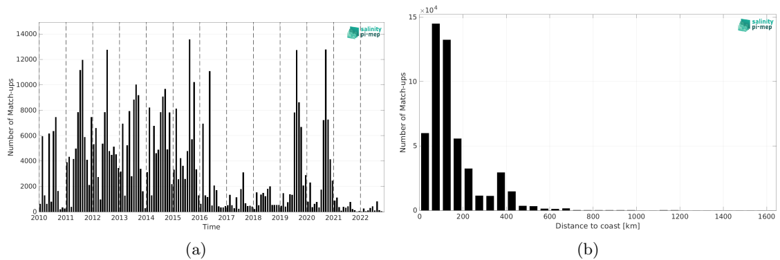
Figure 2: Number of match-ups between ICES and SMOS SSS L3 v335 - 10 Days - 25 km (CATDS-CPDC) SSS as a function of time (a) and as function of the distance to coast (b) over the Global Ocean Pi-MEP region and for the full satellite product period.
