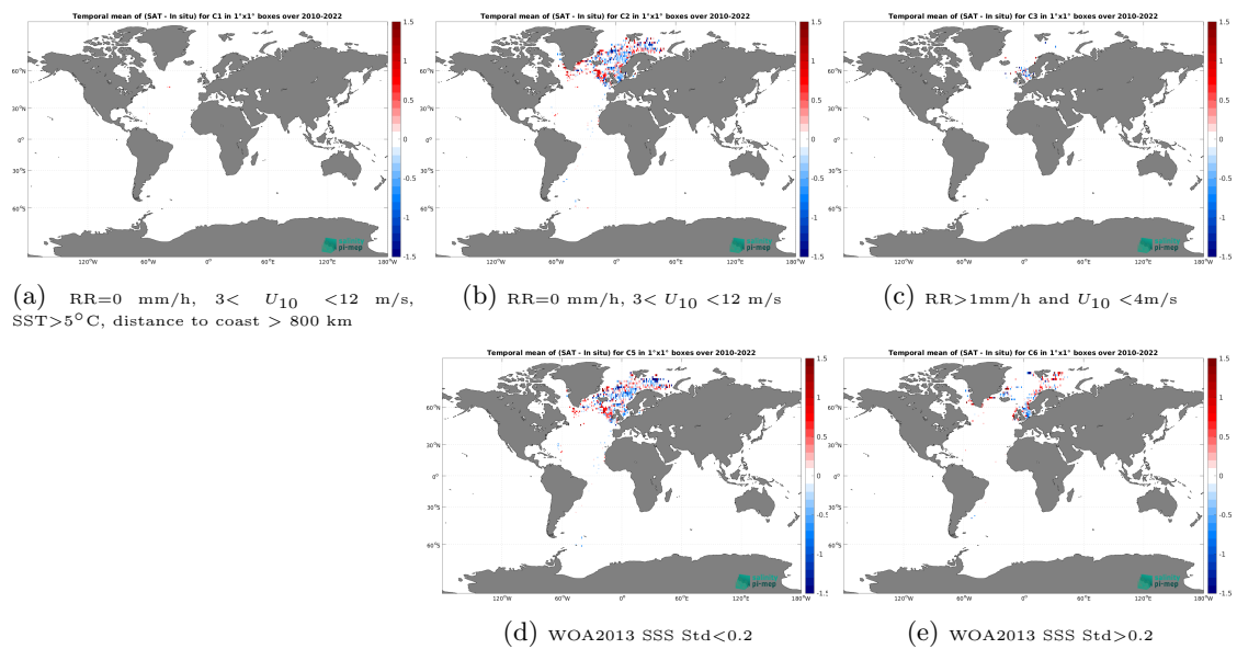
Figure 14: Temporal mean gridded over spatial boxes of size 1^\circ \times 1^\circ of \Delta SSS (SMOS SSS L3 v335 - 10 Days - 25 km (CATDS-CPDC) - ICES) for 5 different subdatasets corresponding to:RR=0 mm/h, 3 < U_{10} < 12 m/s, SST > 5^\circ\text{C} , distance to coast > 800 km (a), RR=0 mm/h, 3 < U_{10} < 12 m/s (b), RR > 1 mm/h and U_{10} < 4 m/s (c), WOA2013 SSS Std < 0.2 (d), WOA2013 SSS Std > 0.2 (e).
