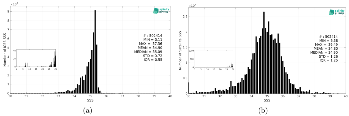
Figure 3: Histograms of SSS from ICES (a) and SMOS SSS L3 v335 - 10 Days - 25 km (CATDS-CPDC) (b) considering all match-up pairs per bins of 0.1 over the Global Ocean Pi-MEP region and for the full satellite product period.
