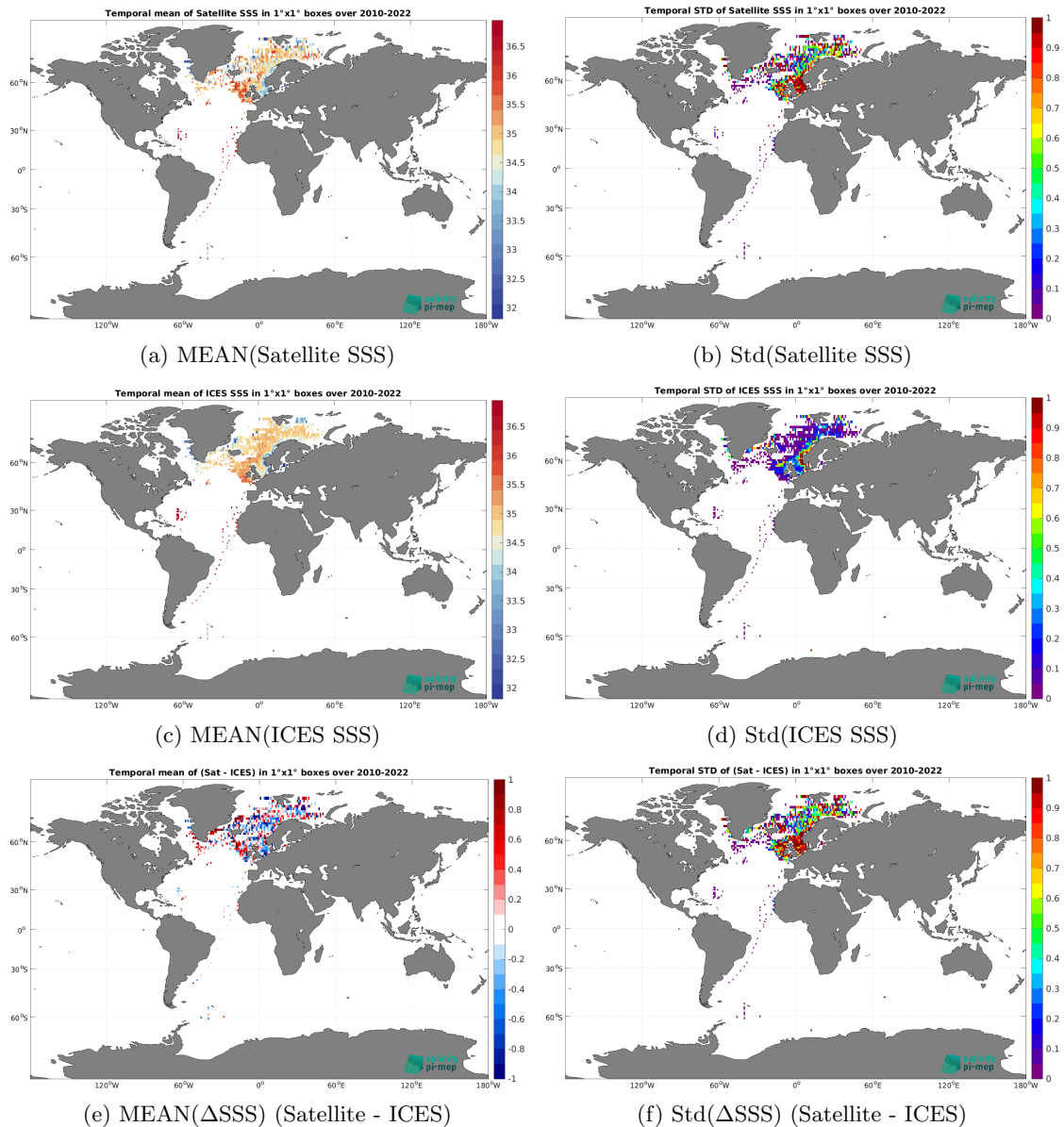
Figure 7: Temporal mean (left) and Std (right) of SSS from SMOS SSS L3 v335 - 10 Days - 25 km (CATDS-CPDC) (top), ICES (middle), and of \Delta SSS (Satellite - ICES). Only match-up pairs are used to generate these maps.
