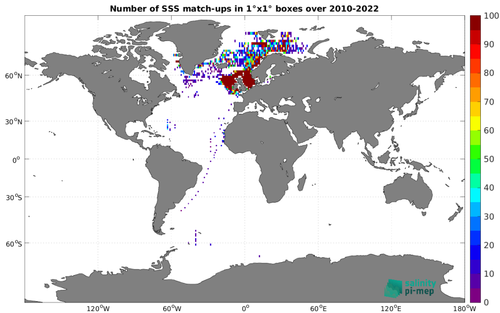
Figure 5: Number of SSS match-ups between ICES SSS and the SMOS SSS L3 v335 - 10 Days - 25 km (CATDS-CPDC) SSS product for the Global Ocean Pi-MEP region over 1^\circ \times 1^\circ boxes and for the full satellite product period.
