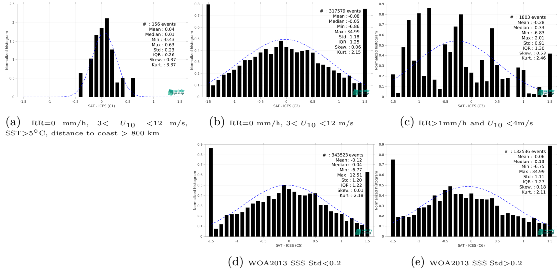
Figure 15: Normalized histogram of \Delta SSS (SMOS SSS L3 v335 - 10 Days - 25 km (CATDS-CPDC) - ICES) for 5 different subdatasets corresponding to: RR=0 mm/h, 3 < U_{10} < 12 m/s, SST > 5°C, distance to coast > 800 km (a), RR=0 mm/h, 3 < U_{10} < 12 m/s (b), RR > 1mm/h and U_{10} < 4 m/s (c), WOA2013 SSS Std < 0.2 (d), WOA2013 SSS Std > 0.2 (e).
