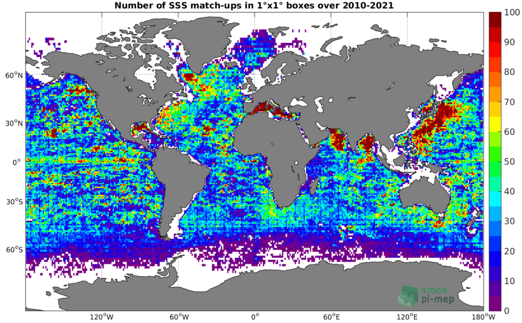
Figure 4: Number of SSS match-ups between Argo SSS and the SMOS SSS L3 v335 - 10 Days - 25 km (CATDS-CPDC) SSS product for the Global Ocean Pi-MEP region over 1^\circ \times 1^\circ boxes and for the full satellite product period.
