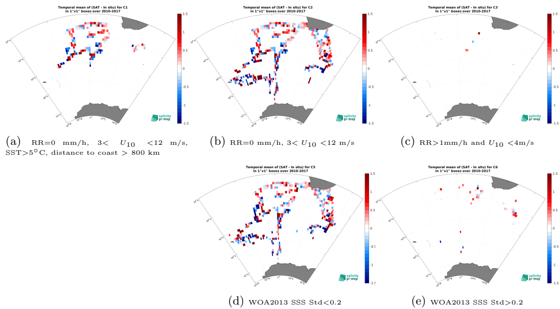
Figure 14: Temporal mean gridded over spatial boxes of size 1^\circ \times 1^\circ of \Delta\text{SSS} (SMOS SSS L2Q v333 - 0.25 Deg (CATDS-CPDC) - TSG (NCEI-0170743)) for 5 different subdatasets corresponding to: RR=0 mm/h, 3 < U_{10} < 12 m/s, SST > 5°C, distance to coast > 800 km (a), RR=0 mm/h, 3 < U_{10} < 12 m/s (b), RR > 1mm/h and U_{10} < 4 m/s (c), WOA2013 SSS Std < 0.2 (d), WOA2013 SSS Std > 0.2 (e).
