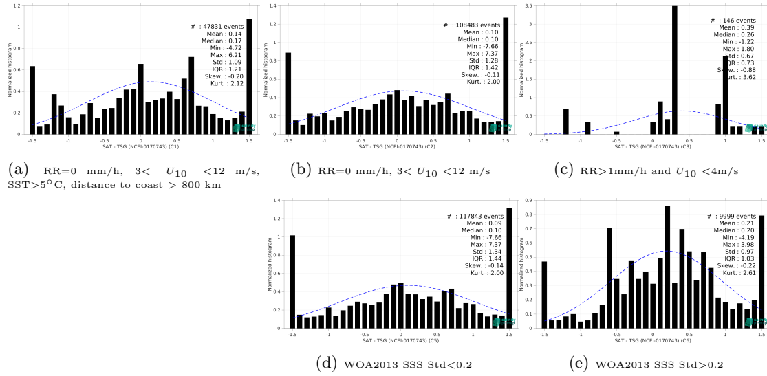
Figure 15: Normalized histogram of \Delta SSS (SMOS SSS L2Q v333 - 0.25 Deg (CATDS-CPDC) - TSG (NCEI-0170743)) for 5 different subdatasets corresponding to: RR=0 mm/h, 3 < U_{10} < 12 m/s, SST>5°C, distance to coast > 800 km (a), RR=0 mm/h, 3 < U_{10} < 12 m/s (b), RR>1mm/h and U_{10} < 4 m/s (c), WOA2013 SSS Std<0.2 (d), WOA2013 SSS Std>0.2 (e).
