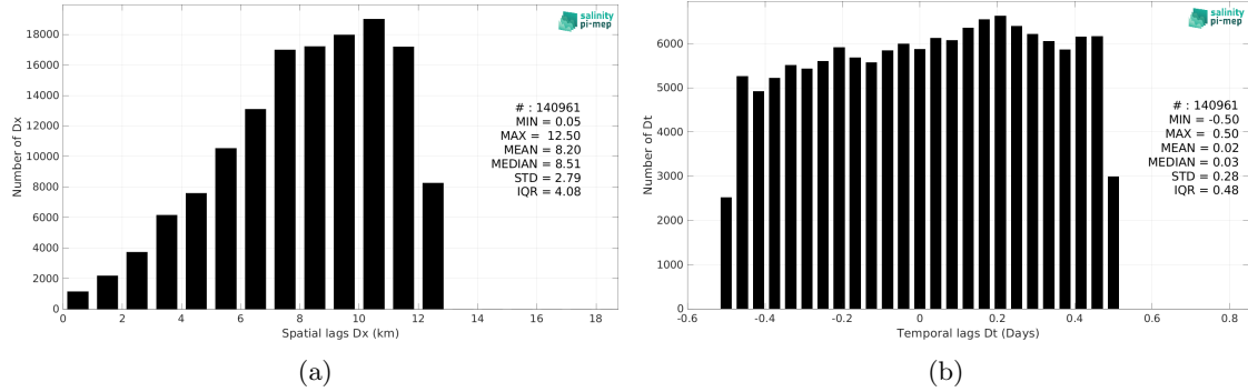
Figure 6: Histograms of the spatial (a) and temporal (b) lags between the location/time of the TSG (NCEI-0170743) measurement and the date of the corresponding SMOS SSS L2Q v333 - 0.25 Deg (CATDS-CPDC) SSS pixel.
