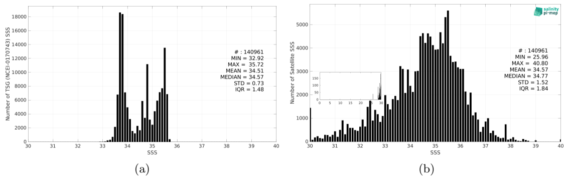
Figure 3: Histograms of SSS from TSG (NCEI-0170743) (a) and SMOS SSS L2Q v333 - 0.25 Deg (CATDS-CPDC) (b) considering all match-up pairs per bins of 0.1 over the Global Ocean Pi-MEP region and for the full satellite product period.
