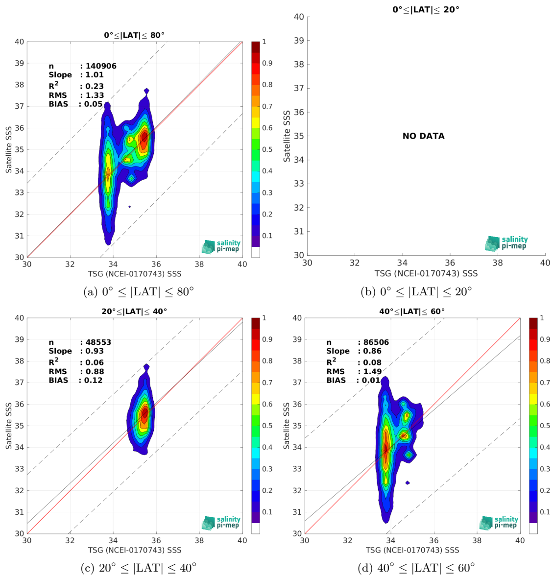
Figure 10: Contour maps of the concentration of SMOS SSS L2Q v333 - 0.25 Deg (CATDS-CPDC) SSS (y-axis) versus TSG (NCEI-0170743) SSS (x-axis) at match-up pairs for different latitude bands. For each plot, the red line shows x=y . The black thin and dashed lines indicate a linear fit through the data cloud and the \pm 95\% confidence levels, respectively. The number match-up pairs n , the slope and R^2 coefficient of the linear fit, the root mean square (RMS) and the mean bias between satellite and in situ data are indicated for each latitude band in each plots.
