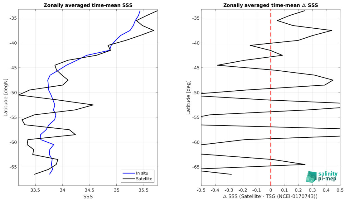
Figure 9: Left panel: Zonal mean SSS from SMOS SSS L2Q v333 - 0.25 Deg (CATDS-CPDC) satellite product (black) and from TSG (NCEI-0170743) (blue). Right panel: Zonal mean of \Delta SSS (Satellite - TSG (NCEI-0170743)) for all the collected Pi-MEP match-up pairs estimated over the full satellite product period.
