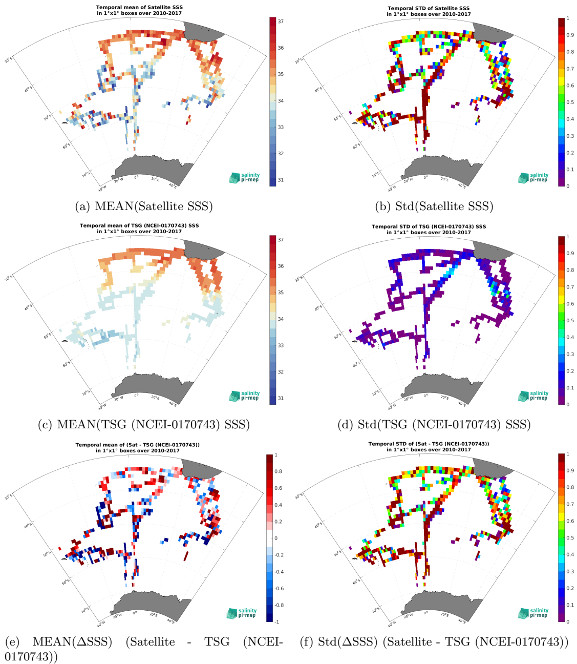
Figure 7: Temporal mean (left) and Std (right) of SSS from SMOS SSS L2Q v333 - 0.25 Deg (CATDS-CPDC) (top), TSG (NCEI-0170743) (middle), and of \Delta SSS (Satellite - TSG (NCEI-0170743)). Only match-up pairs are used to generate these maps.
