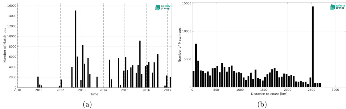
Figure 2: Number of match-ups between TSG (NCEI-0170743) and SMOS SSS L2Q v333 - 0.25 Deg (CATDS-CPDC) SSS as a function of time (a) and as function of the distance to coast (b) over the Global Ocean Pi-MEP region and for the full satellite product period.
