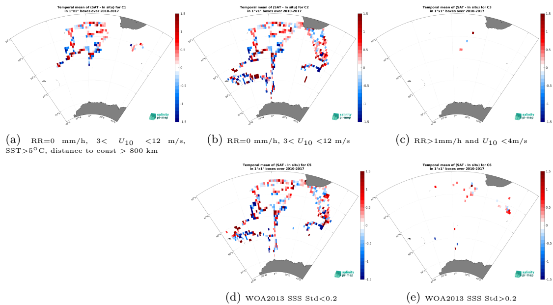
Figure 14: Temporal mean gridded over spatial boxes of size 1^\circ \times 1^\circ of \Delta SSS (SMOS SSS L2Q v333 - 0.25 Deg (CATDS-CPDC) - TSG (NCEI-0170743)) for 5 different subdatasets corresponding to:RR=0 mm/h, 3 < U_{10} < 12 m/s, SST >5^\circ C, distance to coast > 800 km (a), RR=0 mm/h, 3 < U_{10} < 12 m/s (b), RR >1 mm/h and U_{10} < 4 m/s (c), WOA2013 SSS Std <0.2 (d), WOA2013 SSS Std >0.2 (e).
