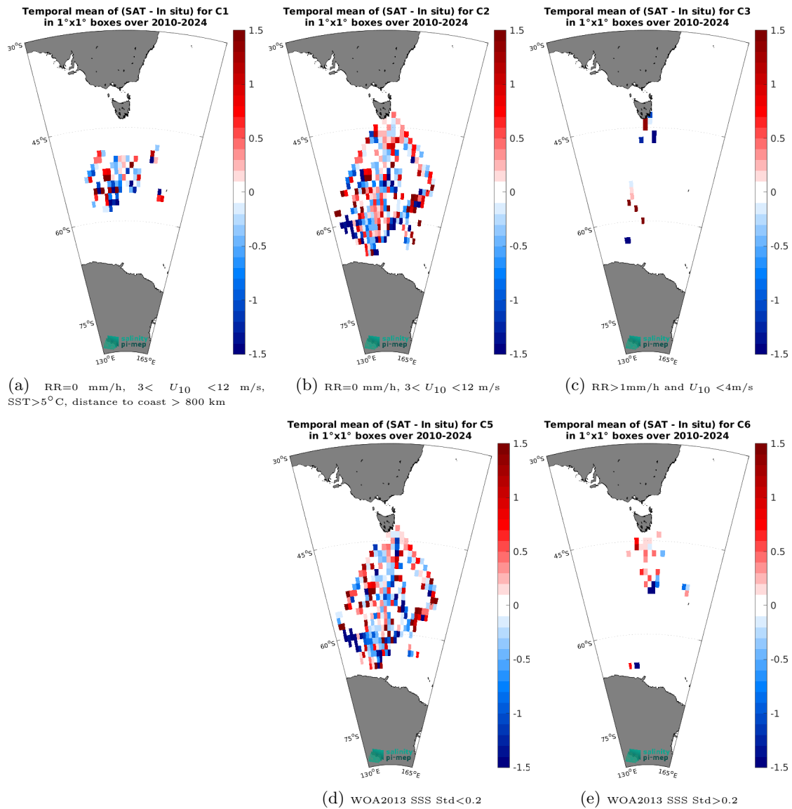
Figure 14: Temporal mean gridded over spatial boxes of size 1^\circ \times 1^\circ of \Delta SSS (SMOS SSS L2Q v333 - 0.25 Deg (CATDS-CPDC) - TSG (LEGOS-Survostral)) for 5 different subdatasets corresponding to:RR=0 mm/h, 3 < U_{10} < 12 m/s, SST>5°C, distance to coast > 800 km (a), RR=0 mm/h, 3 < U_{10} < 12 m/s (b), RR>1mm/h and U_{10} < 4 m/s (c), WOA2013 SSS Std<0.2 (d), WOA2013 SSS Std>0.2 (e).
