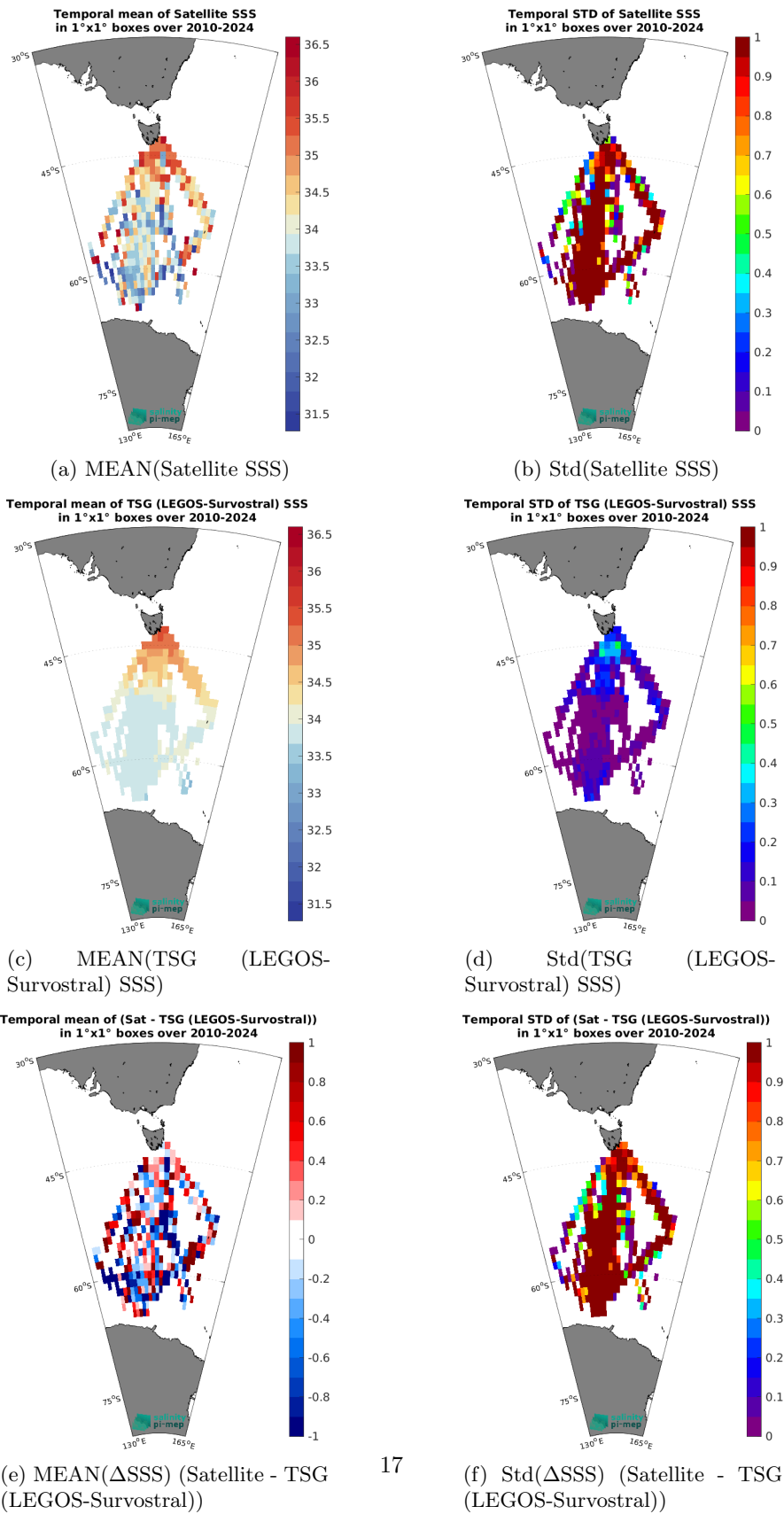
Figure 7: Temporal mean (left) and Std (right) of SSS from SMOS SSS L2Q v333 - 0.25 Deg (CATDS-CPDC) (top), TSG (LEGOS-Survostral) (middle), and of \Delta SSS (Satellite - TSG (LEGOS-Survostral)). Only match-up pairs are used to generate these maps.
