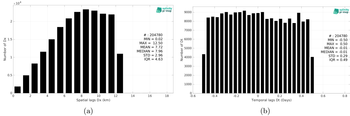
Figure 6: Histograms of the spatial (a) and temporal (b) lags between the location/time of the TSG (LEGOS-Survostral) measurement and the date of the corresponding SMOS SSS L2Q v333 - 0.25 Deg (CATDS-CPDC) SSS pixel.
