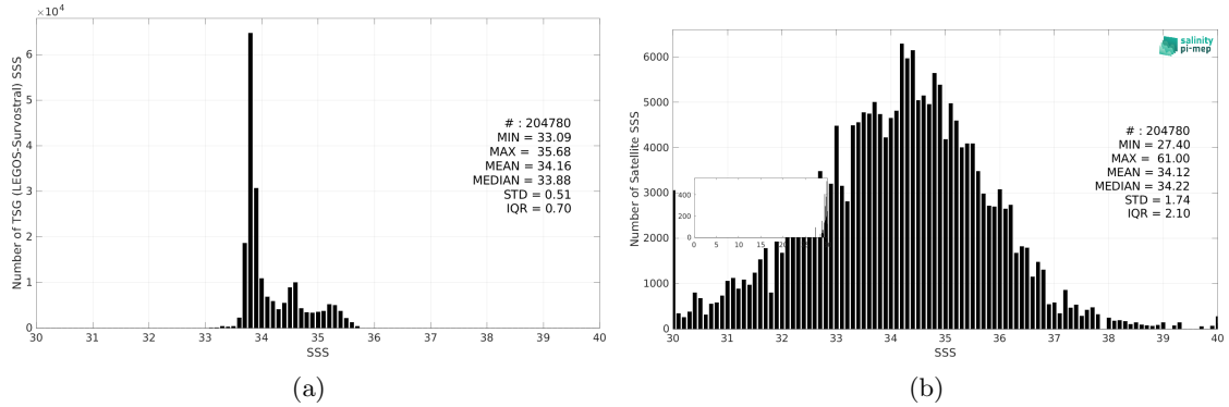
Figure 3: Histograms of SSS from TSG (LEGOS-Survostral) (a) and SMOS SSS L2Q v333 - 0.25 Deg (CATDS-CPDC) (b) considering all match-up pairs per bins of 0.1 over the Global Ocean Pi-MEP region and for the full satellite product period.
