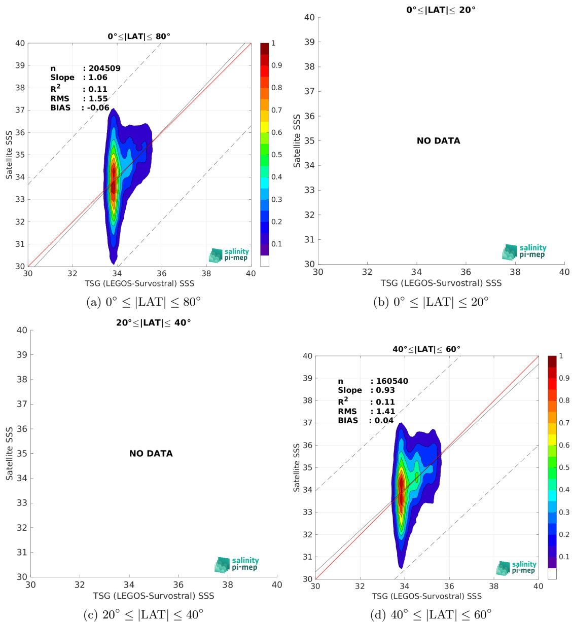
Figure 10: Contour maps of the concentration of SMOS SSS L2Q v333 - 0.25 Deg (CATDS-CPDC) SSS (y-axis) versus TSG (LEGOS-Survostral) SSS (x-axis) at match-up pairs for different latitude bands. For each plot, the red line shows x=y . The black thin and dashed lines indicate a linear fit through the data cloud and the \pm 95\% confidence levels, respectively. The number match-up pairs n , the slope and R^2 coefficient of the linear fit, the root mean square (RMS) and the mean bias between satellite and in situ data are indicated for each latitude band in each plots.
