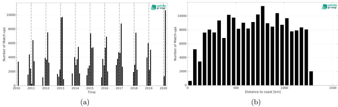
Figure 2: Number of match-ups between TSG (LEGOS-Survostral) and SMOS SSS L2Q v333 - 0.25 Deg (CATDS-CPDC) SSS as a function of time (a) and as function of the distance to coast (b) over the Global Ocean Pi-MEP region and for the full satellite product period.
