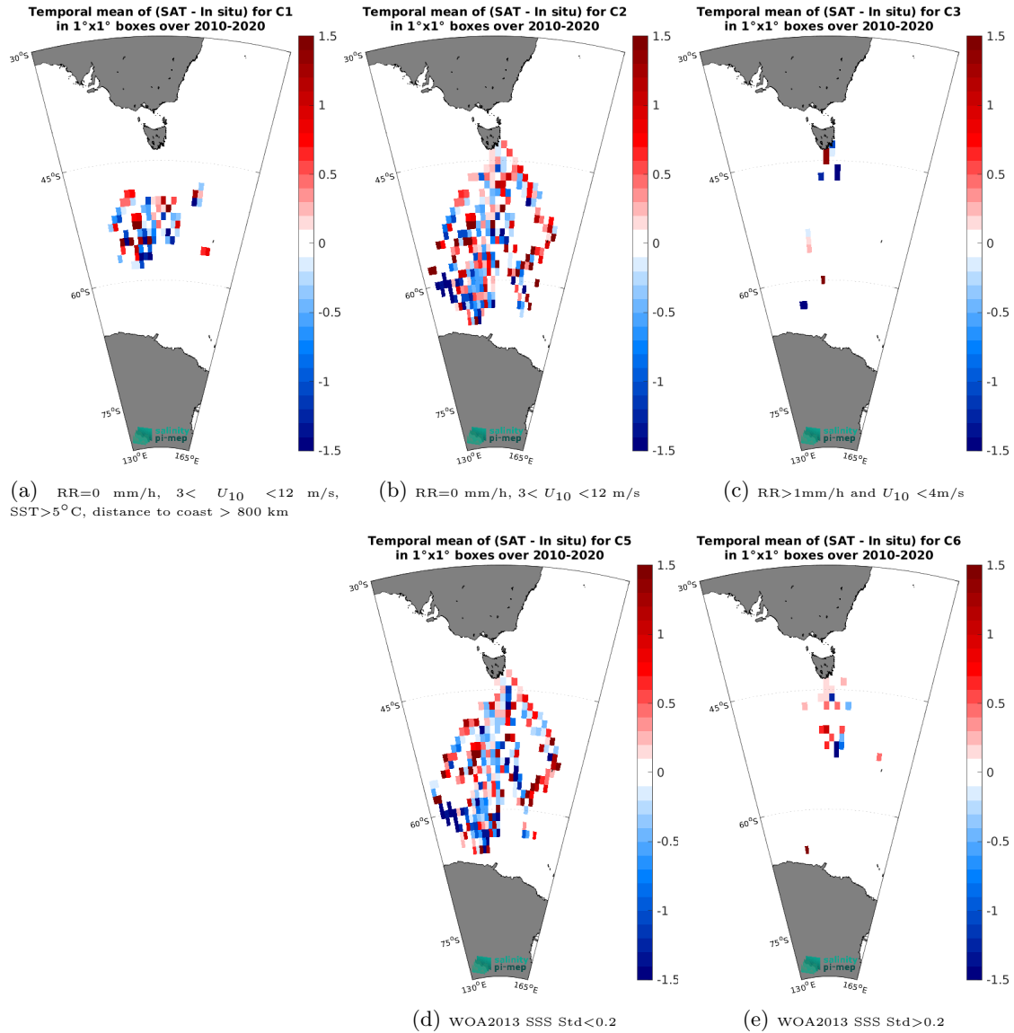
Figure 14: Temporal mean gridded over spatial boxes of size 1^\circ \times 1^\circ of \Delta\text{SSS} (SMOS SSS L2Q v333 - 0.25 Deg (CATDS-CPDC) - TSG (LEGOS-Survostral)) for 5 different subdatasets corresponding to: RR=0 mm/h, 3 < U_{10} < 12 m/s, SST > 5^\circ\text{C} , distance to coast > 800 km (a), RR=0 mm/h, 3 < U_{10} < 12 m/s (b), RR > 1 mm/h and U_{10} < 4 m/s (c), WOA2013 SSS Std < 0.2 (d), WOA2013 SSS Std > 0.2 (e).
