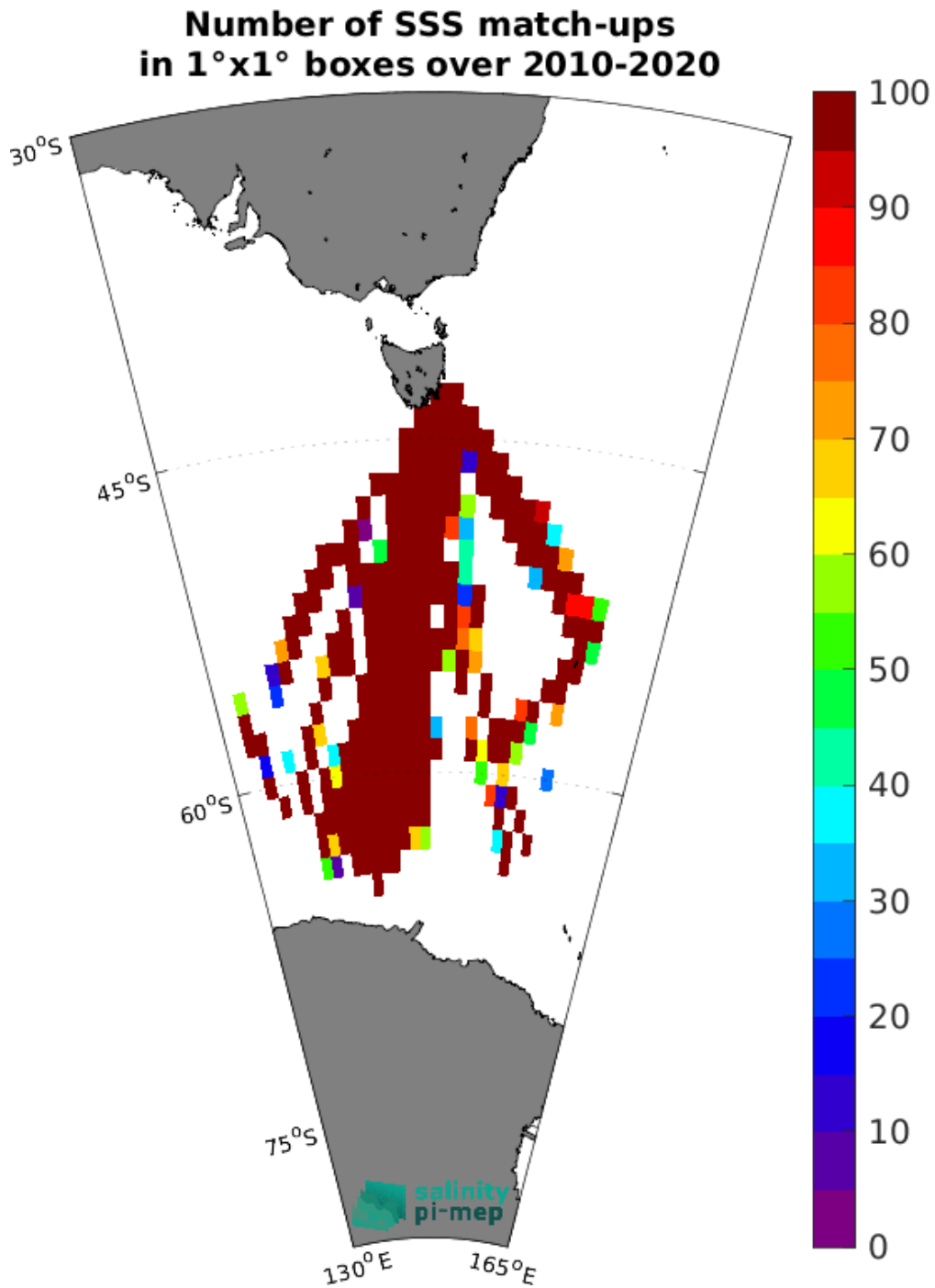
Figure 5: Number of SSS match-ups between TSG (LEGOS-Survostral) SSS and the SMOS SSS L2Q v333 - 0.25 Deg (CATDS-CPDC) SSS product for the Global Ocean Pi-MEP region over 1°x1° boxes and for the full satellite product period.
