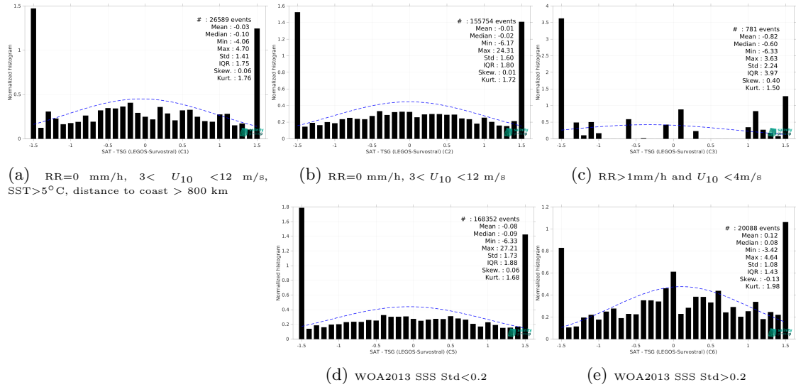
Figure 15: Normalized histogram of \Delta SSS (SMOS SSS L2Q v333 - 0.25 Deg (CATDS-CPDC) - TSG (LEGOS-Survostral)) for 5 different subdatasets corresponding to: RR=0 mm/h, 3 < U_{10} < 12 m/s, SST>5°C, distance to coast > 800 km (a), RR=0 mm/h, 3 < U_{10} < 12 m/s (b), RR>1mm/h and U_{10} < 4 m/s (c), WOA2013 SSS Std<0.2 (d), WOA2013 SSS Std>0.2 (e).
