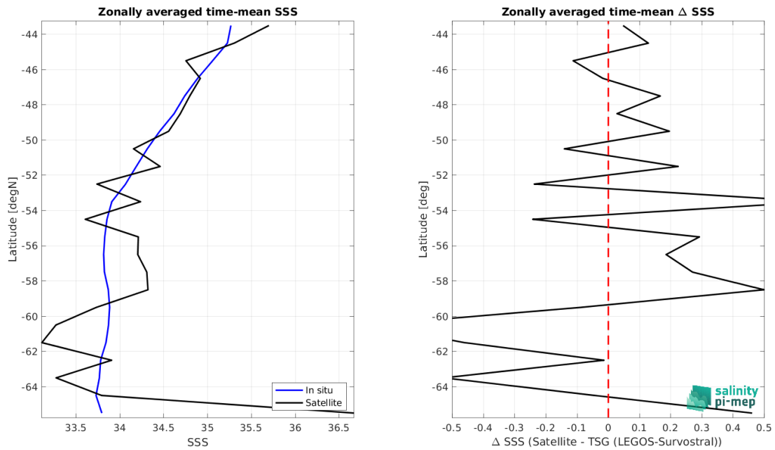
Figure 9: Left panel: Zonal mean SSS from SMOS SSS L2Q v333 - 0.25 Deg (CATDS-CPDC) satellite product (black) and from TSG (LEGOS-Survostral) (blue). Right panel: Zonal mean of \Delta SSS (Satellite - TSG (LEGOS-Survostral)) for all the collected Pi-MEP match-up pairs estimated over the full satellite product period.
