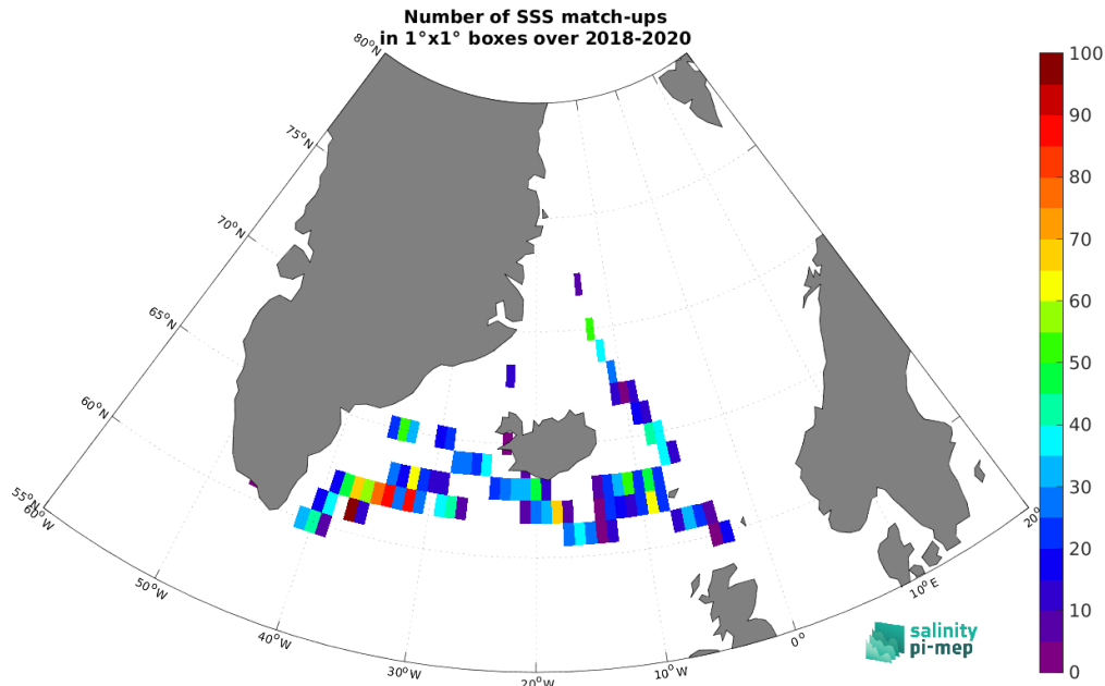
Figure 5: Number of SSS match-ups between TSG (Lauge-Koch) SSS and the SMOS SSS L2Q v333 - 0.25 Deg (CATDS-CPDC) SSS product for the Global Ocean Pi-MEP region over 1^\circ \times 1^\circ boxes and for the full satellite product period.
