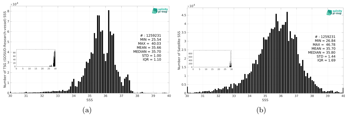
Figure 3: Histograms of SSS from TSG (GOSUD-Research-vessel) (a) and SMOS SSS L2Q v333 - 0.25 Deg (CATDS-CPDC) (b) considering all match-up pairs per bins of 0.1 over the Global Ocean Pi-MEP region and for the full satellite product period.
