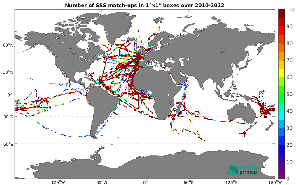
Figure 5: Number of SSS match-ups between TSG (GOSUD-Research-vessel) SSS and the SMOS SSS L2Q v333 - 0.25 Deg (CATDS-CPDC) SSS product for the Global Ocean Pi-MEP region over 1^\circ \times 1^\circ boxes and for the full satellite product period.
