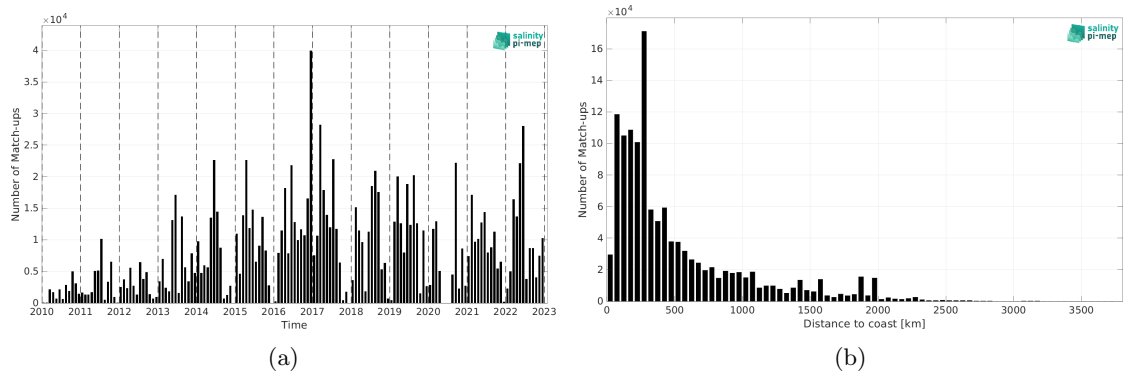
Figure 2: Number of match-ups between TSG (GOSUD-Research-vessel) and SMOS SSS L2Q v333 - 0.25 Deg (CATDS-CPDC) SSS as a function of time (a) and as function of the distance to coast (b) over the Global Ocean Pi-MEP region and for the full satellite product period.
