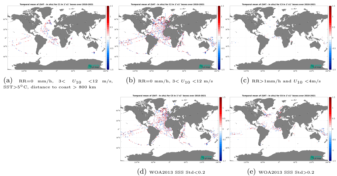
Figure 14: Temporal mean gridded over spatial boxes of size 1^\circ \times 1^\circ of \Delta\text{SSS} (SMOS SSS L2Q v333 - 0.25 Deg (CATDS-CPDC) - TSG (GOSUD-Research-vessel)) for 5 different subdatasets corresponding to:RR=0 mm/h, 3 < U_{10} < 12 m/s, SST > 5^\circ\text{C} , distance to coast > 800 km (a), RR=0 mm/h, 3 < U_{10} < 12 m/s (b), RR > 1 mm/h and U_{10} < 4 m/s (c), WOA2013 SSS Std < 0.2 (d), WOA2013 SSS Std > 0.2 (e).
