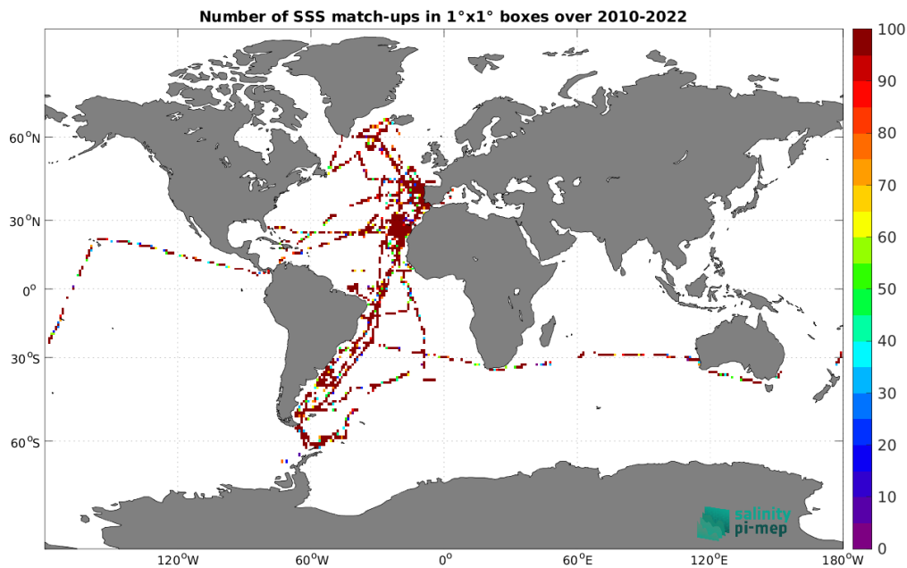
Figure 5: Number of SSS match-ups between TSG (CSIC-UTM) SSS and the SMOS SSS L2Q v333 - 0.25 Deg (CATDS-CPDC) SSS product for the Global Ocean Pi-MEP region over 1^\circ \times 1^\circ boxes and for the full satellite product period.
