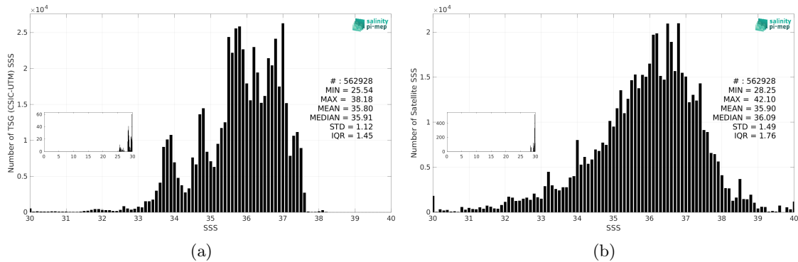
Figure 3: Histograms of SSS from TSG (CSIC-UTM) (a) and SMOS SSS L2Q v333 - 0.25 Deg (CATDS-CPDC) (b) considering all match-up pairs per bins of 0.1 over the Global Ocean Pi-MEP region and for the full satellite product period.
