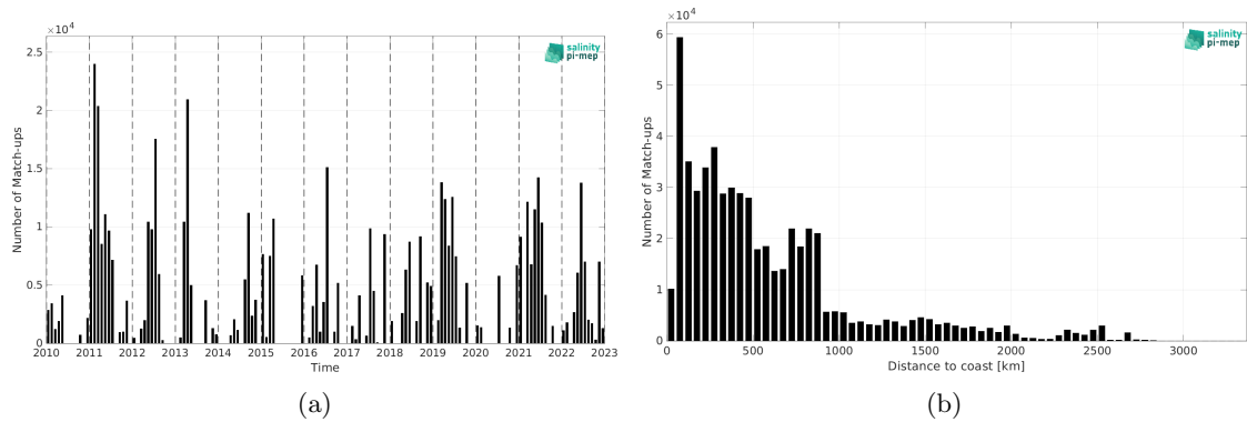
Figure 2: Number of match-ups between TSG (CSIC-UTM) and SMOS SSS L2Q v333 - 0.25 Deg (CATDS-CPDC) SSS as a function of time (a) and as function of the distance to coast (b) over the Global Ocean Pi-MEP region and for the full satellite product period.
