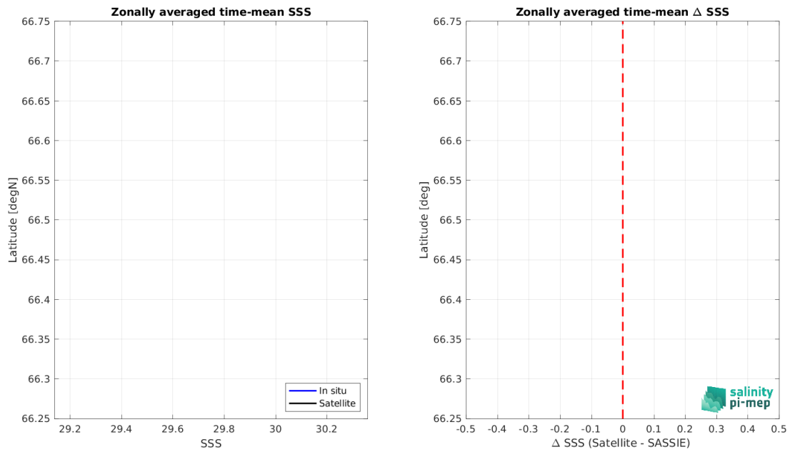
Figure 9: Left panel: Zonal mean SSS from SMOS SSS L2Q v333 - 0.25 Deg (CATDS-CPDC) satellite product (black) and from SASSIE (blue). Right panel: Zonal mean of \Delta SSS (Satellite - SASSIE) for all the collected Pi-MEP match-up pairs estimated over the full satellite product period.
