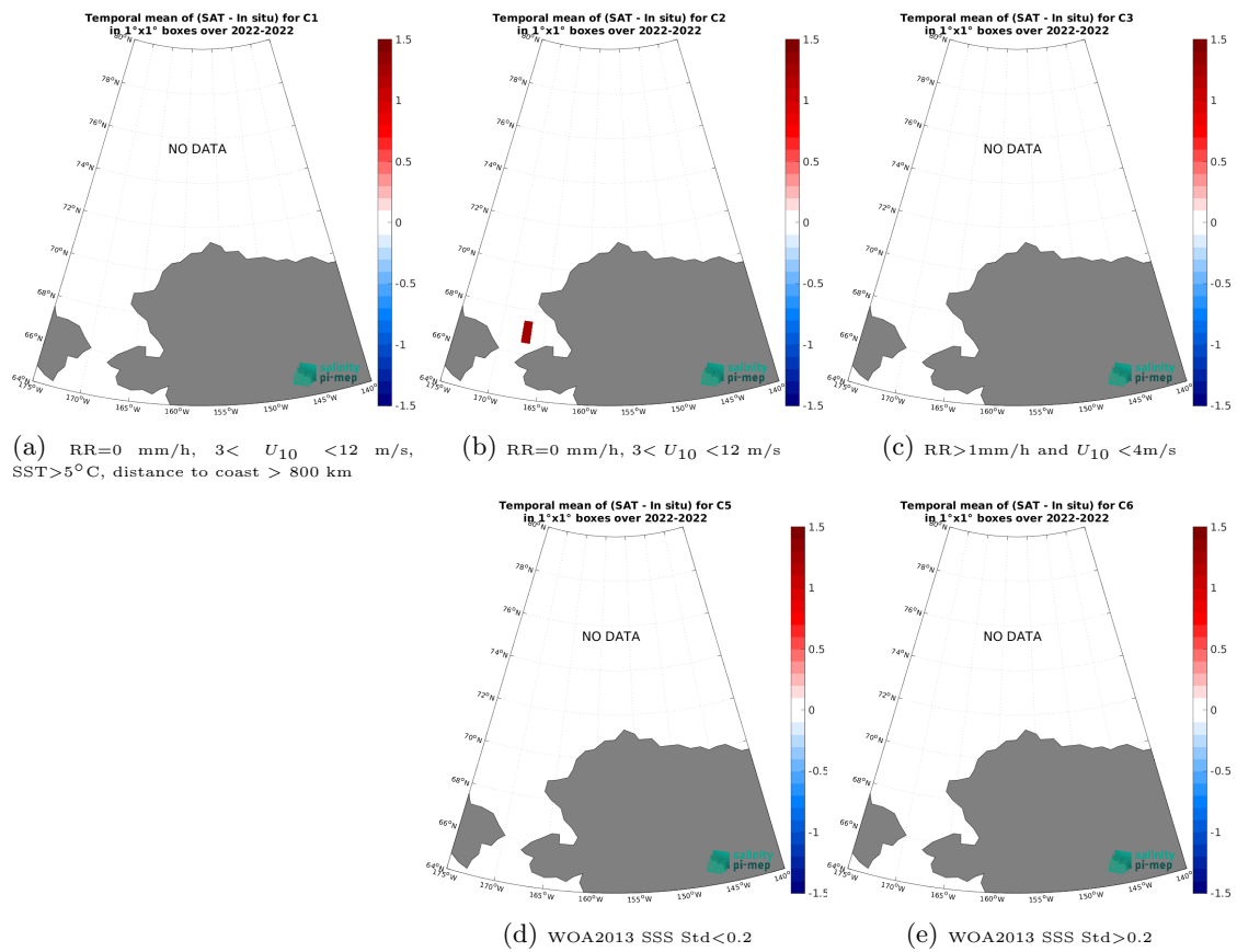
Figure 14: Temporal mean gridded over spatial boxes of size 1^\circ \times 1^\circ of \Delta SSS (SMOS SSS L2Q v333 - 0.25 Deg (CATDS-CPDC) - SASSIE) for 5 different subdatasets corresponding to:RR=0 mm/h, 3 < U_{10} < 12 m/s, SST>5°C, distance to coast > 800 km (a), RR=0 mm/h, 3 < U_{10} < 12 m/s (b), RR>1mm/h and U_{10} < 4 m/s (c), WOA2013 SSS Std<0.2 (d), WOA2013 SSS Std>0.2 (e).
