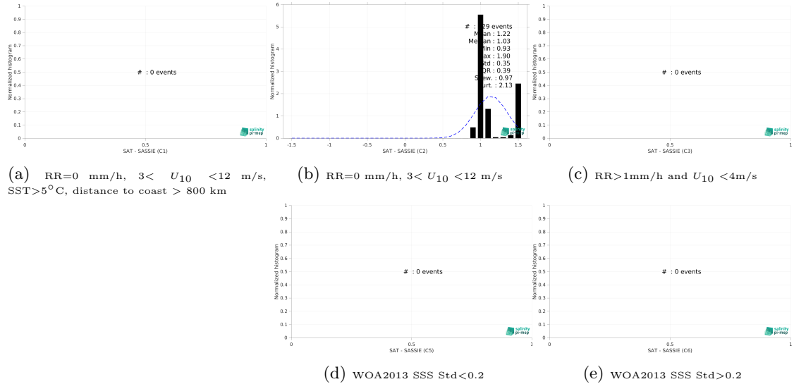
Figure 15: Normalized histogram of \Delta SSS (SMOS SSS L2Q v333 - 0.25 Deg (CATDS-CPDC) - SASSIE) for 5 different subdatasets corresponding to: RR=0 mm/h, 3 < U_{10} < 12 m/s, SST > 5°C, distance to coast > 800 km (a), RR=0 mm/h, 3 < U_{10} < 12 m/s (b), RR > 1mm/h and U_{10} < 4 m/s (c), WOA2013 SSS Std < 0.2 (d), WOA2013 SSS Std > 0.2 (e).
