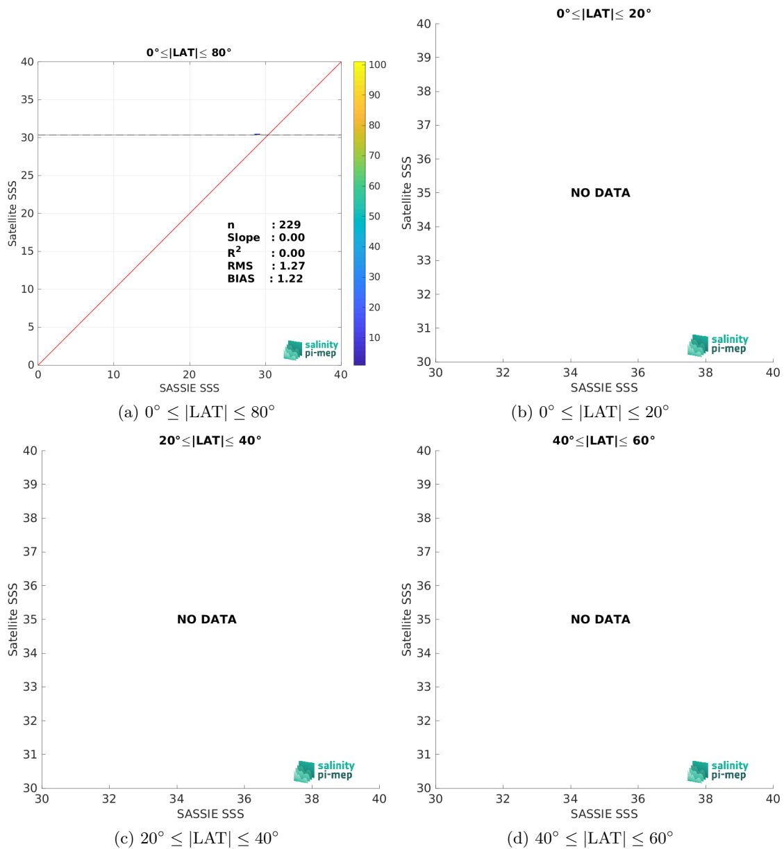
Figure 10: Contour maps of the concentration of SMOS SSS L2Q v333 - 0.25 Deg (CATDS-CPDC) SSS (y-axis) versus SASSIE SSS (x-axis) at match-up pairs for different latitude bands. For each plot, the red line shows x=y . The black thin and dashed lines indicate a linear fit through the data cloud and the \pm 95\% confidence levels, respectively. The number match-up pairs n , the slope and R^2 coefficient of the linear fit, the root mean square (RMS) and the mean bias between satellite and in situ data are indicated for each latitude band in each plots.
