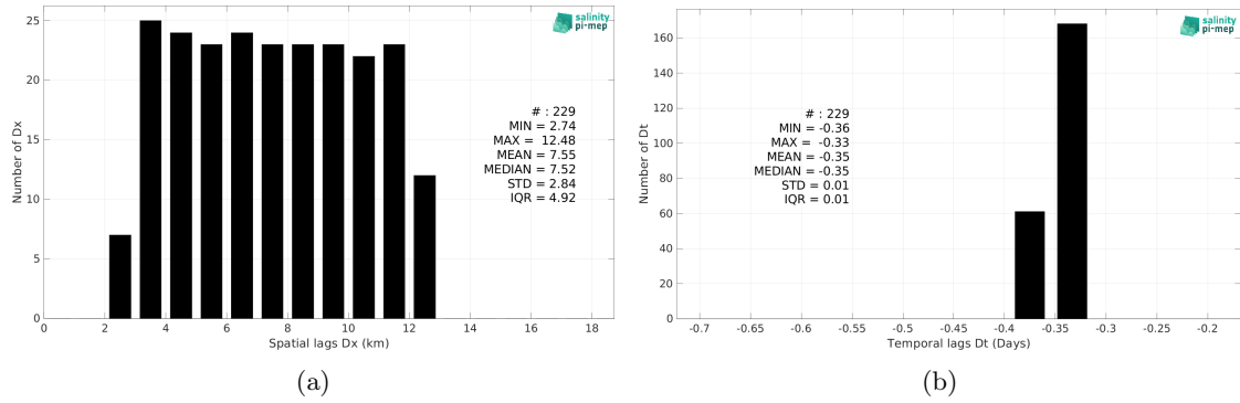
Figure 6: Histograms of the spatial (a) and temporal (b) lags between the location/time of the SASSIE measurement and the date of the corresponding SMOS SSS L2Q v333 - 0.25 Deg (CATDS-CPDC) SSS pixel.
