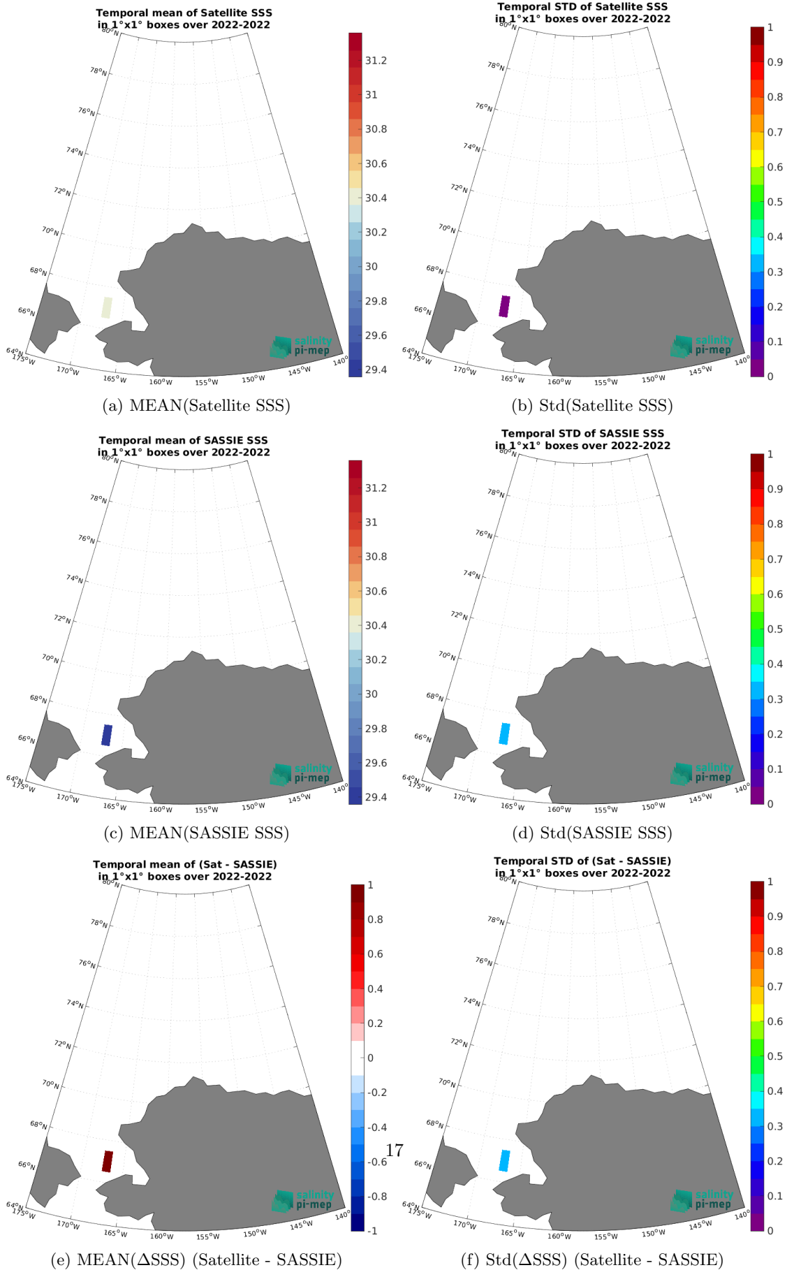
Figure 7: Temporal mean (left) and Std (right) of SSS from SMOS SSS L2Q v333 - 0.25 Deg (CATDS-CPDC) (top), SASSIE (middle), and of \Delta SSS (Satellite - SASSIE). Only match-up pairs are used to generate these maps.
