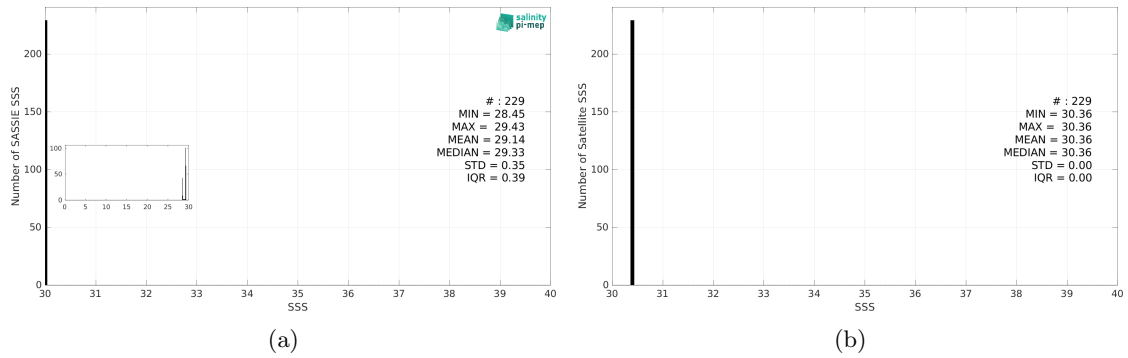
Figure 3: Histograms of SSS from SASSIE (a) and SMOS SSS L2Q v333 - 0.25 Deg (CATDS-CPDC) (b) considering all match-up pairs per bins of 0.1 over the Global Ocean Pi-MEP region and for the full satellite product period.
