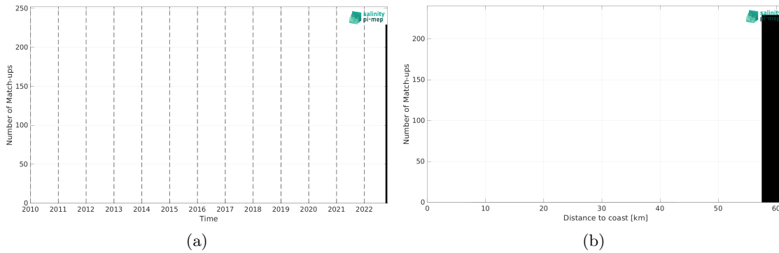
Figure 2: Number of match-ups between SASSIE and SMOS SSS L2Q v333 - 0.25 Deg (CATDS-CPDC) SSS as a function of time (a) and as function of the distance to coast (b) over the Global Ocean Pi-MEP region and for the full satellite product period.
