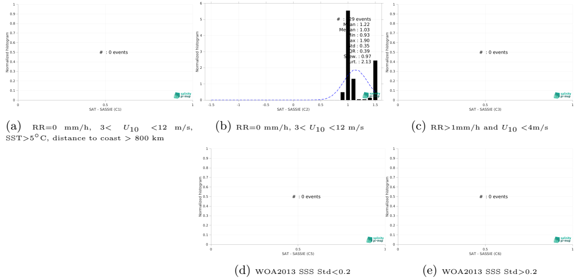
Figure 15: Normalized histogram of \Delta SSS (SMOS SSS L2Q v333 - 0.25 Deg (CATDS-CPDC) - SASSIE) for 5 different subdatasets corresponding to: RR=0 mm/h, 3 < U_{10} < 12 m/s, SST>5°C, distance to coast > 800 km (a), RR=0 mm/h, 3 < U_{10} < 12 m/s (b), RR>1mm/h and U_{10} < 4 m/s (c), WOA2013 SSS Std<0.2 (d), WOA2013 SSS Std>0.2 (e).
