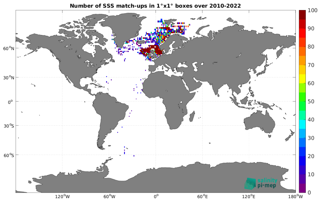
Figure 5: Number of SSS match-ups between ICES SSS and the SMOS SSS L2Q v333 - 0.25 Deg (CATDS-CPDC) SSS product for the Global Ocean Pi-MEP region over 1^\circ \times 1^\circ boxes and for the full satellite product period.
