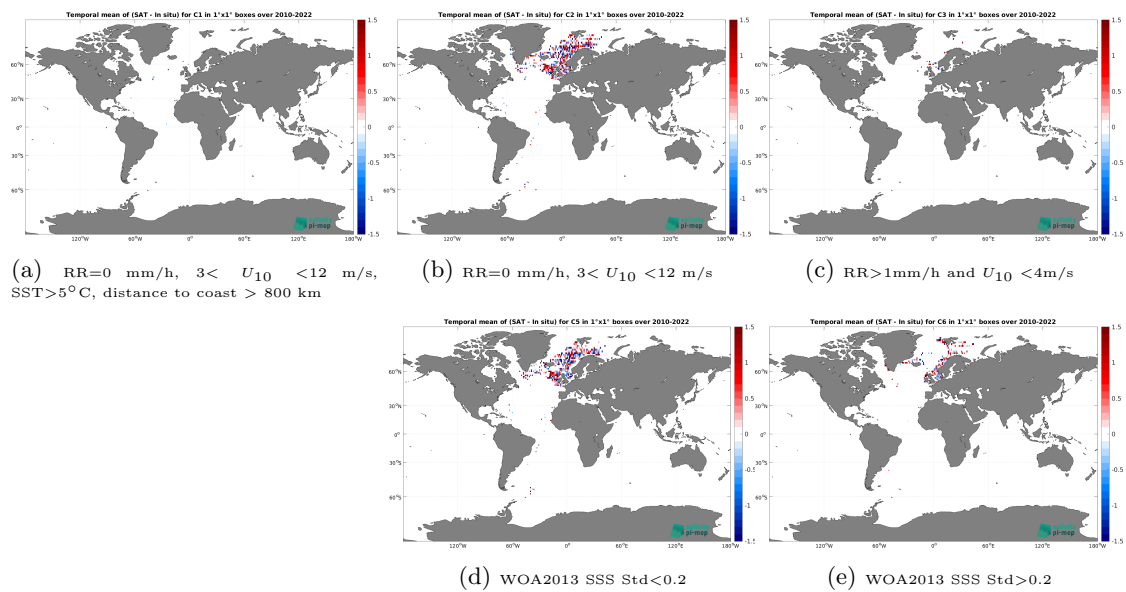
Figure 14: Temporal mean gridded over spatial boxes of size 1^\circ \times 1^\circ of \Delta SSS (SMOS SSS L2Q v333 - 0.25 Deg (CATDS-CPDC) - ICES) for 5 different subdatasets corresponding to:RR=0 mm/h, 3 < U_{10} < 12 m/s, SST > 5^\circ\text{C} , distance to coast > 800 km (a), RR=0 mm/h, 3 < U_{10} < 12 m/s (b), RR > 1 mm/h and U_{10} < 4 m/s (c), WOA2013 SSS Std < 0.2 (d), WOA2013 SSS Std > 0.2 (e).
