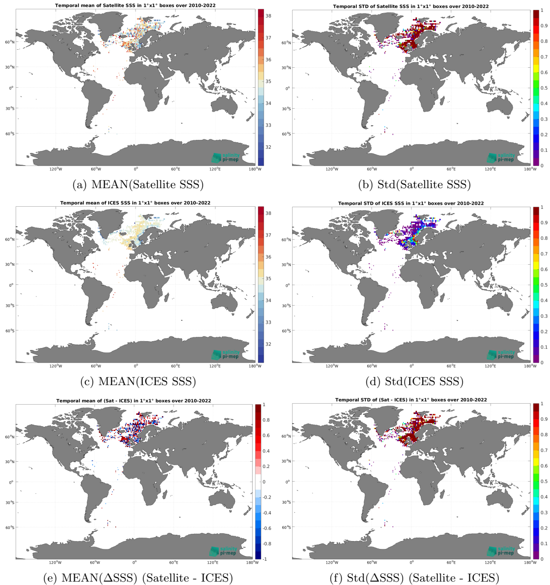
Figure 7: Temporal mean (left) and Std (right) of SSS from SMOS SSS L2Q v333 - 0.25 Deg (CATDS-CPDC) (top), ICES (middle), and of \Delta SSS (Satellite - ICES). Only match-up pairs are used to generate these maps.
