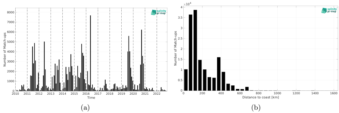
Figure 2: Number of match-ups between ICES and SMOS SSS L2Q v333 - 0.25 Deg (CATDS-CPDC) SSS as a function of time (a) and as function of the distance to coast (b) over the Global Ocean Pi-MEP region and for the full satellite product period.
