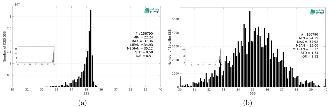
Figure 3: Histograms of SSS from ICES (a) and SMOS SSS L2Q v333 - 0.25 Deg (CATDS-CPDC) (b) considering all match-up pairs per bins of 0.1 over the Global Ocean Pi-MEP region and for the full satellite product period.
