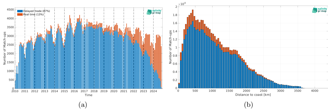
Figure 2: Number of match-ups between Argo and SMOS SSS L2Q v333 - 0.25 Deg (CATDS-CPDC) SSS as a function of time (a) and as function of the distance to coast (b) over the Global Ocean Pi-MEP region and for the full satellite product period.
