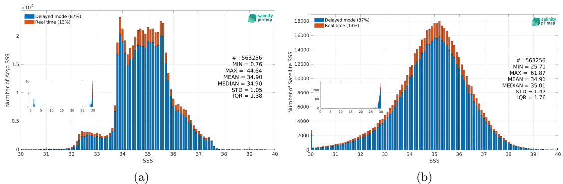
Figure 3: Histograms of SSS from Argo (a) and SMOS SSS L2Q v333 - 0.25 Deg (CATDS-CPDC) (b) considering all match-up pairs per bins of 0.1 over the Global Ocean Pi-MEP region and for the full satellite product period.
