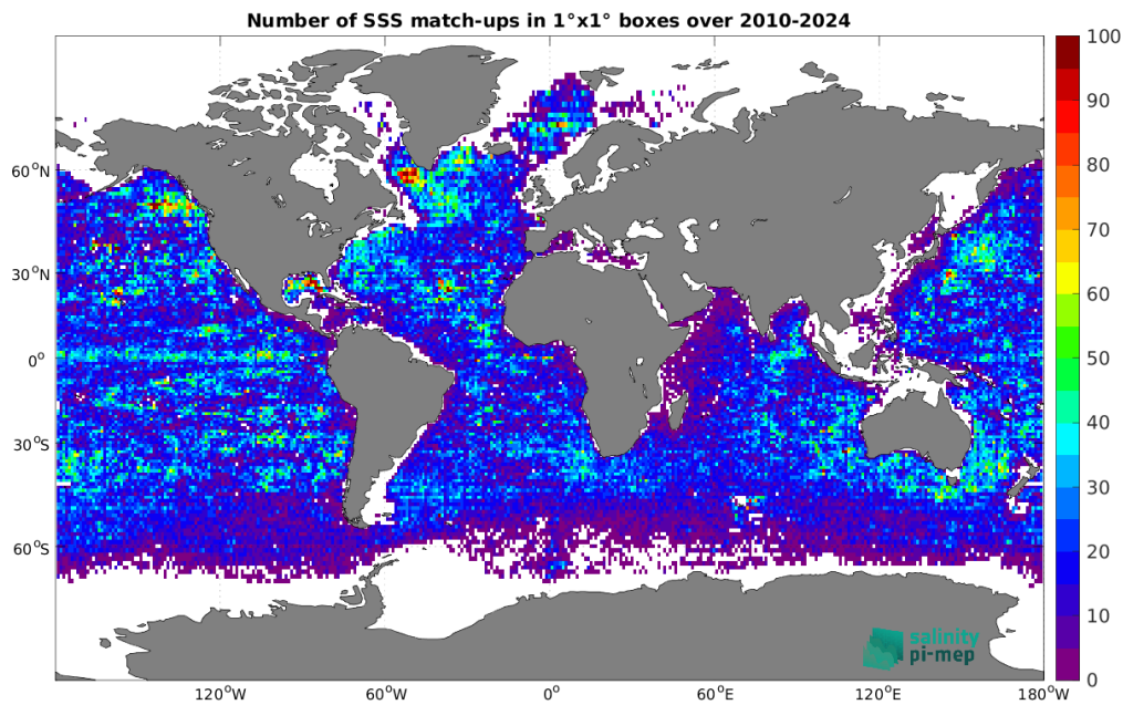
Figure 5: Number of SSS match-ups between Argo SSS and the SMOS SSS L2Q v333 - 0.25 Deg (CATDS-CPDC) SSS product for the Global Ocean Pi-MEP region over 1^\circ \times 1^\circ boxes and for the full satellite product period.
