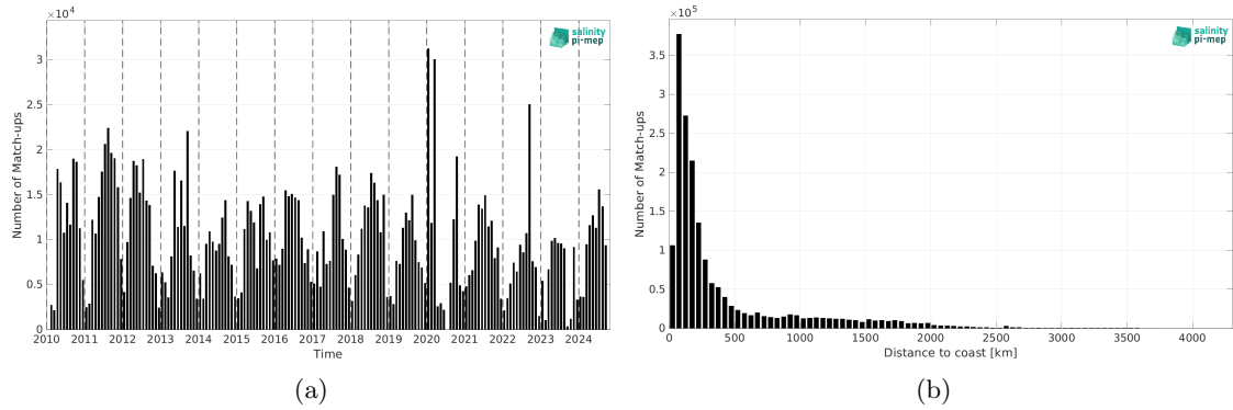
Figure 2: Number of match-ups between TSG (SAMOS) and SMOS SSS L3 v332 - 9 Days (CATDS-CPDC) SSS as a function of time (a) and as function of the distance to coast (b) over the Global Ocean Pi-MEP region and for the full satellite product period.
