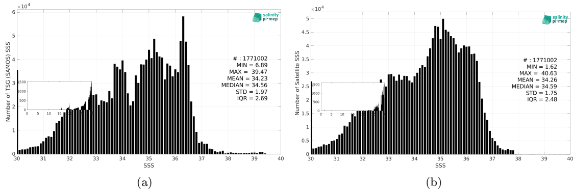
Figure 3: Histograms of SSS from TSG (SAMOS) (a) and SMOS SSS L3 v332 - 9 Days (CATDS-CPDC) (b) considering all match-up pairs per bins of 0.1 over the Global Ocean Pi-MEP region and for the full satellite product period.
