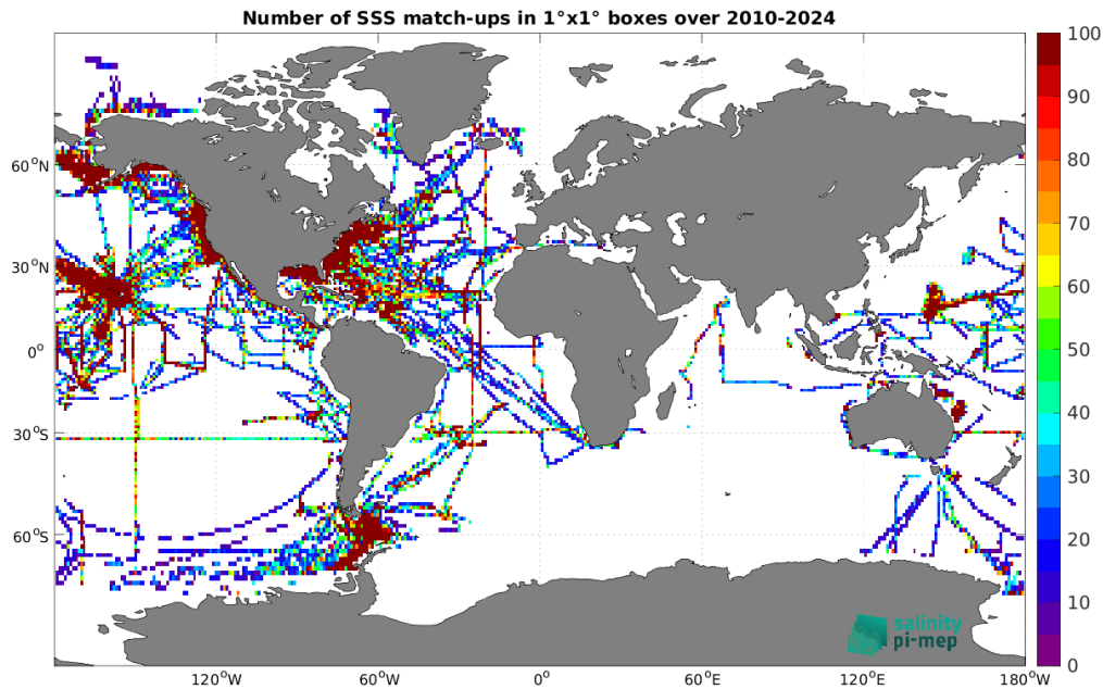
Figure 5: Number of SSS match-ups between TSG (SAMOS) SSS and the SMOS SSS L3 v332 - 9 Days (CATDS-CPDC) SSS product for the Global Ocean Pi-MEP region over 1^\circ \times 1^\circ boxes and for the full satellite product period.
