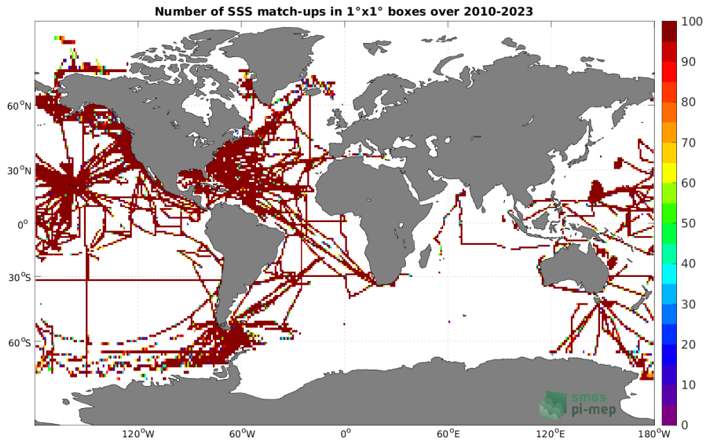
Figure 4: Number of SSS match-ups between TSG (SAMOS) SSS and the SMOS SSS L3 v332 - 9 Days (CATDS-CPDC) SSS product for the Global Ocean Pi-MEP region over 1^\circ \times 1^\circ boxes and for the full satellite product period.
