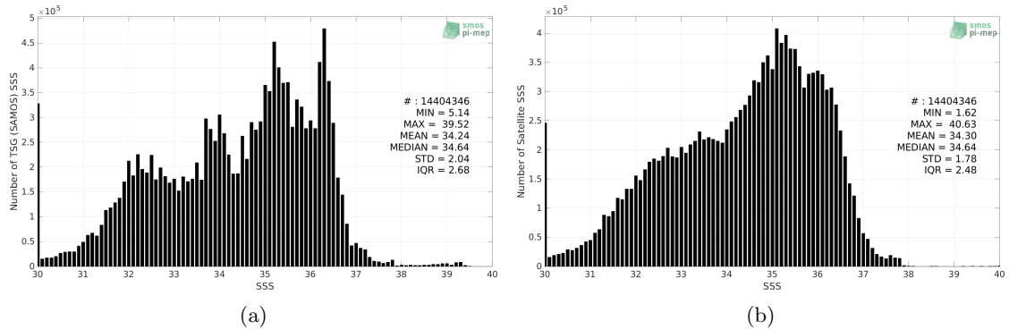
Figure 2: Histograms of SSS from TSG (SAMOS) (a) and SMOS SSS L3 v332 - 9 Days (CATDS-CPDC) (b) considering all match-up pairs per bins of 0.1 over the Global Ocean Pi-MEP region and for the full satellite product period.
