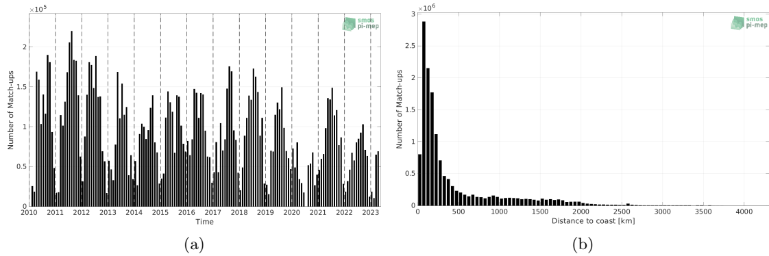
Figure 1: Number of match-ups between TSG (SAMOS) and SMOS SSS L3 v332 - 9 Days (CATDS-CPDC) SSS as a function of time (a) and as function of the distance to coast (b) over the Global Ocean Pi-MEP region and for the full satellite product period.
