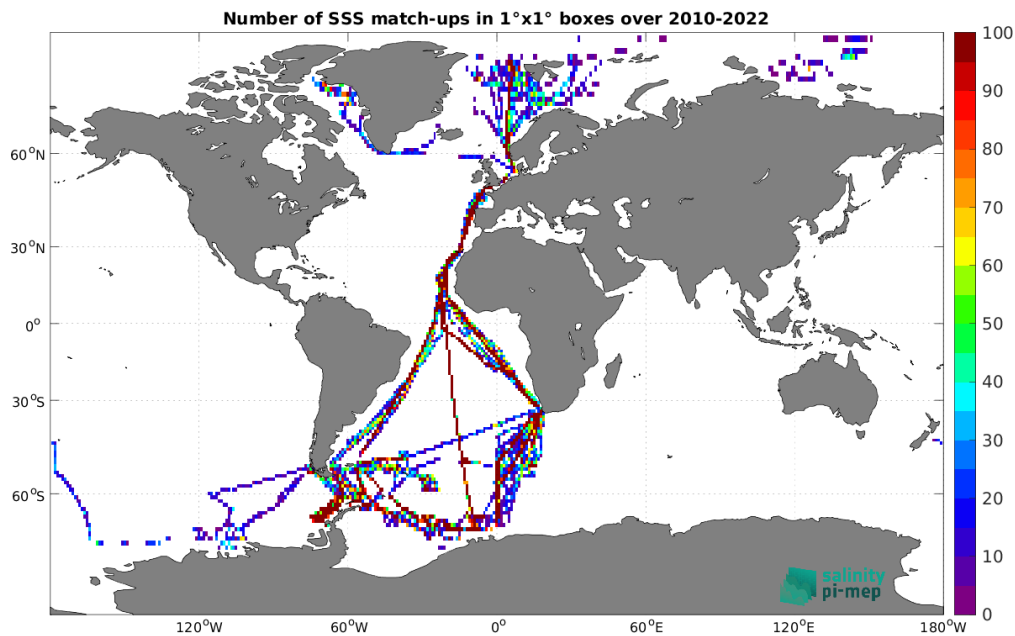
Figure 4: Number of SSS match-ups between TSG (Polarstern) SSS and the SMOS SSS L3 v332 - 9 Days (CATDS-CPDC) SSS product for the Global Ocean Pi-MEP region over 1^\circ \times 1^\circ boxes and for the full satellite product period.
