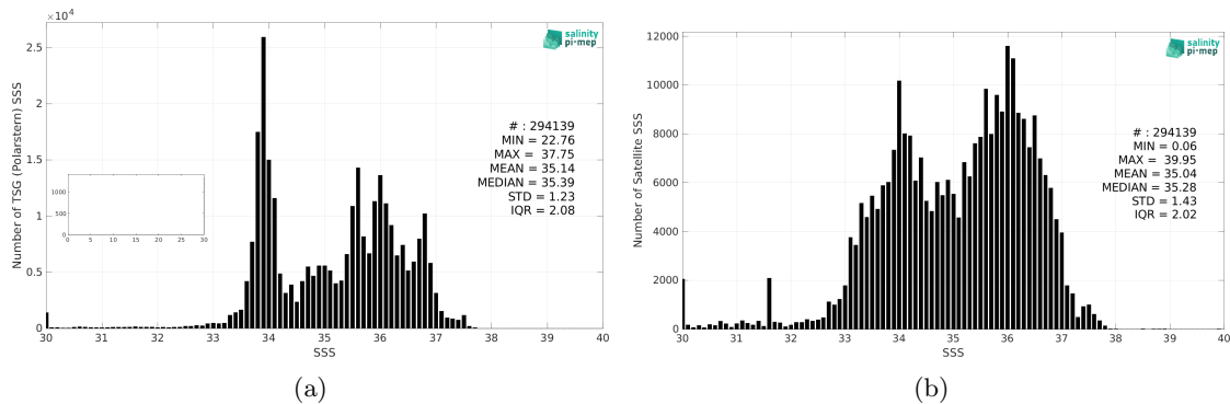
Figure 2: Histograms of SSS from TSG (Polarstern) (a) and SMOS SSS L3 v332 - 9 Days (CATDS-CPDC) (b) considering all match-up pairs per bins of 0.1 over the Global Ocean Pi-MEP region and for the full satellite product period.
