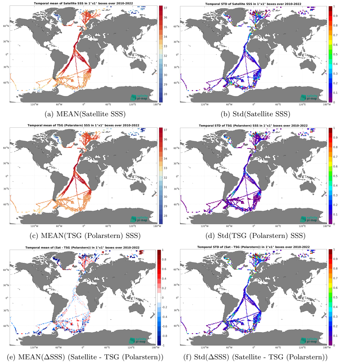
Figure 6: Temporal mean (left) and Std (right) of SSS from SMOS SSS L3 v332 - 9 Days (CATDS-CPDC) (top), TSG (Polarstern) (middle), and of \Delta SSS (Satellite - TSG (Polarstern)). Only match-up pairs are used to generate these maps.
