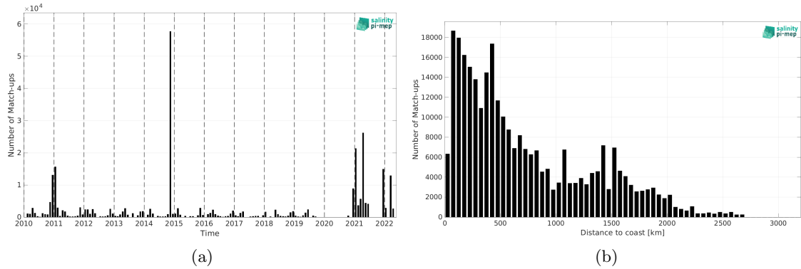
Figure 1: Number of match-ups between TSG (Polarstern) and SMOS SSS L3 v332 - 9 Days (CATDS-CPDC) SSS as a function of time (a) and as function of the distance to coast (b) over the Global Ocean Pi-MEP region and for the full satellite product period.
