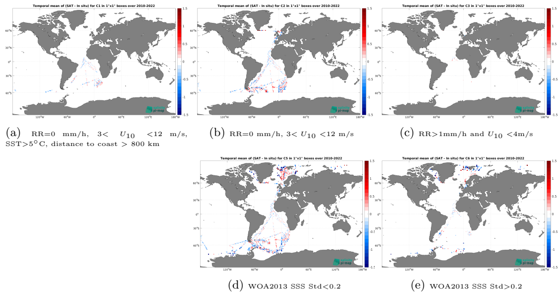
Figure 12: Temporal mean gridded over spatial boxes of size 1^\circ \times 1^\circ of \Delta SSS (SMOS SSS L3 v332 - 9 Days (CATDS-CPDC) - TSG (Polarstern)) for 5 different subdatasets corresponding to:RR=0 mm/h, 3 < U_{10} < 12 m/s, SST > 5^\circ\text{C} , distance to coast > 800 km (a), RR=0 mm/h, 3 < U_{10} < 12 m/s (b), RR > 1 mm/h and U_{10} < 4 m/s (c), WOA2013 SSS Std < 0.2 (d), WOA2013 SSS Std > 0.2 (e).
