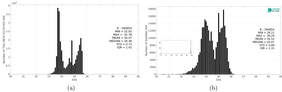
Figure 3: Histograms of SSS from TSG (NCEI-0170743) (a) and SMOS SSS L3 v332 - 9 Days (CATDS-CPDC) (b) considering all match-up pairs per bins of 0.1 over the Global Ocean Pi-MEP region and for the full satellite product period.
