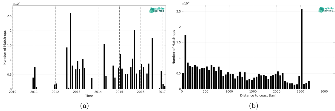
Figure 2: Number of match-ups between TSG (NCEI-0170743) and SMOS SSS L3 v332 - 9 Days (CATDS-CPDC) SSS as a function of time (a) and as function of the distance to coast (b) over the Global Ocean Pi-MEP region and for the full satellite product period.
