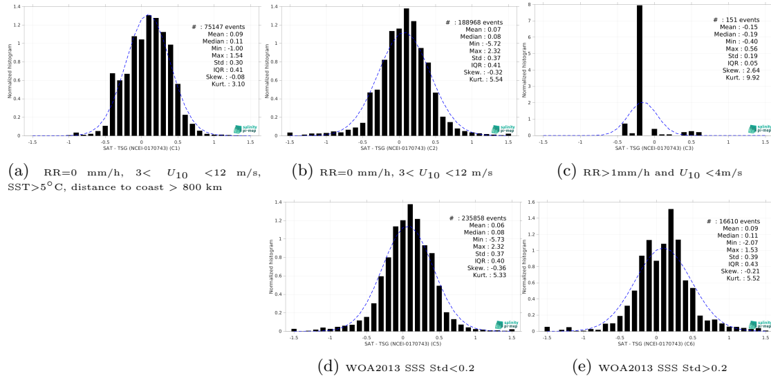
Figure 15: Normalized histogram of \Delta SSS (SMOS SSS L3 v332 - 9 Days (CATDS-CPDC) - TSG (NCEI-0170743)) for 5 different subdatasets corresponding to: RR=0 mm/h, 3 < U_{10} < 12 m/s, SST>5°C, distance to coast > 800 km (a), RR=0 mm/h, 3 < U_{10} < 12 m/s (b), RR>1mm/h and U_{10} < 4 m/s (c), WOA2013 SSS Std<0.2 (d), WOA2013 SSS Std>0.2 (e).
