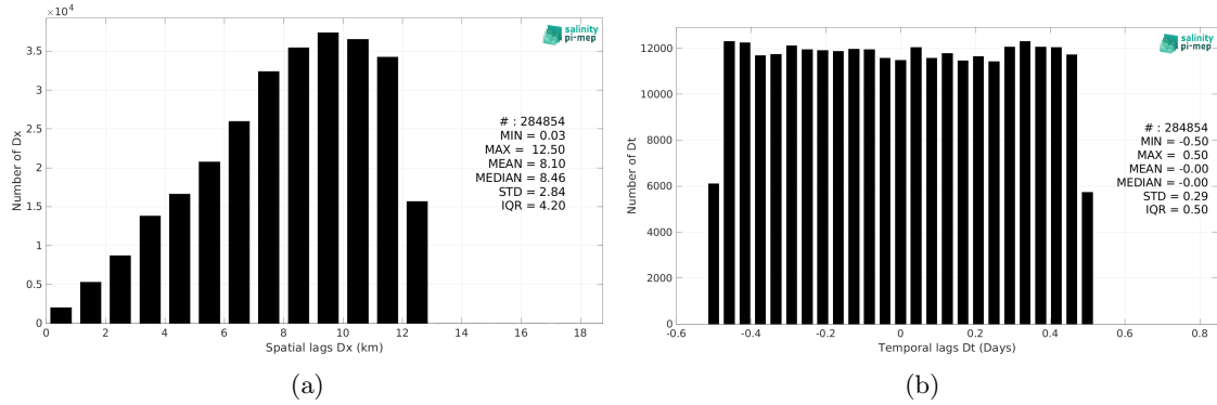
Figure 6: Histograms of the spatial (a) and temporal (b) lags between the location/time of the TSG (NCEI-0170743) measurement and the date of the corresponding SMOS SSS L3 v332 - 9 Days (CATDS-CPDC) SSS pixel.
