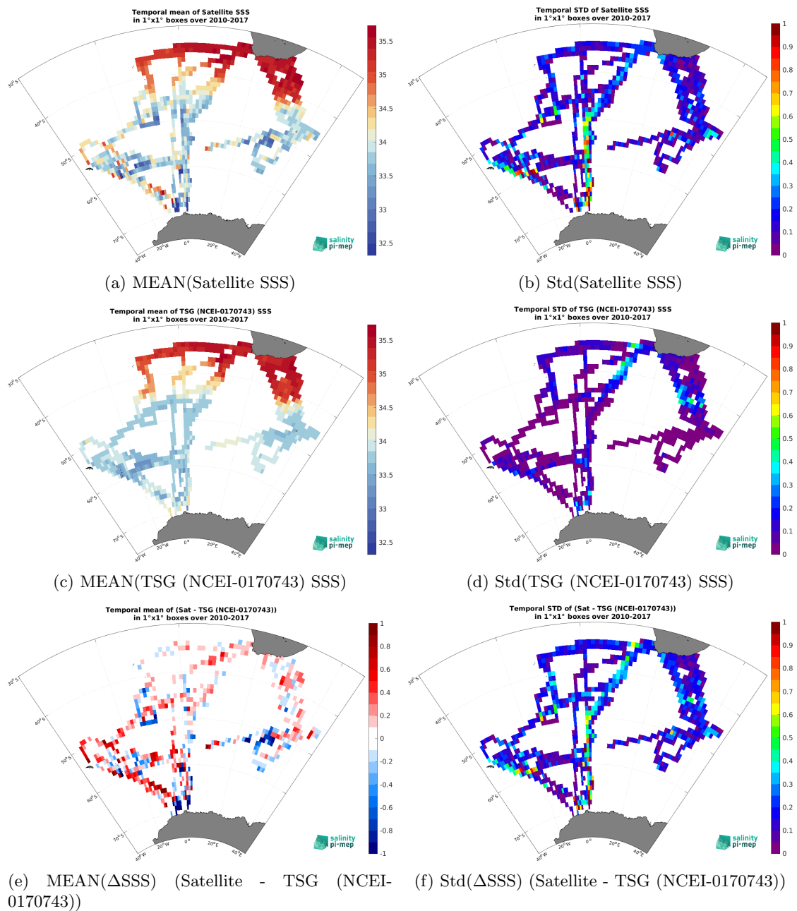
Figure 7: Temporal mean (left) and Std (right) of SSS from SMOS SSS L3 v332 - 9 Days (CATDS-CPDC) (top), TSG (NCEI-0170743) (middle), and of \Delta SSS (Satellite - TSG (NCEI-0170743)). Only match-up pairs are used to generate these maps.
