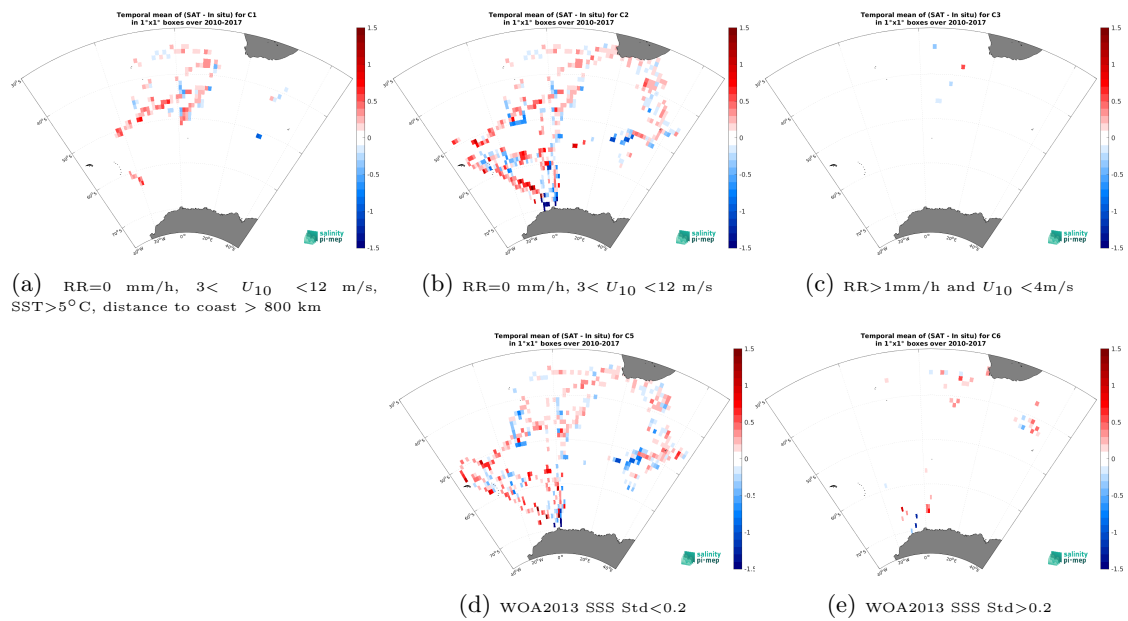
Figure 14: Temporal mean gridded over spatial boxes of size 1^\circ \times 1^\circ of \Delta SSS (SMOS SSS L3 v332 - 9 Days (CATDS-CPDC) - TSG (NCEI-0170743)) for 5 different subdatasets corresponding to: RR=0 mm/h, 3 < U_{10} < 12 m/s, SST > 5^\circ\text{C} , distance to coast > 800 km (a), RR=0 mm/h, 3 < U_{10} < 12 m/s (b), RR > 1 mm/h and U_{10} < 4 m/s (c), WOA2013 SSS Std < 0.2 (d), WOA2013 SSS Std > 0.2 (e).
