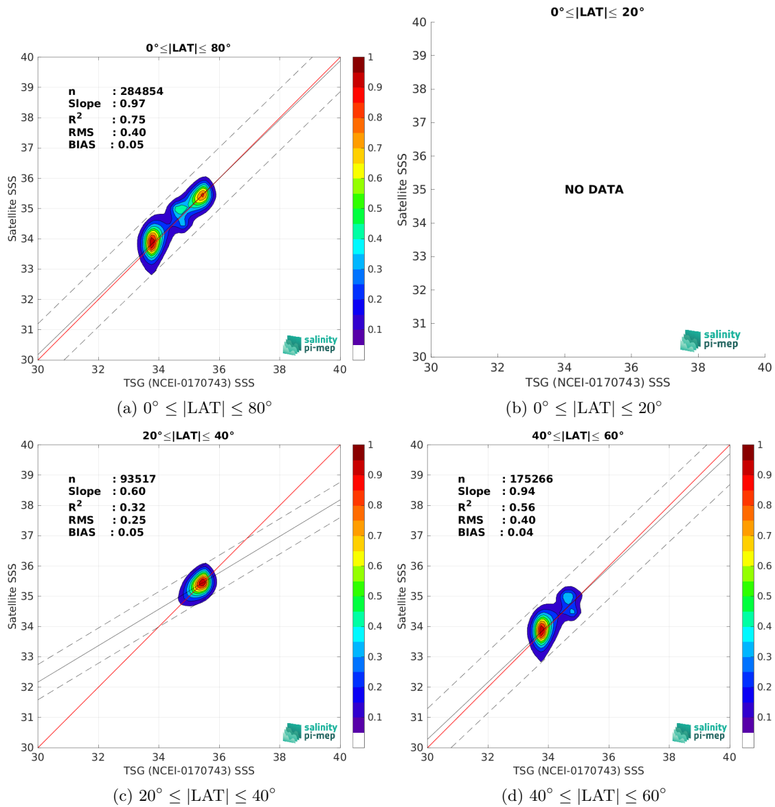
Figure 10: Contour maps of the concentration of SMOS SSS L3 v332 - 9 Days (CATDS-CPDC) SSS (y-axis) versus TSG (NCEI-0170743) SSS (x-axis) at match-up pairs for different latitude bands. For each plot, the red line shows x=y . The black thin and dashed lines indicate a linear fit through the data cloud and the \pm 95\% confidence levels, respectively. The number match-up pairs n , the slope and R^2 coefficient of the linear fit, the root mean square (RMS) and the mean bias between satellite and in situ data are indicated for each latitude band in each plots.
