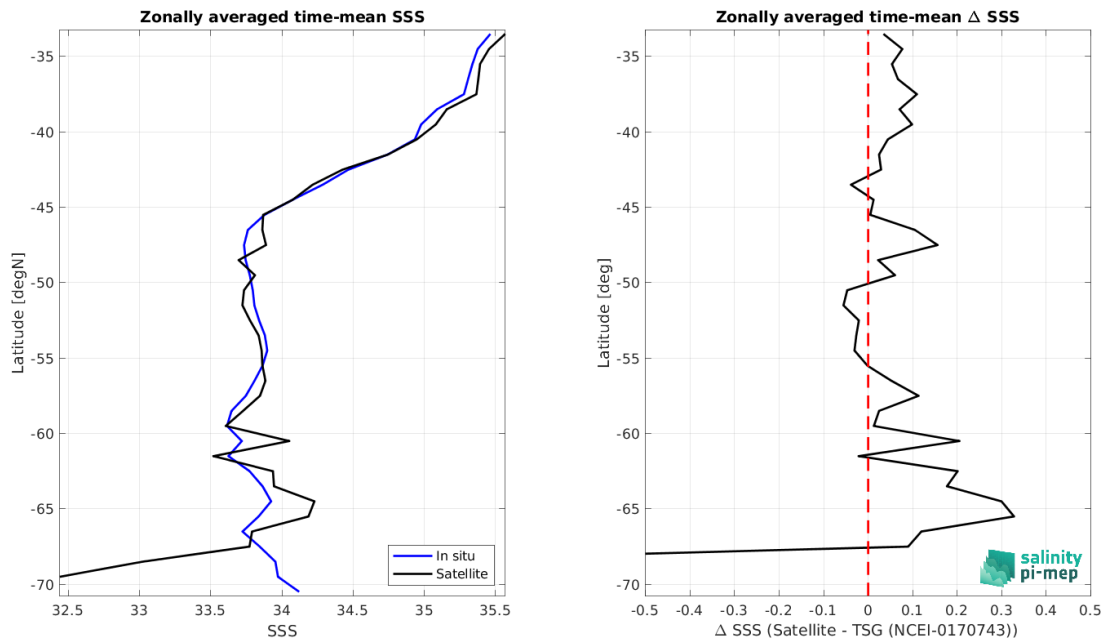
Figure 9: Left panel: Zonal mean SSS from SMOS SSS L3 v332 - 9 Days (CATDS-CPDC) satellite product (black) and from TSG (NCEI-0170743) (blue). Right panel: Zonal mean of \Delta SSS (Satellite - TSG (NCEI-0170743)) for all the collected Pi-MEP match-up pairs estimated over the full satellite product period.
