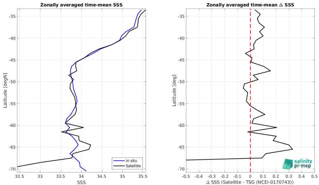
Figure 8: Left panel: Zonal mean SSS from SMOS SSS L3 v332 - 9 Days (CATDS-CPDC) satellite product (black) and from TSG (NCEI-0170743) (blue). Right panel: Zonal mean of \Delta SSS (Satellite - TSG (NCEI-0170743)) for all the collected Pi-MEP match-up pairs estimated over the full satellite product period.
