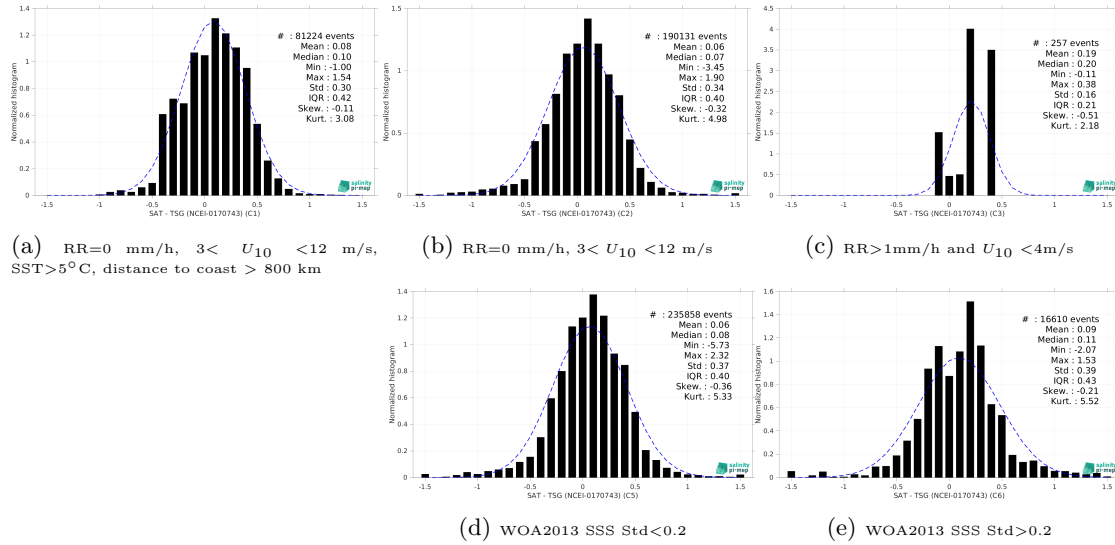
Figure 13: Normalized histogram of \Delta SSS (SMOS SSS L3 v332 - 9 Days (CATDS-CPDC) - TSG (NCEI-0170743)) for 5 different subdatasets corresponding to: RR=0 mm/h, 3 < U_{10} < 12 m/s, SST > 5°C, distance to coast > 800 km (a), RR=0 mm/h, 3 < U_{10} < 12 m/s (b), RR > 1mm/h and U_{10} < 4 m/s (c), WOA2013 SSS Std < 0.2 (d), WOA2013 SSS Std > 0.2 (e).
