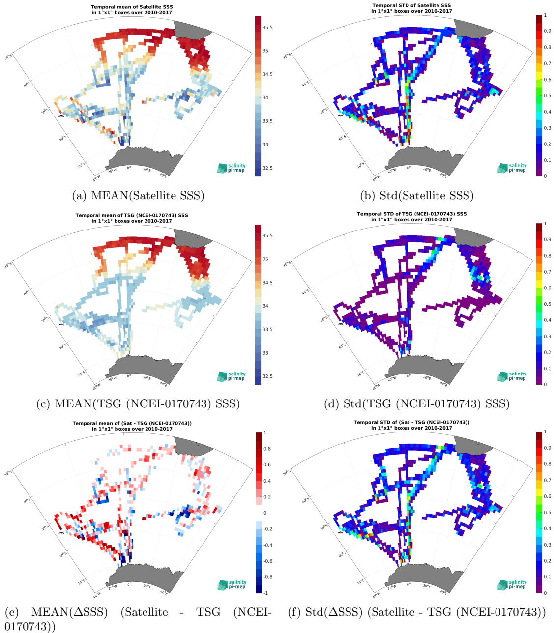
Figure 6: Temporal mean (left) and Std (right) of SSS from SMOS SSS L3 v332 - 9 Days (CATDS-CPDC) (top), TSG (NCEI-0170743) (middle), and of \Delta SSS (Satellite - TSG (NCEI-0170743)). Only match-up pairs are used to generate these maps.
