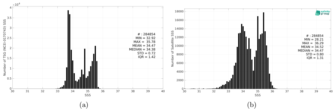
Figure 2: Histograms of SSS from TSG (NCEI-0170743) (a) and SMOS SSS L3 v332 - 9 Days (CATDS-CPDC) (b) considering all match-up pairs per bins of 0.1 over the Global Ocean Pi-MEP region and for the full satellite product period.
