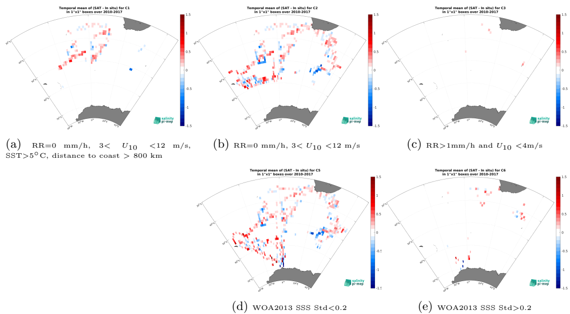
Figure 12: Temporal mean gridded over spatial boxes of size 1^\circ \times 1^\circ of \Delta SSS (SMOS SSS L3 v332 - 9 Days (CATDS-CPDC) - TSG (NCEI-0170743)) for 5 different subdatasets corresponding to:RR=0 mm/h, 3 < U_{10} < 12 m/s, SST > 5^\circ\text{C} , distance to coast > 800 km (a), RR=0 mm/h, 3 < U_{10} < 12 m/s (b), RR > 1 mm/h and U_{10} < 4 m/s (c), WOA2013 SSS Std < 0.2 (d), WOA2013 SSS Std > 0.2 (e).
