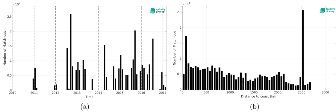
Figure 1: Number of match-ups between TSG (NCEI-0170743) and SMOS SSS L3 v332 - 9 Days (CATDS-CPDC) SSS as a function of time (a) and as function of the distance to coast (b) over the Global Ocean Pi-MEP region and for the full satellite product period.
