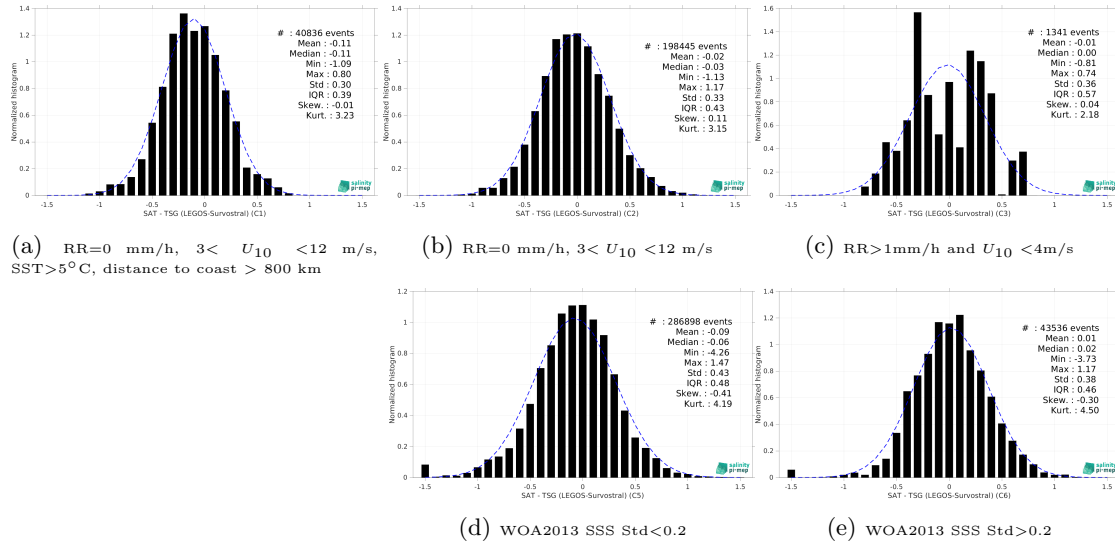
Figure 13: Normalized histogram of \Delta\text{SSS} (SMOS SSS L3 v332 - 9 Days (CATDS-CPDC) - TSG (LEGOS-Survostral)) for 5 different subdatasets corresponding to: RR=0 mm/h, 3 < U_{10} < 12 m/s, SST>5°C, distance to coast > 800 km (a), RR=0 mm/h, 3 < U_{10} < 12 m/s (b), RR>1mm/h and U_{10} < 4 m/s (c), WOA2013 SSS Std<0.2 (d), WOA2013 SSS Std>0.2 (e).
