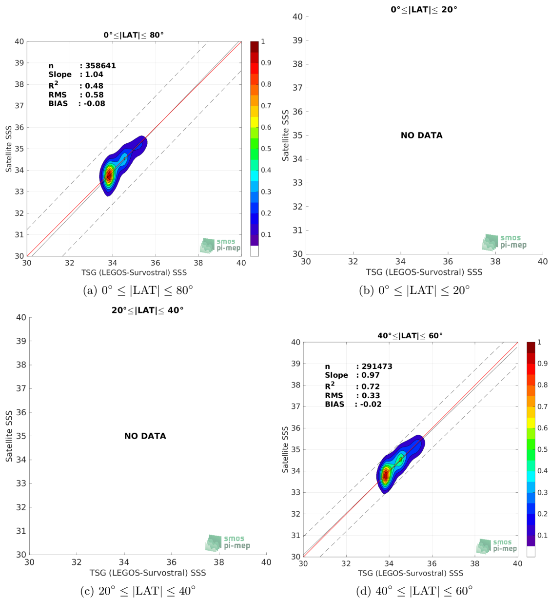
Figure 9: Contour maps of the concentration of SMOS SSS L3 v332 - 9 Days (CATDS-CPDC) SSS (y-axis) versus TSG (LEGOS-Survostral) SSS (x-axis) at match-up pairs for different latitude bands. For each plot, the red line shows x=y . The black thin and dashed lines indicate a linear fit through the data cloud and the \pm 95\% confidence levels, respectively. The number match-up pairs n , the slope and R^2 coefficient of the linear fit, the root mean square (RMS) and the mean bias between satellite and in situ data are indicated for each latitude band in each plots.
