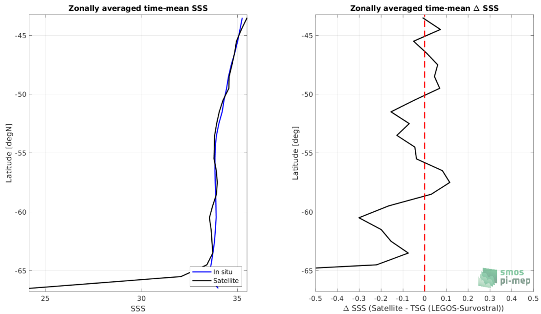
Figure 8: Left panel: Zonal mean SSS from SMOS SSS L3 v332 - 9 Days (CATDS-CPDC) satellite product (black) and from TSG (LEGOS-Survostral) (blue). Right panel: Zonal mean of \Delta SSS (Satellite - TSG (LEGOS-Survostral)) for all the collected Pi-MEP match-up pairs estimated over the full satellite product period.
