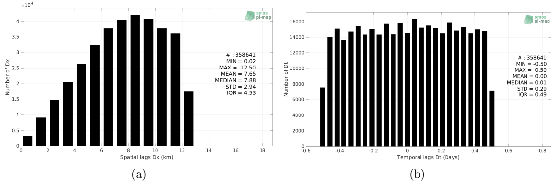
Figure 5: Histograms of the spatial (a) and temporal (b) lags between the location/time of the TSG (LEGOS-Survostral) measurement and the date of the corresponding SMOS SSS L3 v332 - 9 Days (CATDS-CPDC) SSS pixel.
