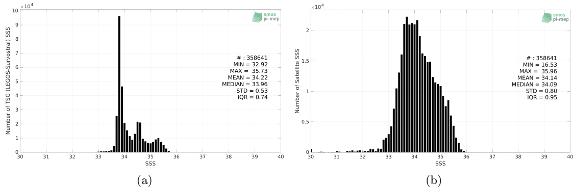
Figure 2: Histograms of SSS from TSG (LEGOS-Survostral) (a) and SMOS SSS L3 v332 - 9 Days (CATDS-CPDC) (b) considering all match-up pairs per bins of 0.1 over the Global Ocean Pi-MEP region and for the full satellite product period.
