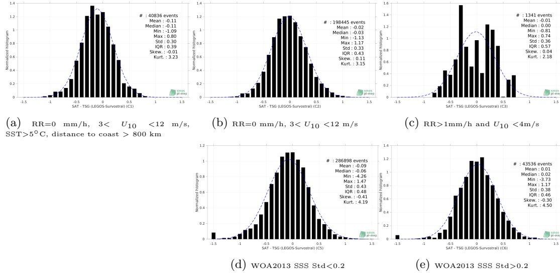
Figure 13: Normalized histogram of \Delta SSS (SMOS SSS L3 v332 - 9 Days (CATDS-CPDC) - TSG (LEGOS-Survostral)) for 5 different subdatasets corresponding to: RR=0 mm/h, 3 < U_{10} < 12 m/s, SST > 5°C, distance to coast > 800 km (a), RR=0 mm/h, 3 < U_{10} < 12 m/s (b), RR > 1mm/h and U_{10} < 4 m/s (c), WOA2013 SSS Std < 0.2 (d), WOA2013 SSS Std > 0.2 (e).
