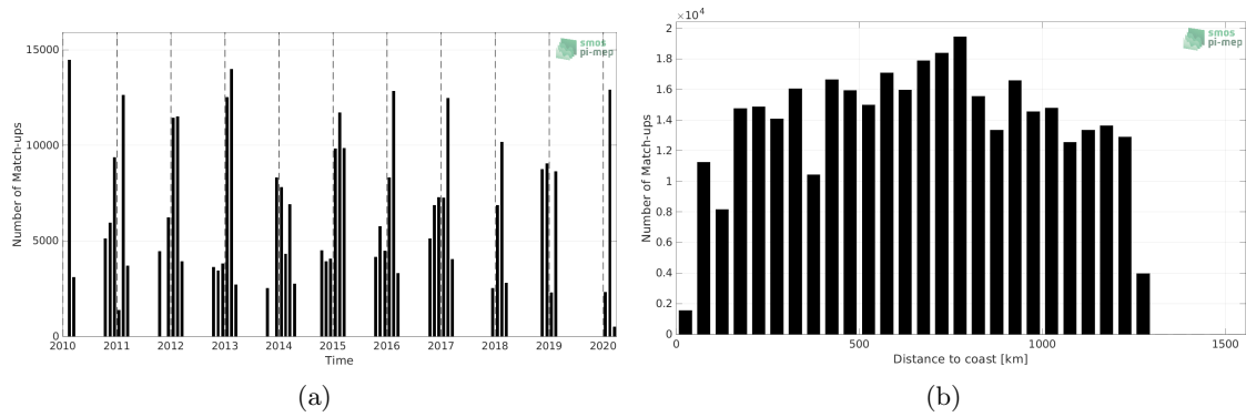
Figure 1: Number of match-ups between TSG (LEGOS-Survostral) and SMOS SSS L3 v332 - 9 Days (CATDS-CPDC) SSS as a function of time (a) and as function of the distance to coast (b) over the Global Ocean Pi-MEP region and for the full satellite product period.
