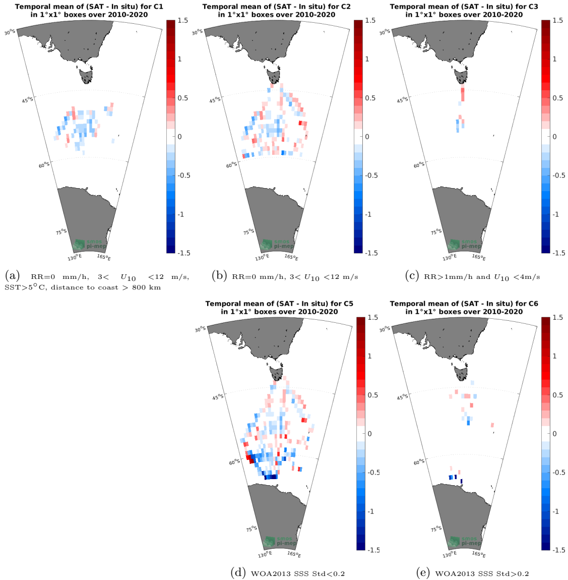
Figure 12: Temporal mean gridded over spatial boxes of size 1^\circ \times 1^\circ of \Delta SSS (SMOS SSS L3 v332 - 9 Days (CATDS-CPDC) - TSG (LEGOS-Survostral)) for 5 different subdatasets corresponding to: RR=0 mm/h, 3 < U_{10} < 12 m/s, SST>5°C, distance to coast > 800 km (a), RR=0 mm/h, 3 < U_{10} < 12 m/s (b), RR>1mm/h and U_{10} < 4 m/s (c), WOA2013 SSS Std<0.2 (d), WOA2013 SSS Std>0.2 (e).
