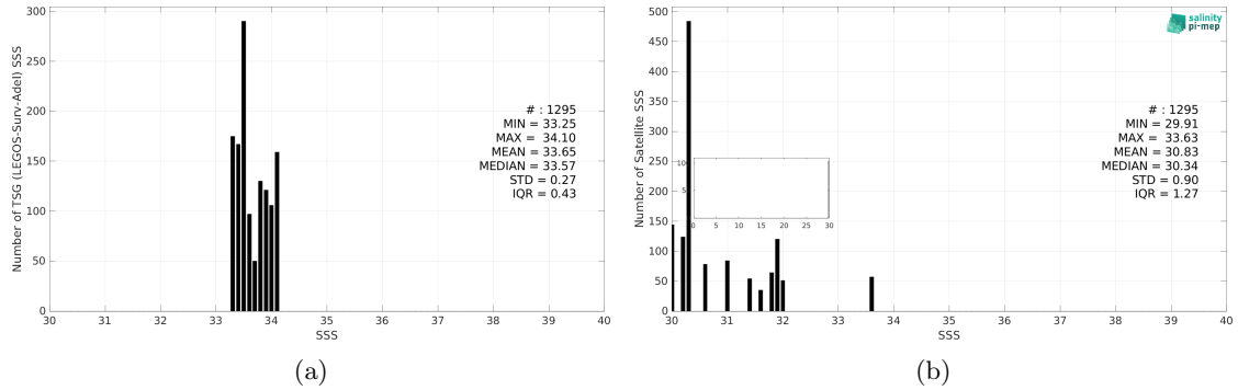
Figure 3: Histograms of SSS from TSG (LEGOS-Surv-Adel) (a) and SMOS SSS L3 v332 - 9 Days (CATDS-CPDC) (b) considering all match-up pairs per bins of 0.1 over the Global Ocean Pi-MEP region and for the full satellite product period.
