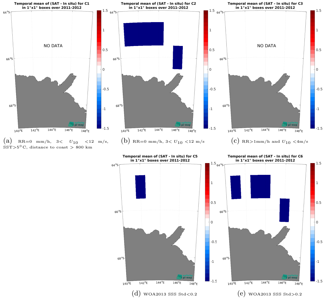
Figure 14: Temporal mean gridded over spatial boxes of size 1^\circ \times 1^\circ of \Delta SSS (SMOS SSS L3 v332 - 9 Days (CATDS-CPDC) - TSG (LEGOS-Surv-Adel)) for 5 different subdatasets corresponding to: RR=0 mm/h, 3 < U_{10} < 12 m/s, SST>5°C, distance to coast > 800 km (a), RR=0 mm/h, 3 < U_{10} < 12 m/s (b), RR>1mm/h and U_{10} < 4 m/s (c), WOA2013 SSS Std<0.2 (d), WOA2013 SSS Std>0.2 (e).
