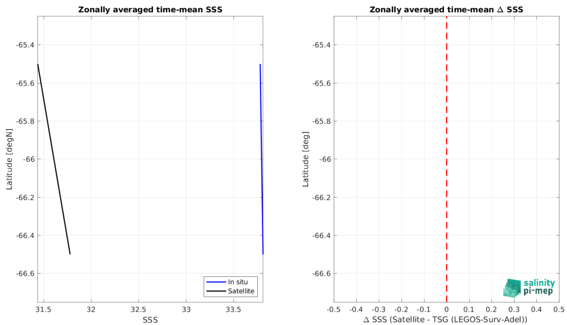
Figure 9: Left panel: Zonal mean SSS from SMOS SSS L3 v332 - 9 Days (CATDS-CPDC) satellite product (black) and from TSG (LEGOS-Surv-Adel) (blue). Right panel: Zonal mean of \Delta SSS (Satellite - TSG (LEGOS-Surv-Adel)) for all the collected Pi-MEP match-up pairs estimated over the full satellite product period.
