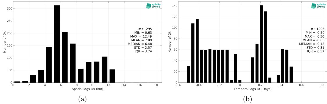
Figure 6: Histograms of the spatial (a) and temporal (b) lags between the location/time of the TSG (LEGOS-Surv-Adel) measurement and the date of the corresponding SMOS SSS L3 v332 - 9 Days (CATDS-CPDC) SSS pixel.
