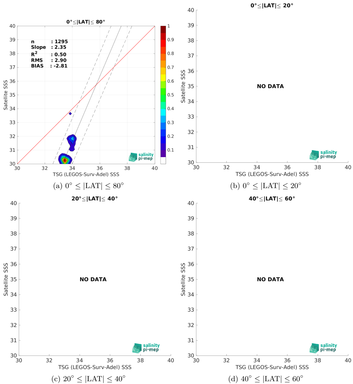
Figure 10: Contour maps of the concentration of SMOS SSS L3 v332 - 9 Days (CATDS-CPDC) SSS (y-axis) versus TSG (LEGOS-Surv-Adel) SSS (x-axis) at match-up pairs for different latitude bands. For each plot, the red line shows x=y . The black thin and dashed lines indicate a linear fit through the data cloud and the \pm 95\% confidence levels, respectively. The number match-up pairs n , the slope and R^2 coefficient of the linear fit, the root mean square (RMS) and the mean bias between satellite and in situ data are indicated for each latitude band in each plots.
