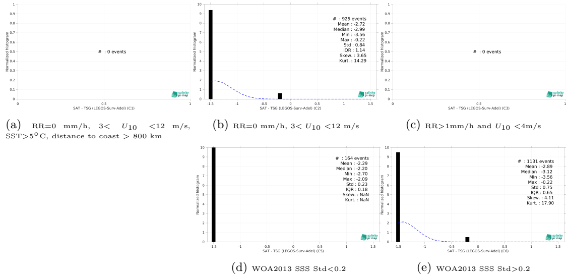
Figure 15: Normalized histogram of \Delta SSS (SMOS SSS L3 v332 - 9 Days (CATDS-CPDC) - TSG (LEGOS-Surv-Adel)) for 5 different subdatasets corresponding to: RR=0 mm/h, 3 < U_{10} < 12 m/s, SST > 5°C, distance to coast > 800 km (a), RR=0 mm/h, 3 < U_{10} < 12 m/s (b), RR > 1mm/h and U_{10} < 4 m/s (c), WOA2013 SSS Std < 0.2 (d), WOA2013 SSS Std > 0.2 (e).
