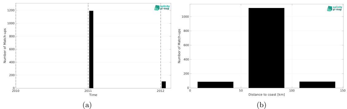
Figure 2: Number of match-ups between TSG (LEGOS-Surv-Adel) and SMOS SSS L3 v332 - 9 Days (CATDS-CPDC) SSS as a function of time (a) and as function of the distance to coast (b) over the Global Ocean Pi-MEP region and for the full satellite product period.
