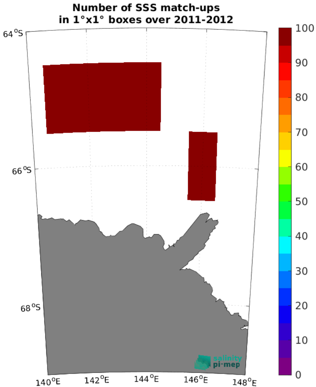
Figure 5: Number of SSS match-ups between TSG (LEGOS-Surv-Adel) SSS and the SMOS SSS L3 v332 - 9 Days (CATDS-CPDC) SSS product for the Global Ocean Pi-MEP region over 1°x1° boxes and for the full satellite product period.
