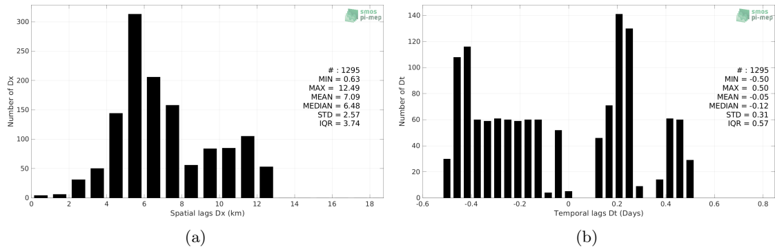
Figure 5: Histograms of the spatial (a) and temporal (b) lags between the location/time of the TSG (LEGOS-Surv-Adel) measurement and the date of the corresponding SMOS SSS L3 v332 - 9 Days (CATDS-CPDC) SSS pixel.
