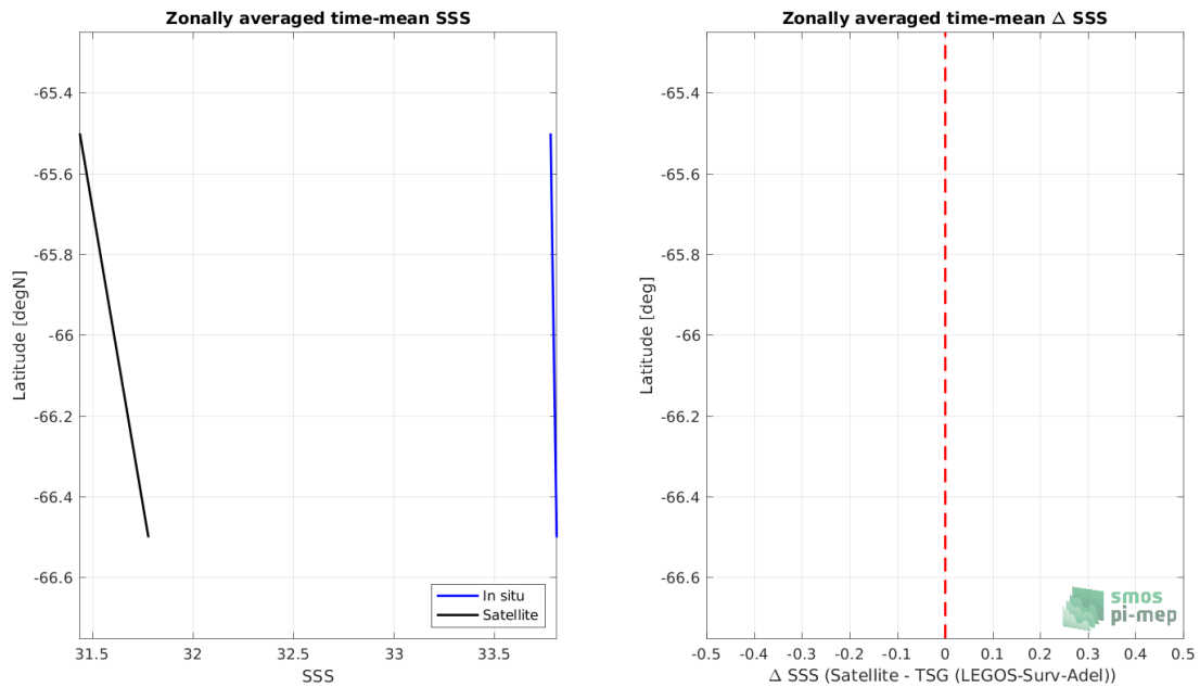
Figure 8: Left panel: Zonal mean SSS from SMOS SSS L3 v332 - 9 Days (CATDS-CPDC) satellite product (black) and from TSG (LEGOS-Surv-Adel) (blue). Right panel: Zonal mean of \Delta SSS (Satellite - TSG (LEGOS-Surv-Adel)) for all the collected Pi-MEP match-up pairs estimated over the full satellite product period.
