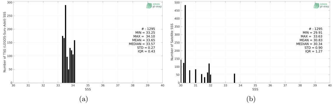
Figure 2: Histograms of SSS from TSG (LEGOS-Surv-Adel) (a) and SMOS SSS L3 v332 - 9 Days (CATDS-CPDC) (b) considering all match-up pairs per bins of 0.1 over the Global Ocean Pi-MEP region and for the full satellite product period.
