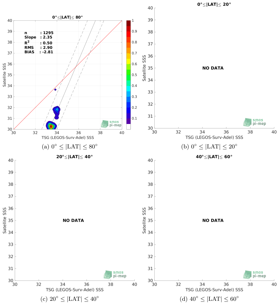
Figure 9: Contour maps of the concentration of SMOS SSS L3 v332 - 9 Days (CATDS-CPDC) SSS (y-axis) versus TSG (LEGOS-Surv-Adel) SSS (x-axis) at match-up pairs for different latitude bands. For each plot, the red line shows x=y . The black thin and dashed lines indicate a linear fit through the data cloud and the \pm 95\% confidence levels, respectively. The number match-up pairs n , the slope and R^2 coefficient of the linear fit, the root mean square (RMS) and the mean bias between satellite and in situ data are indicated for each latitude band in each plots.
