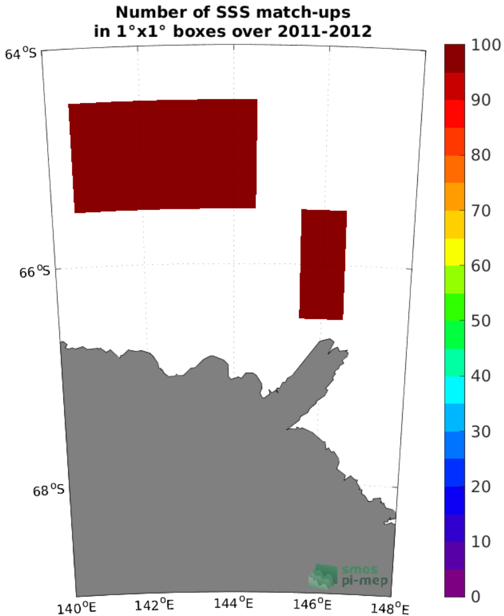
Figure 4: Number of SSS match-ups between TSG (LEGOS-Surv-Adel) SSS and the SMOS SSS L3 v332 - 9 Days (CATDS-CPDC) SSS product for the Global Ocean Pi-MEP region over 1°x1° boxes and for the full satellite product period.
