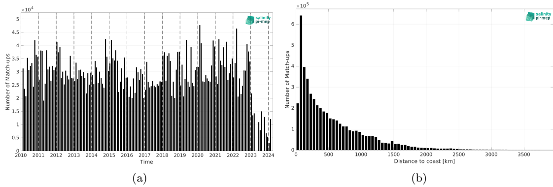
Figure 2: Number of match-ups between TSG (LEGOS-DM) and SMOS SSS L3 v332 - 9 Days (CATDS-CPDC) SSS as a function of time (a) and as function of the distance to coast (b) over the Global Ocean Pi-MEP region and for the full satellite product period.
