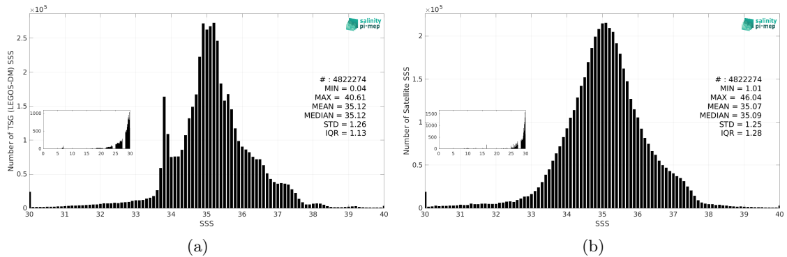
Figure 3: Histograms of SSS from TSG (LEGOS-DM) (a) and SMOS SSS L3 v332 - 9 Days (CATDS-CPDC) (b) considering all match-up pairs per bins of 0.1 over the Global Ocean Pi-MEP region and for the full satellite product period.
