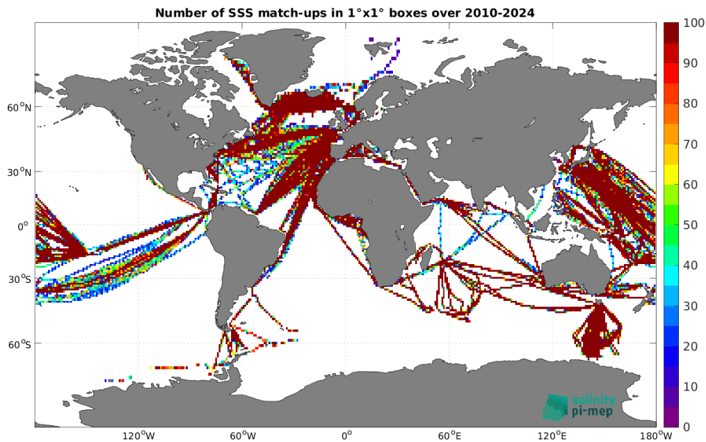
Figure 5: Number of SSS match-ups between TSG (LEGOS-DM) SSS and the SMOS SSS L3 v332 - 9 Days (CATDS-CPDC) SSS product for the Global Ocean Pi-MEP region over 1^\circ \times 1^\circ boxes and for the full satellite product period.
