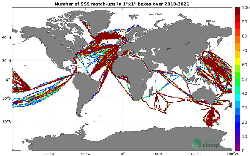
Figure 4: Number of SSS match-ups between TSG (LEGOS-DM) SSS and the SMOS SSS L3 v332 - 9 Days (CATDS-CPDC) SSS product for the Global Ocean Pi-MEP region over 1^\circ \times 1^\circ boxes and for the full satellite product period.
