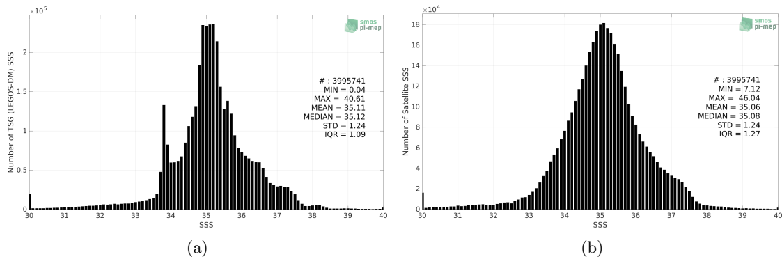
Figure 2: Histograms of SSS from TSG (LEGOS-DM) (a) and SMOS SSS L3 v332 - 9 Days (CATDS-CPDC) (b) considering all match-up pairs per bins of 0.1 over the Global Ocean Pi-MEP region and for the full satellite product period.
