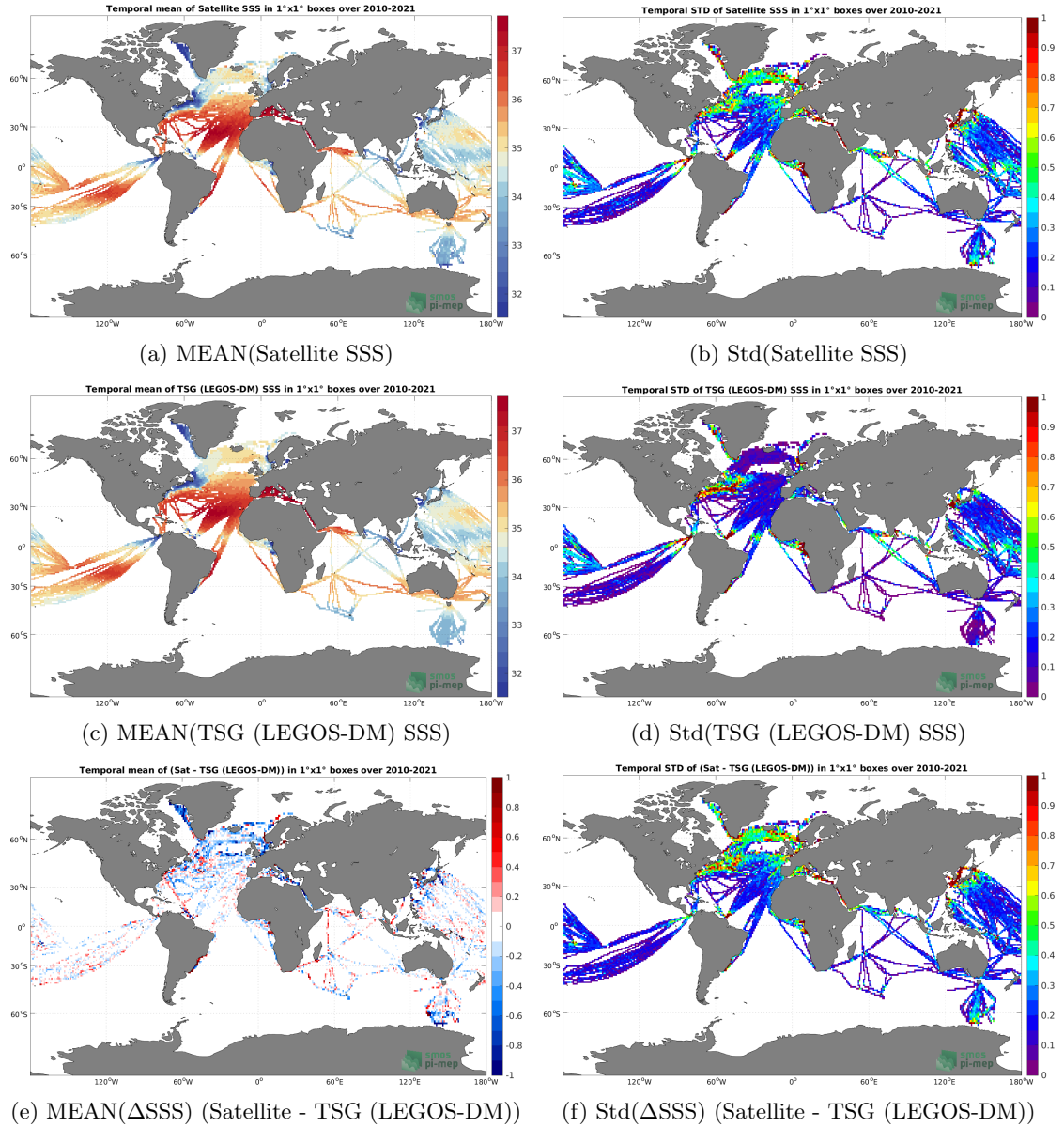
Figure 6: Temporal mean (left) and Std (right) of SSS from SMOS SSS L3 v332 - 9 Days (CATDS-CPDC) (top), TSG (LEGOS-DM) (middle), and of \Delta SSS (Satellite - TSG (LEGOS-DM)). Only match-up pairs are used to generate these maps.
