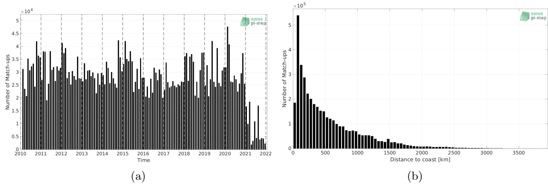
Figure 1: Number of match-ups between TSG (LEGOS-DM) and SMOS SSS L3 v332 - 9 Days (CATDS-CPDC) SSS as a function of time (a) and as function of the distance to coast (b) over the Global Ocean Pi-MEP region and for the full satellite product period.
